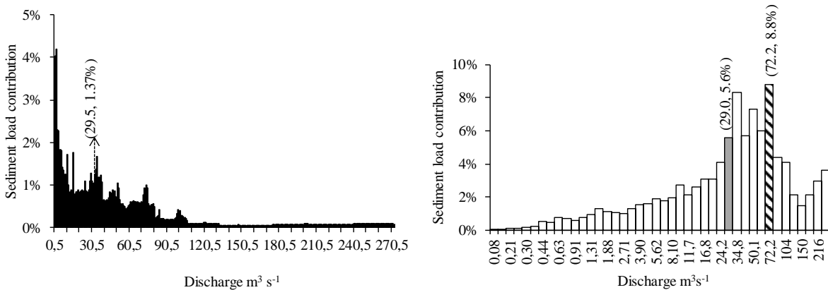
10 Figure 11: Sediment load histogram established using the sediment rating curve: for a subdivision into classes of equal amplitudes 1 \text{ m}^3 \text{ s}^{-1} (left) and with a geometric progression of common ratio 1.2 (right).
