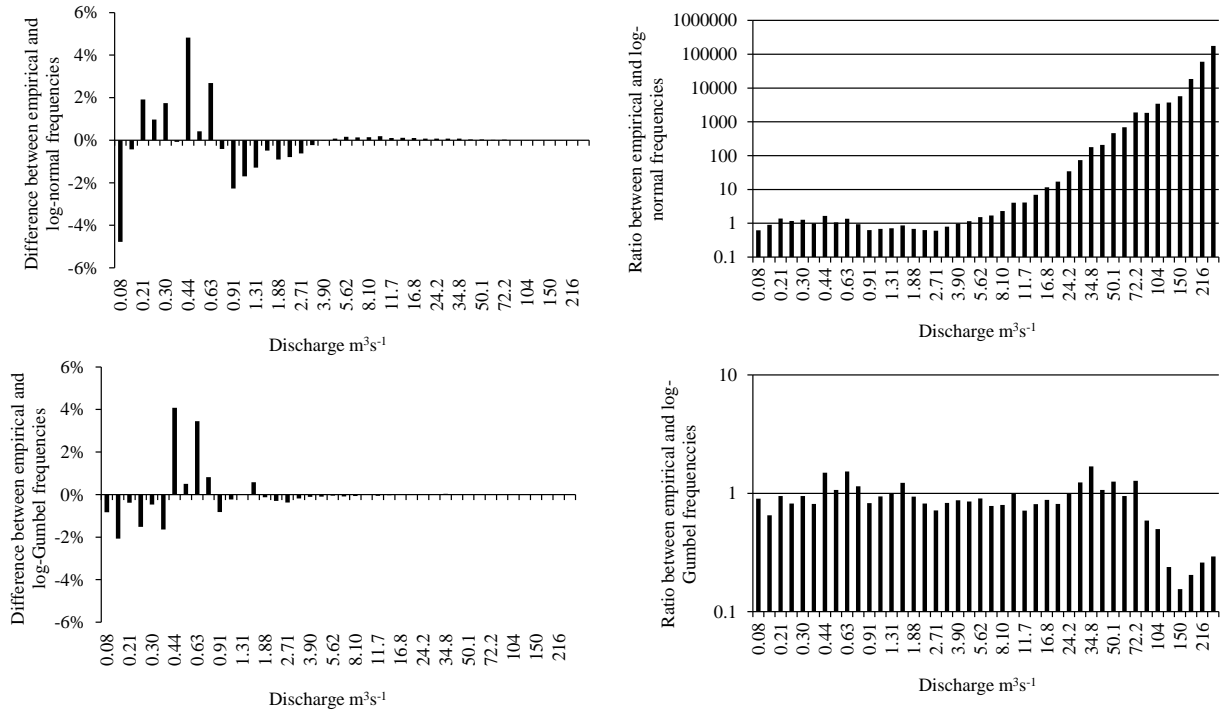
10 Figure 12: Analysis of errors (difference and ratio) between observed and theoretical frequencies of water discharge: for the log-normal distribution (above) and for the log-Gumbel distribution (below).
