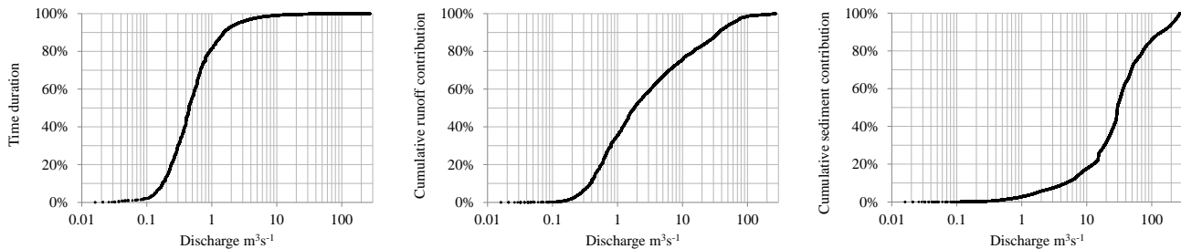
20 Figure 3: Cumulative frequency, water and sediment inputs assigned to ordinal discharges in the Wadi Sebdou (1973-2004).
