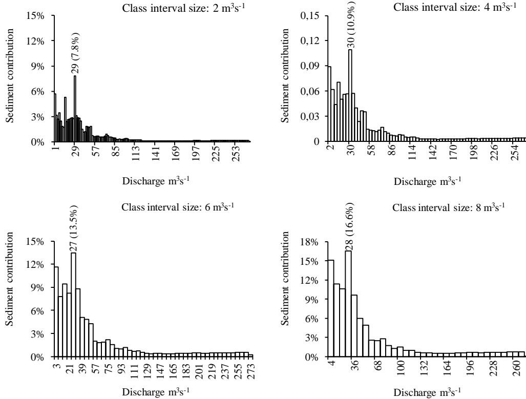
Figure 5: Sediment yields for subdivisions of equal lengths: 2, 4, 6 and 8 \text{ m}^3 \text{ s}^{-1} .
