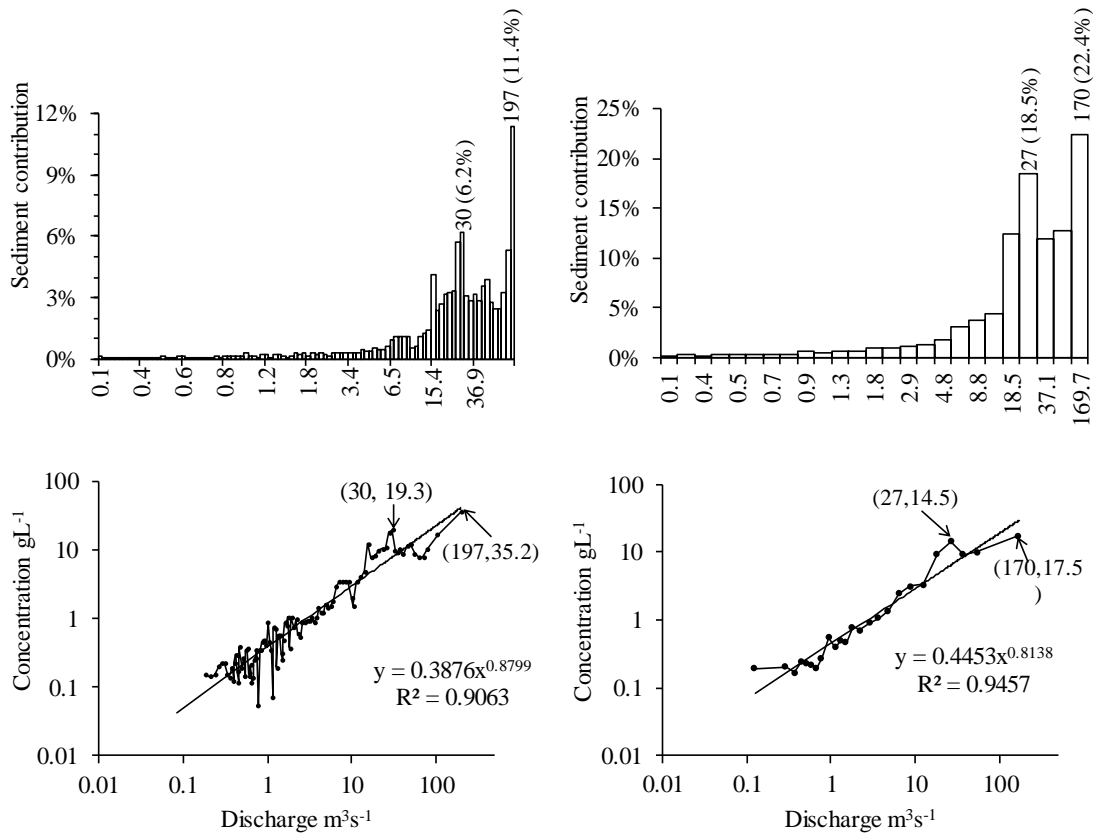
5 Figure 6: Sediment supply per class, and sediment rating curves, for a subdivision into classes of equal water supplies of 1% (left) and 4% (right).
