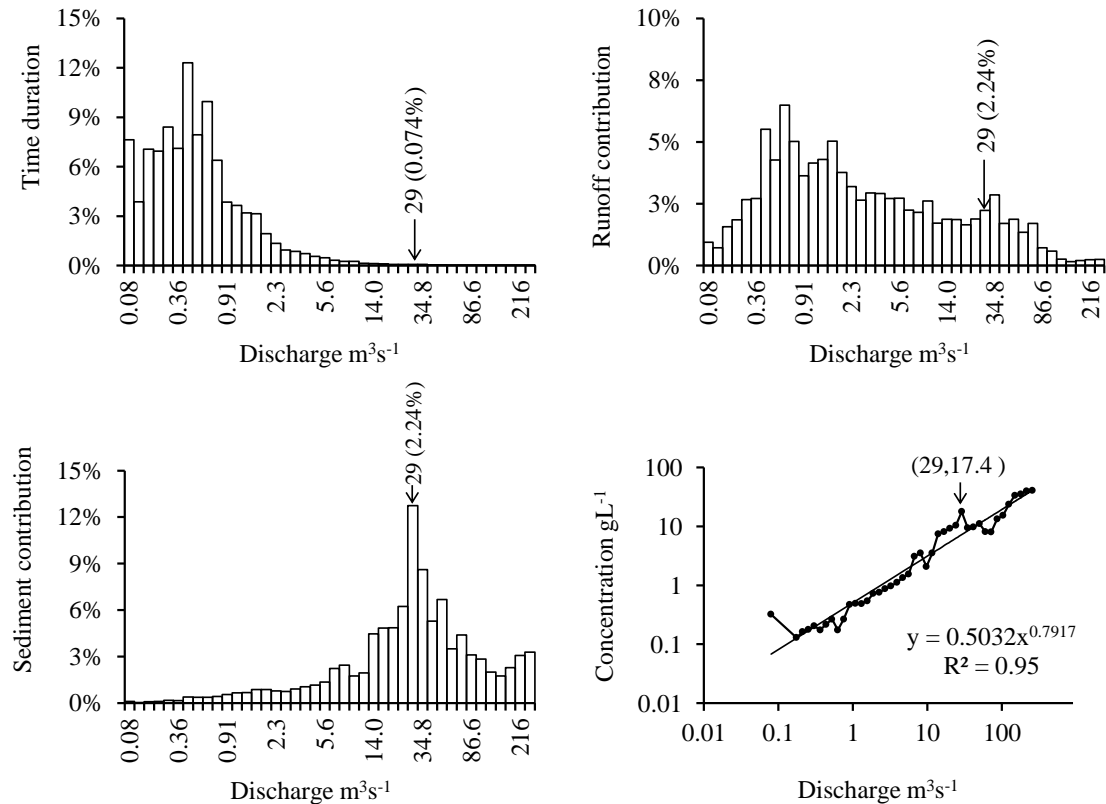
Figure 7: Duration, water and sediment input per class, and sediment rating curves, for the subdivision into classes of geometric progression of common ratio 1.2
