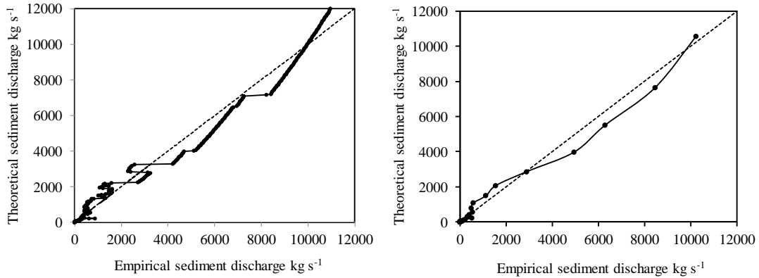
5 Figure 10: Comparison between the analytical sediment supply by class given from the rating curve ( Q_s^k = a Q^{(b+1)} , in ordinate) and the elementary contributions Q_{S,obs} = 10^6 \frac{\Delta Y^k}{\Delta T^k} where \Delta Y^k (unit: 10^3 tonnes) and \Delta T^k (unit: s) are obtained from Eq. 3 (in abscissa): for a subdivision into classes of equal amplitudes 1 \text{ m}^3 \text{ s}^{-1} (left) and with a geometric progression of common ratio 1.2 (right).
