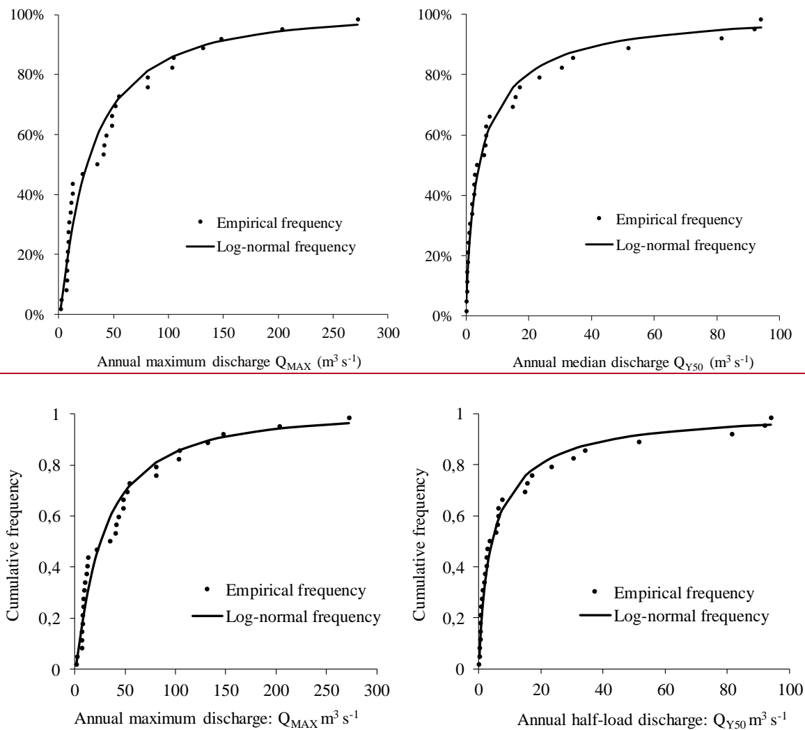
Figure 8: Adjustment to the log-normal distribution of maximum annual discharges, Q_{MAX} , and median annual discharges in terms of sediment yield , Q_{Y50} .
