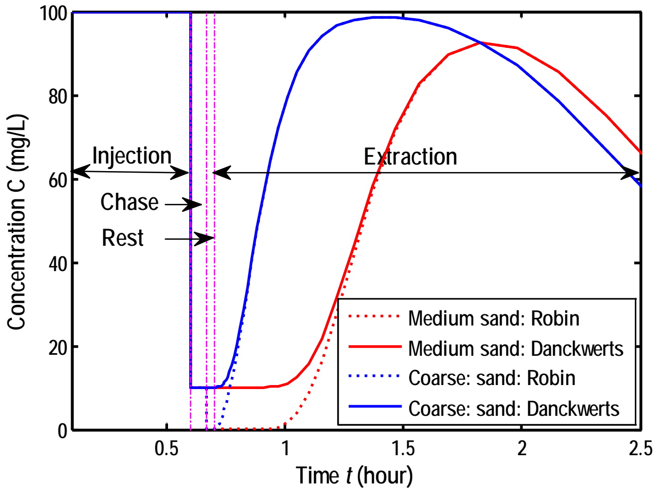
A Figure 4. Comparison of BTCs in the wellbore between the Robin and Danckwerts conditions: A. C_0^{cha} = 10.0 mg/L, B.
