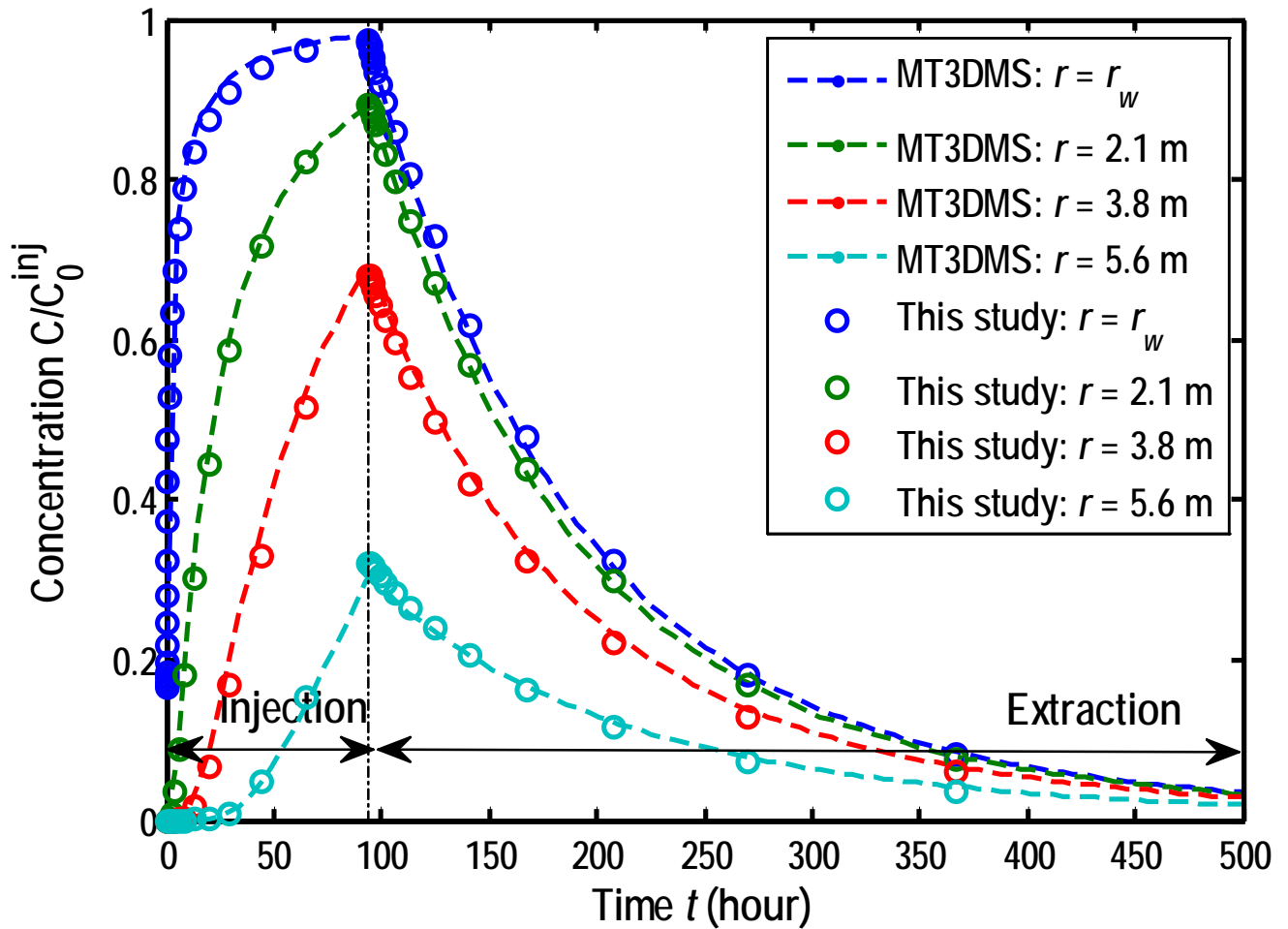
Figure 3. Comparison of BTCs between the solutions of MODFLOW/MT3DMS and of this study.
