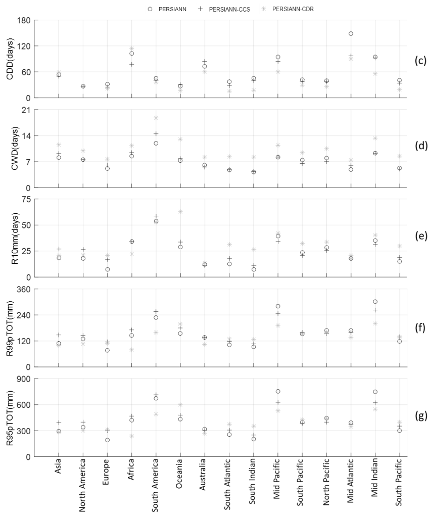
Figure 199: Mean annual precipitation and Extreme Indices (SDII, CDD, CWD, R10mm, R99pTOT, and R95pTOT) over continents and oceans for PERSIANN, PERSIANN-CCS, and PERSIANN-CDR.
