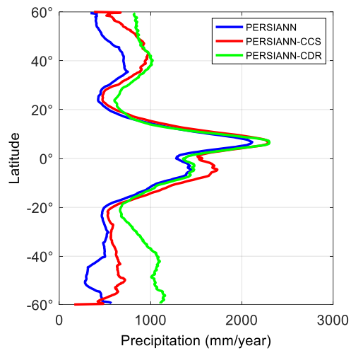
Figure_87: Mean annual zonal precipitation (mm/year) for PERSIANN, PERSIANN-CCS, and PERSIANN-CDR.
