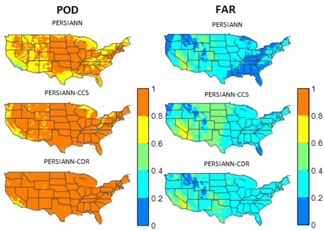
Figure 43: Probability of Detection (POD) and False Alarm Ratio (FAR) of PERSIANN, PERSIANN-CCS, and PERSIANN-CDR against CPC for the period (2003-2015) over the CONUS.
