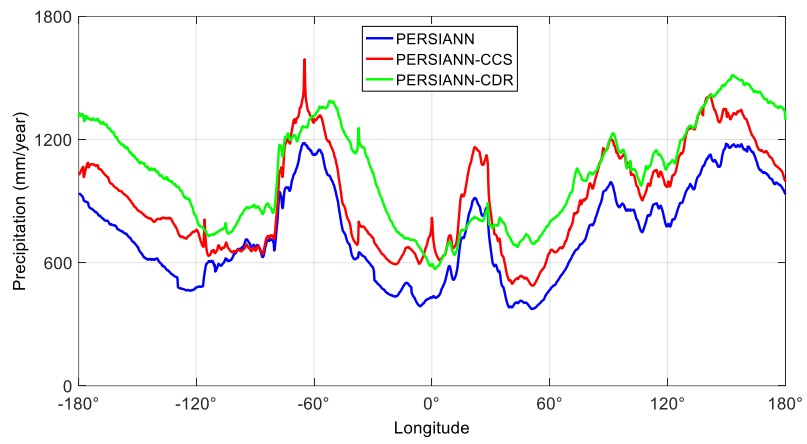
Figure_98: Mean annual meridional precipitation (mm/year) for PERSIANN, PERSIANN-CCS, and PERSIANN-CDR.
