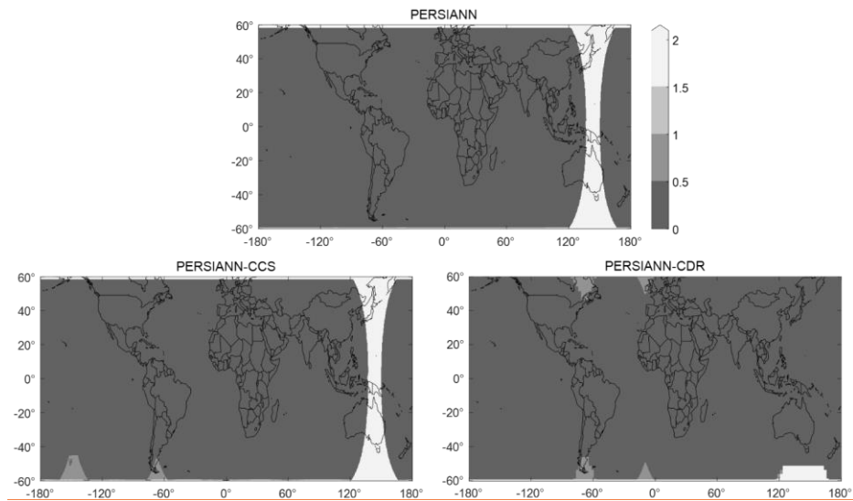
Figure 1: Percentage of missing data over the period (2003-2015) for PERSIANN, PERSIANN-CCS and PERSIANN-CDR.
