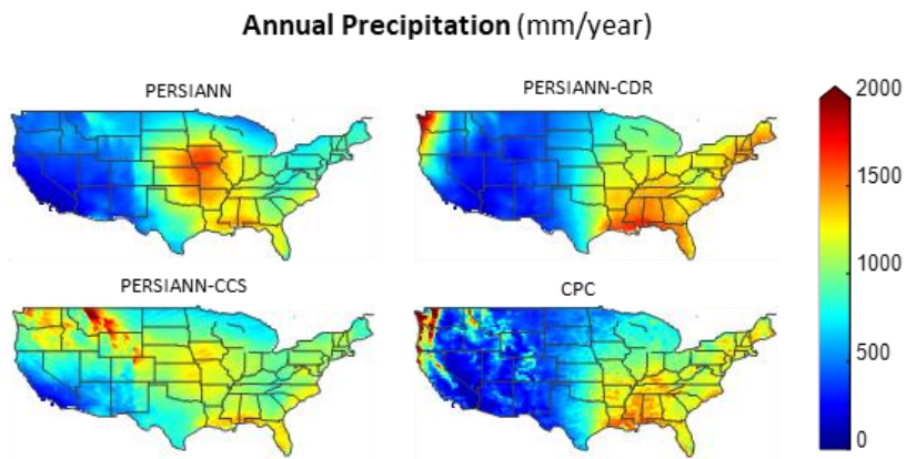
Figure 21: Average annual precipitation (mm/year) for the period (2003-2015) over the CONUS.
