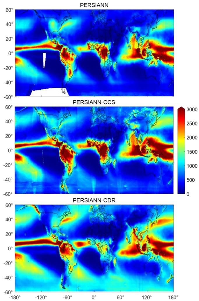
Figure_76: Mean annual precipitation (mm) for PERSIANN, PERSIANN-CCS, and PERSIANN-CDR.
