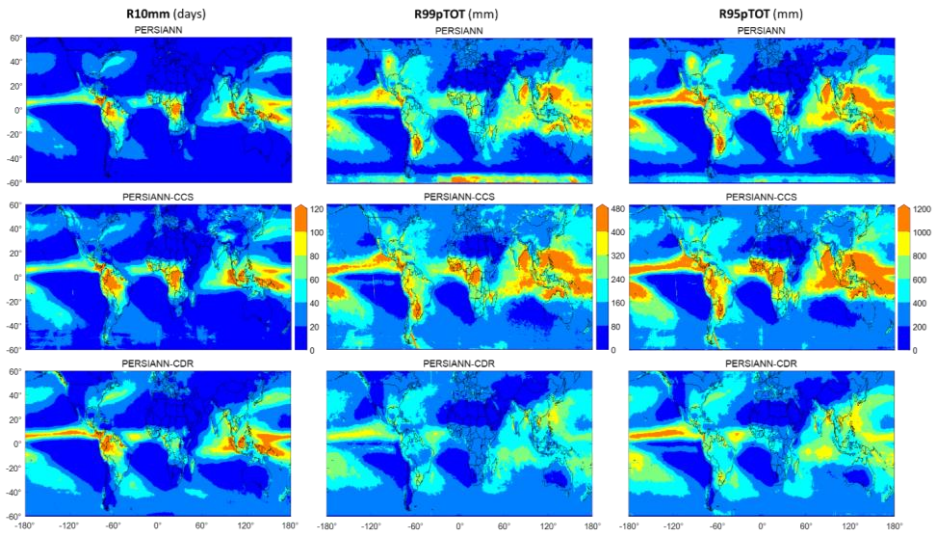
Figure 1211: Extreme Precipitation Indices (R10mm, R99pTOT, and R95pTOT) for PERSIANN, PERSIANN-CCS, and PERSIANN-CDR over the globe. (See Table 4 for definition of the indices).
