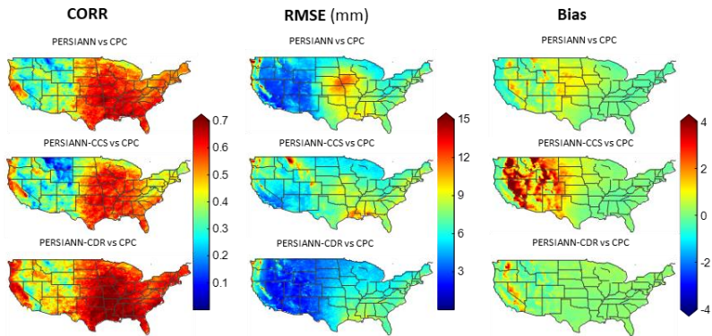
20 Figure 23: Correlation (CORR), Root Mean Square Error (RMSE) and multiplicative Bias of PERSIANN, PERSIANN-CCS, and PERSIANN-CDR against CPC for the period (2003-2015) over the CONUS.
