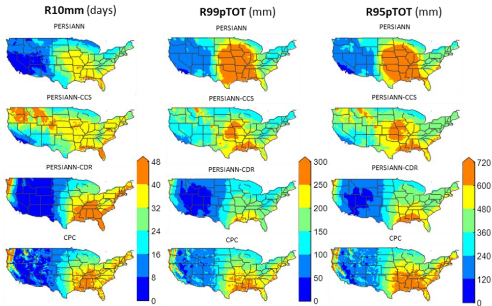
Figure 65: Extreme Precipitation Indices (R10mm, R99pTOT and R95pTOT) for PERSIANN, PERSIANN-CCS, and PERSIANN-CDR over the CONUS (See Table 4 for definition of the indices).
