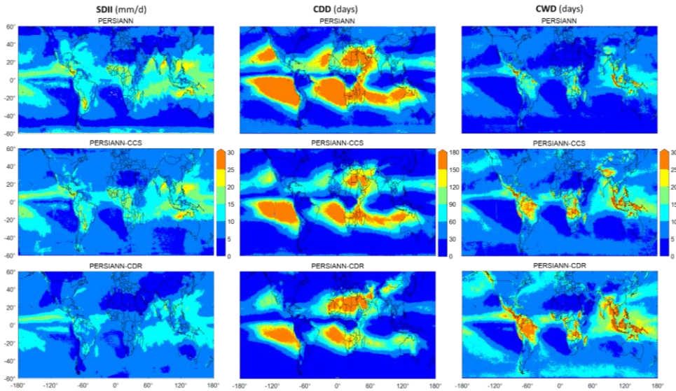
5 Figure 1410: Extreme Precipitation Indices (SDII, CDD, and CWD) for PERSIANN, PERSIANN-CCS, and PERSIANN-CDR over the globe. (See Table 4 for definition of the indices).
