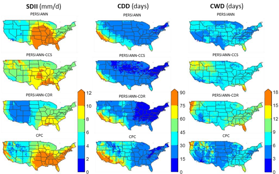
5 | Figure 54: Extreme Precipitation Indices (SDII, CDD and CWD) for PERSIANN, PERSIANN-CCS 2 and PERSIANN-CDR over the CONUS (See Table 4 for definition of the indices).
