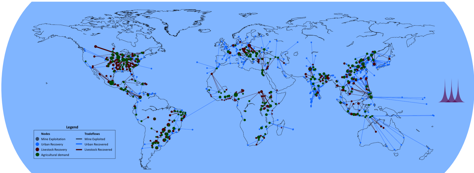
Figure 6. Phosphorus trade network for trade in recycled P only (scenario 3) at determined phosphorus market prices of 5,700 [ \$ t^{-1} ] with 7.92 [Mt] being traded. All of this trade is sustainable but is only able to accommodate 41% of demand.
