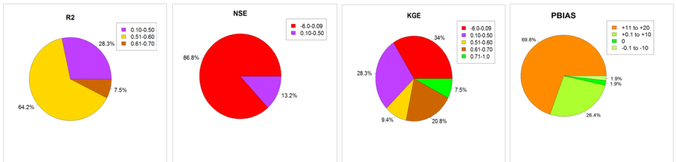
Figure 7. Performance metrics (NSE, KGE, R^2 , and PBIAS) result of SWAT (SWAT_P-M) when validated MOD16 (MS6)
