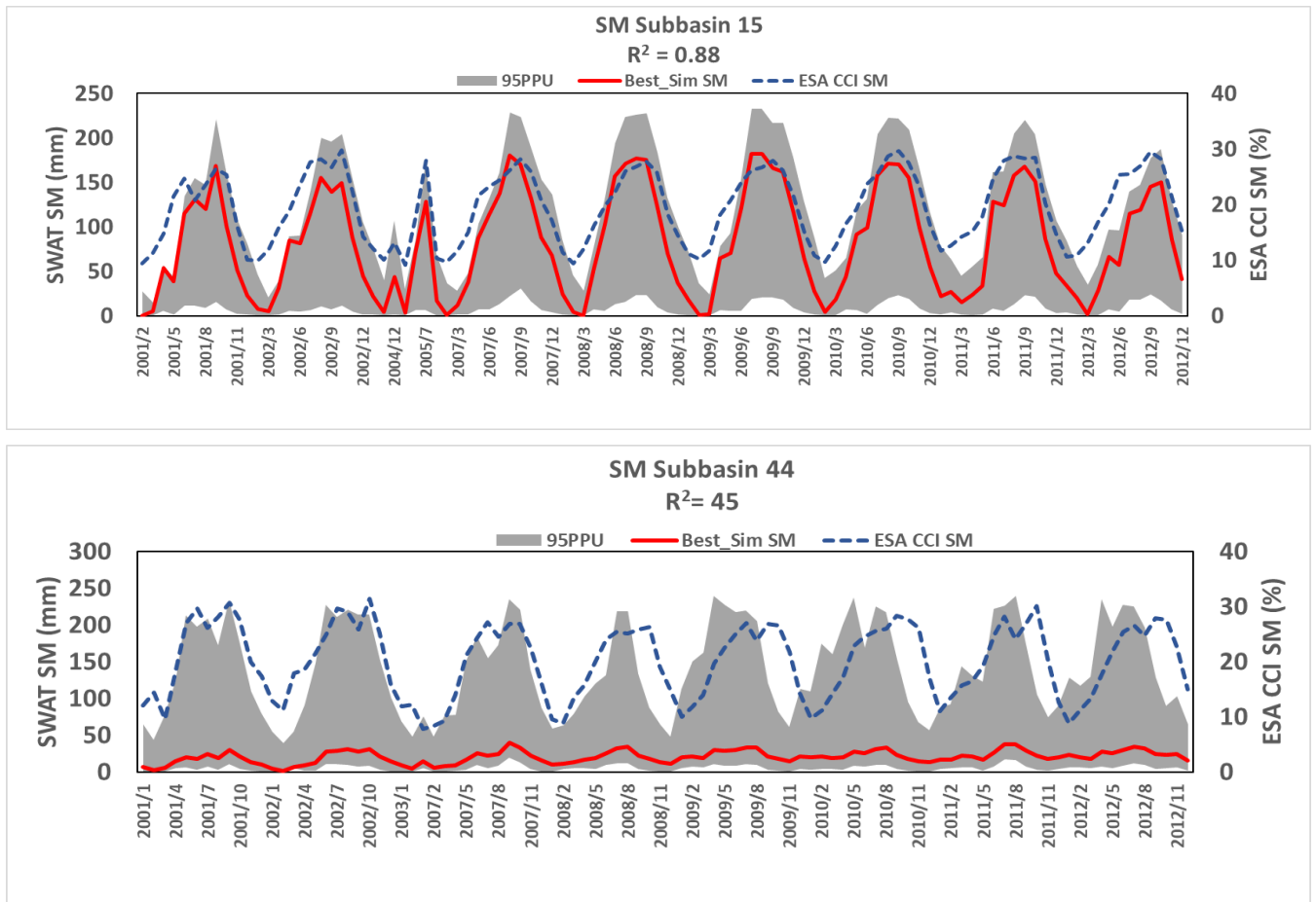
Figure 13. Performance metric ( R^2 ) of SWAT simulated soil moisture when validated with ESA CCI soil moisture v3.2
