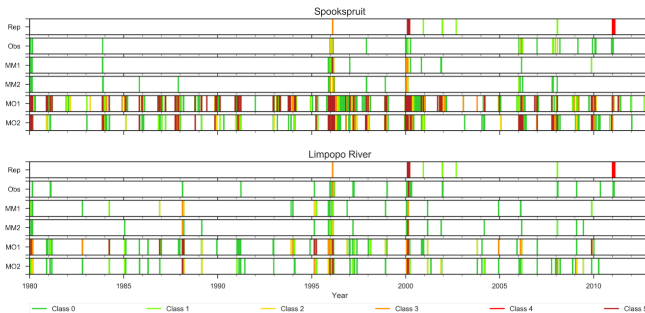
Figure 3: Occurrence of flood events of increasing severity classes at the Spookspruit gauge (252 km 2 ; upper panel) and in the main Limpopo River (98,240 km 2 ; lower panel). Model flood events were identified using model climatology (MM1 & MM2) or observed climatology (MO1 & MO2), and were compared to benchmarks based on a compiled disaster impact database (Rep) and observed river discharge data (Obs). The index value refer to models with 0.5 degree resolution (1) and 0.25 degree resolution (2). Results are shown for the WaterGAP3 model, which is available in the earth2Observe Water Resources Re-analysis dataset.
