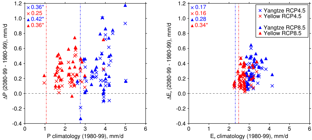
Figure 9. Future-minus-present changes (2080–2099 minus 1980–1999) in P (left) and E_p (right) against P and E_p climatologies (1980–1999), respectively, for 34 CMIP5 models. The dashed vertical lines show the observed climatologies for the Yellow (red) and Yangtze (blue) catchments. The values in the top left of each panel refer to correlation coefficients for the catchment and RCP emissions scenario listed in the legend. Those with asterisks are significant at the 95 % ( p = 0.05 ) confidence level.
