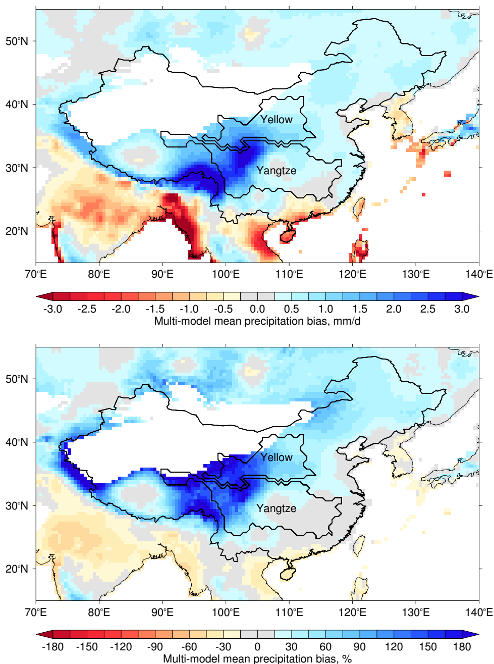
Figure 6. Absolute (top) and relative (bottom) multi-model mean precipitation climatology bias for 1961–1990. The location of the Yangtze and Yellow catchments within China is shown. Desert regions ( <200 \text{ mm year}^{-1} ), as determined from CRU climatology (1961–1990), are masked in white.
