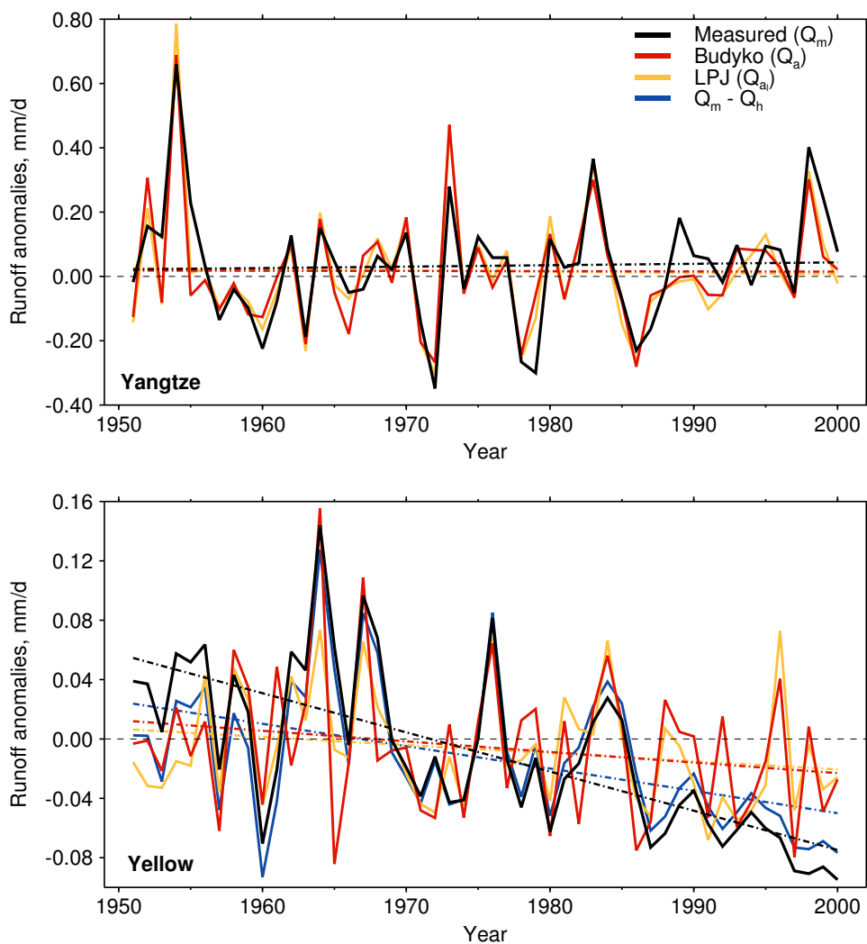
Figure 5. Runoff anomalies for the Yangtze (top) and Yellow (bottom) river catchments for 1951–2000, relative to 1961–1990. Shown are measured runoff ( Q_m ), runoff due to aridity change ( Q_a ), runoff simulated by the LPJ LSM ( Q_{ai} ) and (for the Yellow river only) the difference between Q_m and runoff due to direct human impacts ( Q_h ). The dashed lines show linear fits to the time series.
