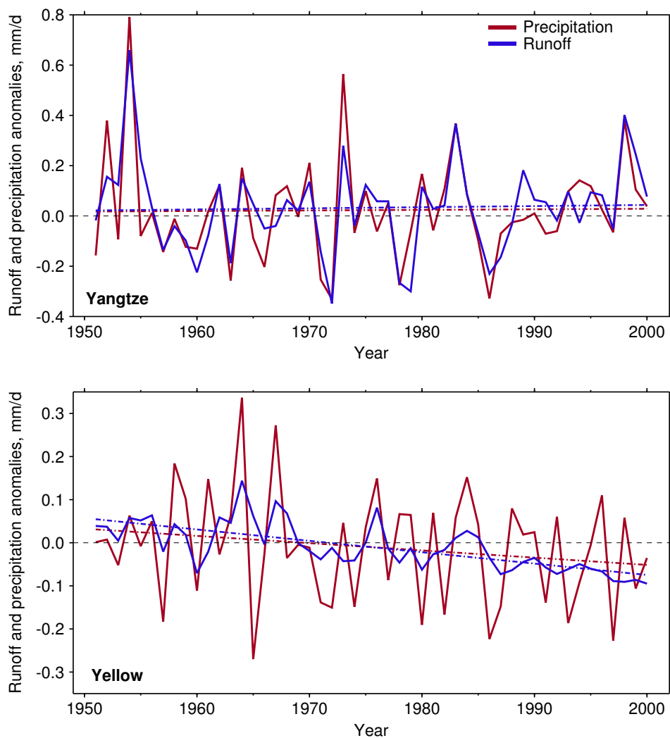
Figure 3. Observed runoff and precipitation anomalies for the Yangtze (top) and Yellow (bottom) river catchments for 1951–2000, relative to 1961–1990. The dot-dashed lines show linear fits to the time series.
