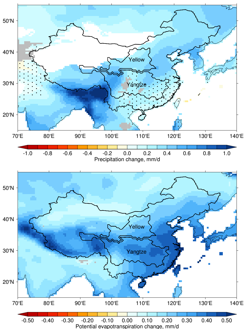
Figure 8. Multi-model mean future-minus-present changes (2080–2099 minus 1980–1999) in P (top) and E_p (bottom) in RCP8.5. Stippling indicates where less than 50 % of the CMIP5 models show significant change, as determined with a t -test comparing present-day and future climates. Absence of stippling indicates where more than 50 % of the models show significant change and more than 80 % of the significant models agree on the sign. Gray indicates where more than 50 % of the models show significant change but less than 80 % of the significant models agree on the sign. This method follows (Tebaldi et al., 2011). Desert regions ( <200 \text{ mm year}^{-1} ), as determined from CRU climatology (1961–1990), are masked in white for P .
