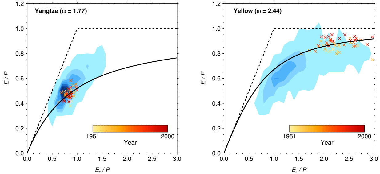
Figure 7. The evaporative index against aridity for the Yangtze (left) and Yellow (right) river catchments. The shaded blue regions represent the density of CMIP5 annual mean data for the 1951–2000 period, with darker shades meaning more data in a given region of the Budyko space. The symbols represent observed data with darker shades for the more recent years. \omega values are calculated for the 1951–2000 period using Eq. (5).
