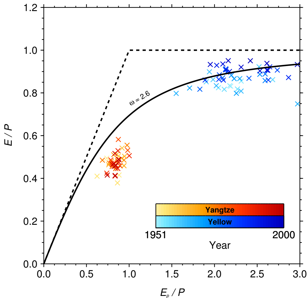
Figure 4. The evaporative index against aridity for the Yangtze (red) and Yellow (blue) river catchments. The symbols represent observed annual mean data for 1951–2000 with darker shades for the more recent years. The traditional Budyko curve is fitted, corresponding to \omega = 2.6 in Eq. (3).
