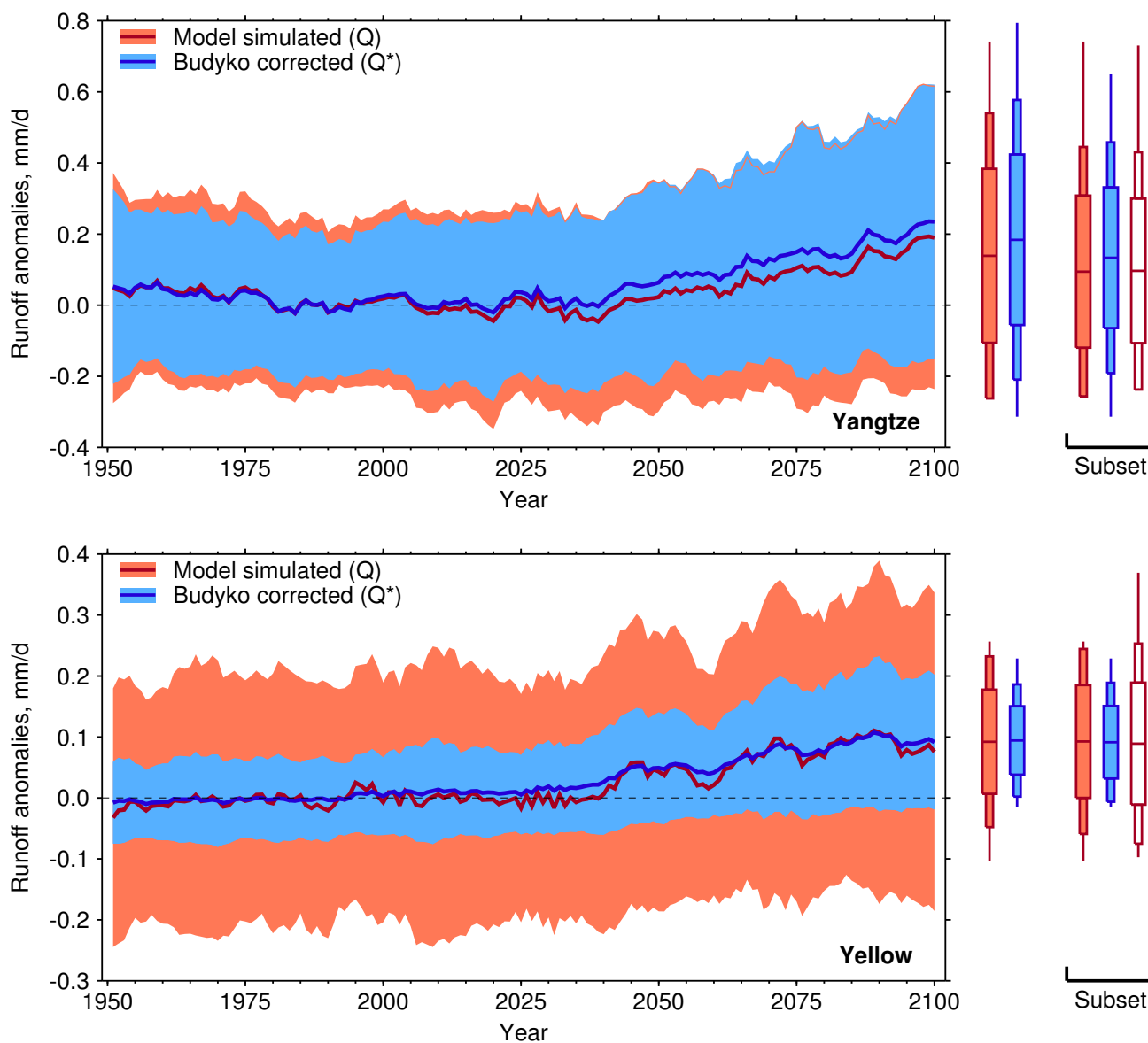
Figure 10. CMIP5 model simulated ( Q ; orange) and CMIP5 Budyko corrected ( Q^* ; blue) runoff anomalies for 1951–2100, relative to 1980–1999, for the Yangtze (top) and Yellow (bottom) river catchments in the historical and RCP8.5 experiments. Shown are the 5-year running multi-model mean (thick line) and 5–95 % ranges (shading) across the CMIP5 ensemble. The box plots (mean, \pm one standard deviation ranges, 5–95 % ranges, and minimum to maximum ranges) are given for 2080–2099 (Table 1). Also shown, for comparison, are box plots for a subset of 28 (from 34) CMIP5 models for which Q is directly simulated (not limited to being calculated as P - E ). The unfilled box plot shows CMIP5 model directly simulated runoff for 2080–2099.
