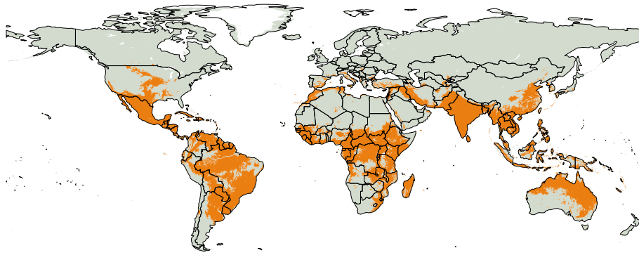
Figure 6. Global map indicating the areas (in orange) prone for infiltration excess surface runoff, defined as those areas where extreme precipitation exceeds the infiltration rate (Fig. S2). See SI for more details.
