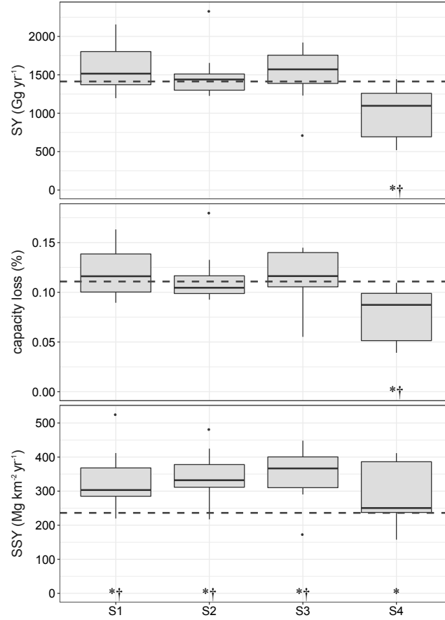
Figure S9. Catchment-average reservoir sediment yield (SY) (Gg yr -1 ), capacity loss (%) and hillslope erosion (SSY) (Mg km -2 yr -1 ). The boxplots indicate the spread of the catchment-average among the nine climate models. In each panel the horizontal dashed line represents the catchment-average value for the reference scenario. An asterisk (*) indicates a robust change and a dagger (†) indicates a significant change (p<0.05). The boxplots are described as follows: the hinges indicate the 25th and 75th percentiles, the thick horizontal line indicates the median, the whiskers indicate 1.5 times the inter quantile range from each of the two hinges and the dots indicate outliers.
