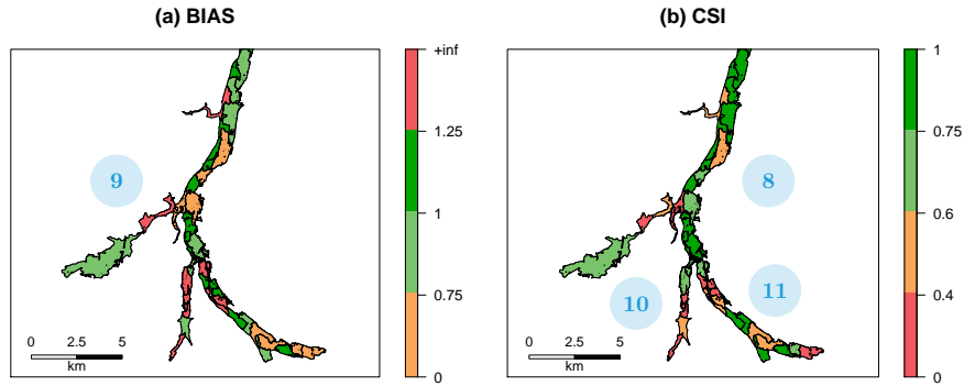
Figure 14. Reach-scale performance (a) BIAS and (b) CSI for the physical combination of parameters : Kch = 10 and Kfp = 5m^{1/3} \cdot s^{-1} , for the upstream part of the catchment. Criteria values have been categorised as follows: excellent (dark green), good (green), average (orange) and poor (red). The black lines delineate the reaches. Locations 8 to 11 correspond to areas where the model struggles to reproduce the observation (orange and/or red zones).
