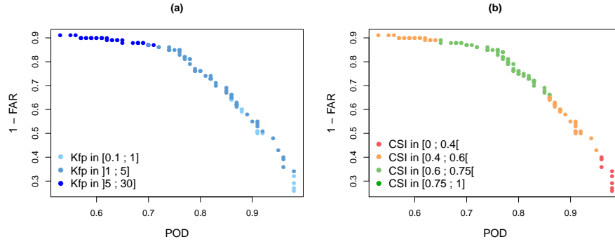
Figure 10. Pareto diagram for two forecast scores, POD and FAR . 1 - FAR is used so that each criterion evolves in the same way, (a) distribution of K_{fp} values and (b) distribution of CSI values according to POD and 1 - FAR .
