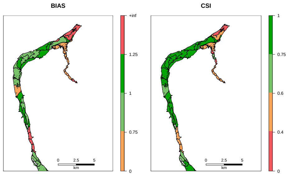
Fig. 1. Reach-scale performance for the physical combination of parameters, for the downstream part of the catchment.
