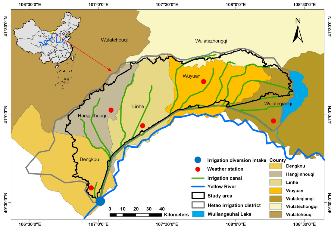
Fig. 1. Fig. 1. Location of the Hetao Irrigation District (HID) in China
