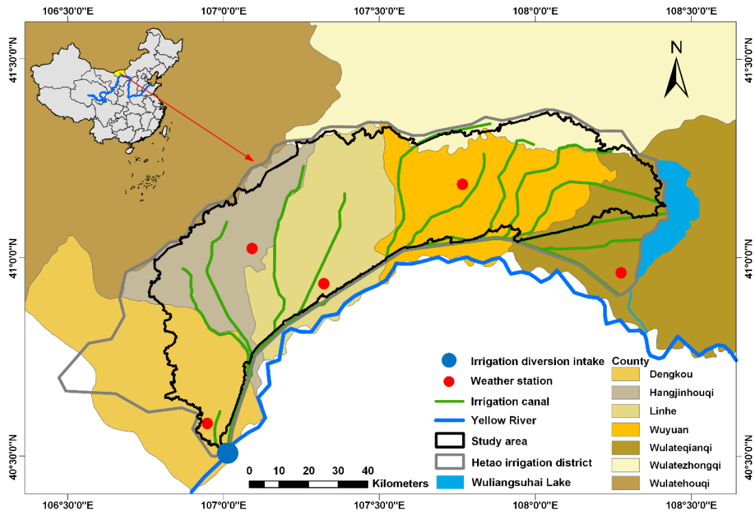
Fig. 1. Location of the Hetao Irrigation District (HID) in China
