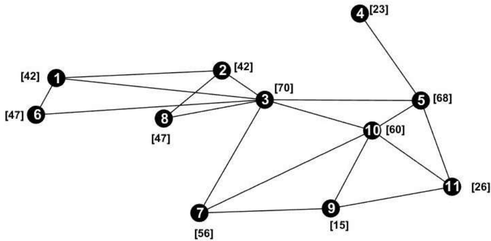
Figure A1: Location Sample rain gauge network of eleven randomly selected rain stations (a), used to construct a complex network based on the cross-correlation similarity measure and 90 th percentile threshold (b) only for illustrative purposes. Autocorrelation (diagonal) has been ignored in the network construction. Numbers 1 to 11 are node counts, and values in brackets represent the WDB values.
