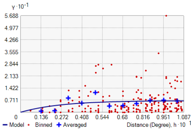
Figure A2: Typical variogram model (a) and fitted variogram models for daily mean (b), 90 th (c), 95 th (d), and 99 th (e) percentile precipitation and for mean (b), 90 th percentile (c), 95 th percentile (d), 99 th percentile (e) precipitation and number of wet days (f).
