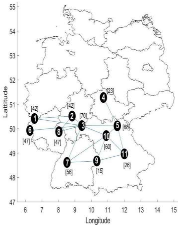
5 Figure A1: Location of eleven randomly selected rain stations used to construct a complex network based on the cross-correlation similarity measure and 90 th percentile threshold. Diagonal values (autocorrelation) in Table 1 have been ignored in network construction. Numbers 1 to 11 are node counts, and values in brackets represent the WDB values.
