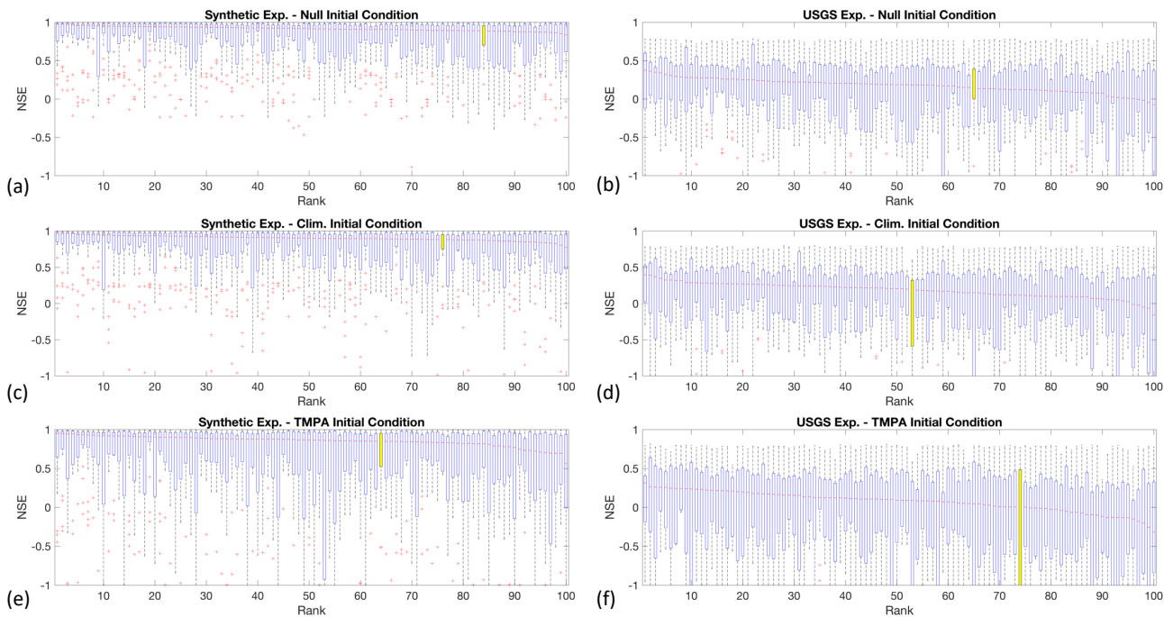
5 Figure 10: Box plots of NSE values at 25 validation sites for 100 random configurations of the gauge network. Experiments are divided into two categories: the entirely synthetic discharge reconstructions (a,c,e) and the discharge reconstructions from USGS observations (b,d,f). These experiments are further differentiated by the three initial runoff conditions used: Null (a,b), Climatology (c,d), and TMPA derived (e,f). The yellow box plots represent the gauge network configuration used for the results presented in this study.
