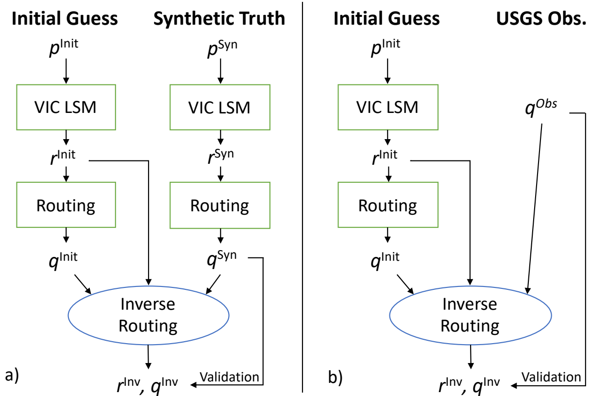
5 Figure 2: a) Overall process flow diagram for the synthetic experiments with the ISR model, where p is the input precipitation for the VIC LSM distributed over the study domain and study period, r is the runoff fields distributed over the same space, and q is discharge at discrete points during the study period. The superscripts “Init” and “Syn” represent the initial guess and the synthetic truth, respectively, while the “Inv” superscript indicates the products resulting from the model. b) Overall process flow diagram for the ISR model, substituting actual USGS discharge observations for the synthetic truth of the previous experiments.
