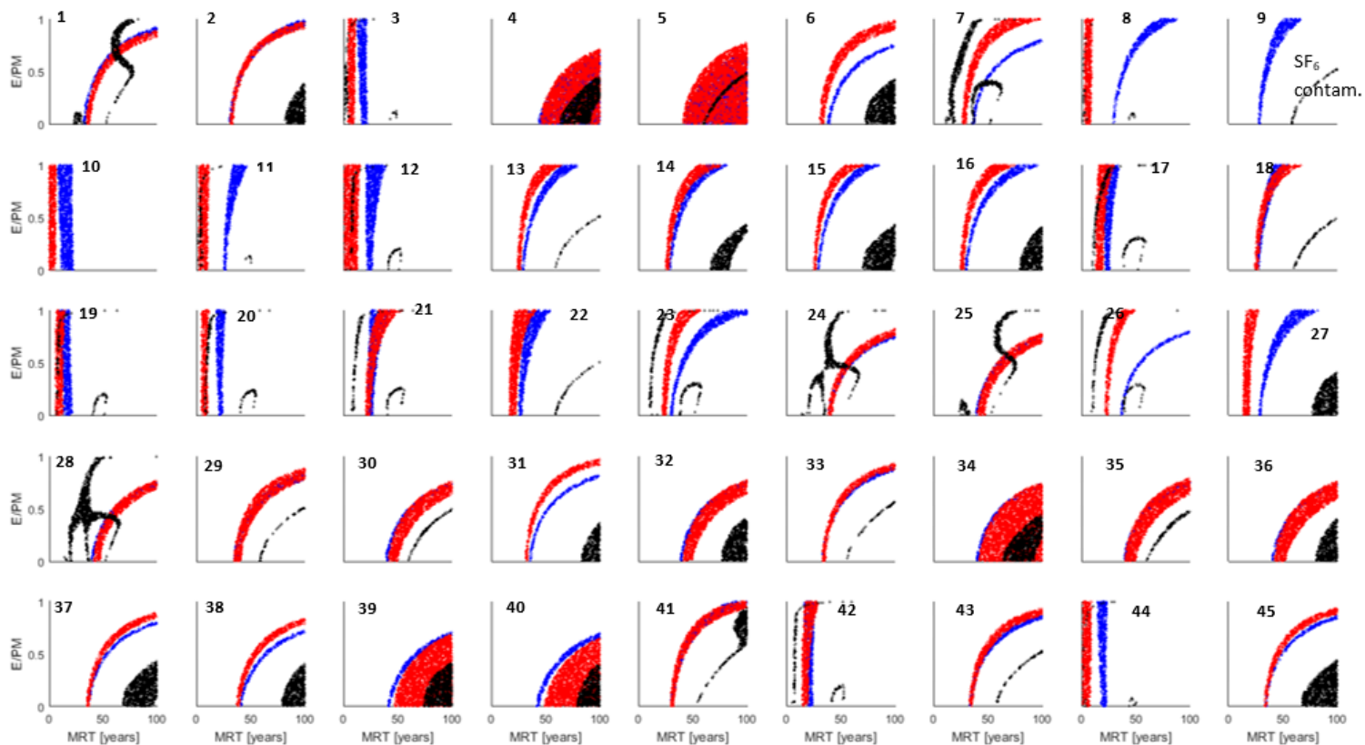
Figure 14: Behavioural age information (MRT and E/PM) inferred from SF 6 (red), tritium (black) and Halon-1301 (blue) for sites 1 to 45
