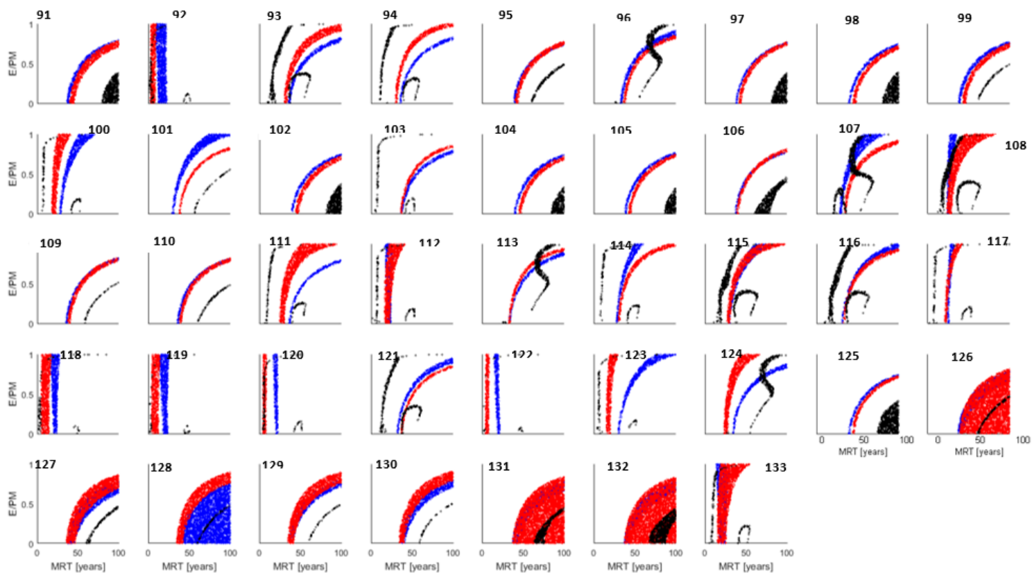
Figure 16: Behavioural age information (MRT and E/PM) inferred from SF 6 (red), tritium (black) and Halon-1301 (blue) for sites 91 to 133
