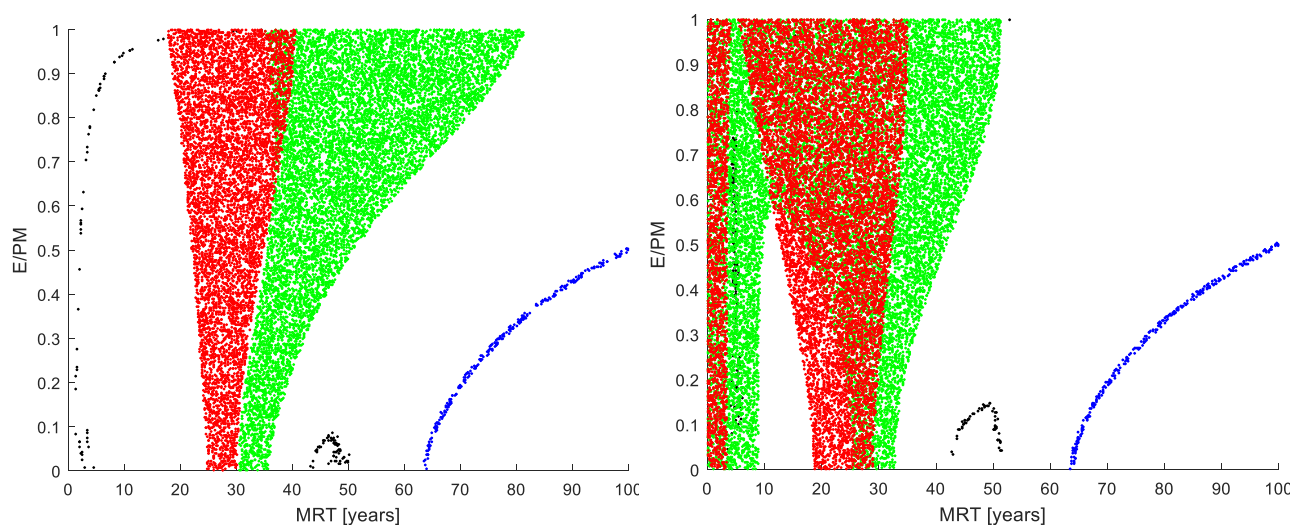
5 Figure 8: Typical EPM parameter could be inferred with tritium (black), CFC-11 (green), CFC-12 (red) and CFC-113 (blue). In both figures tritium and CFC-11 and CFC-12 inferred LPM parameter clouds overlap, i.e. age interpretations agree; in both figures, tritium gives ambiguous age estimates, in right figure CFC-11 and CFC-12 also give ambiguous age estimates due to recently falling atmospheric concentrations.
