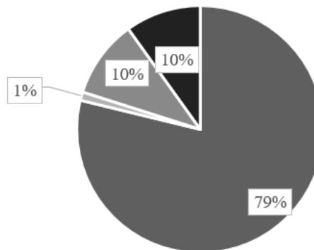
Figure 11: Summary of performance of Halon-1301 as an age tracer compared to tritium in predicting the MRT (upper) and the mixing parameter E/PM (lower). Overall, at 99 % of the sites MRTs agree within +/- 10 %.
