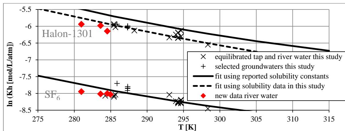
15 Figure 5: estimated solubility of Halon-1301 and SF 6 in equilibrated tap water, river water, and oxic young groundwater in comparison to reported solubility data, * data from Deeds (2008) for Halon-1301 and Bullister et al. (2011) for SF 6
