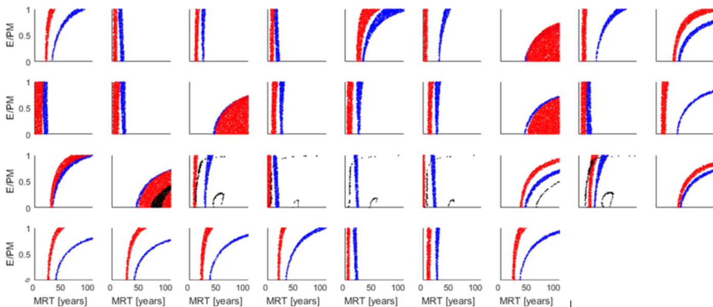
Figure 20: Behavioural age information (MRT and E/PM) inferred from SF 6 (red), tritium (black) and Halon-1301 (blue) for sites 268 to 302
