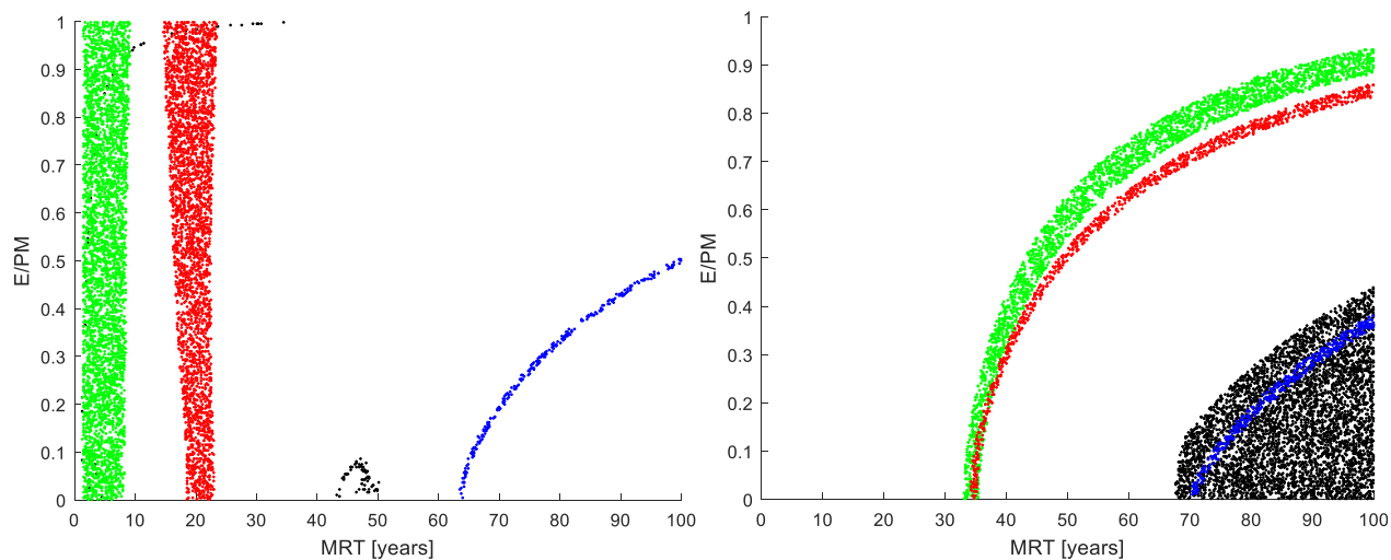
5 Figure 10: Typical EPM parameter could be inferred with tritium (black), SF 6 (green), Halon-1301 (red) and CFC-113 (blue). In both figures some agreement of age interpretations is evident through overlapping LPM parameter clouds. In the left figure tritium age interpretation is ambiguous; the younger part agrees with the SF 6 and Halon-1301 inferred age. In the right figure the tritium and CFC-113 inferred age agrees, but differs from Halon-1301 and SF 6 inferred ages (which agree with each other).
