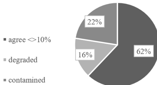
CFC-11 and tritium inferred MRTs
