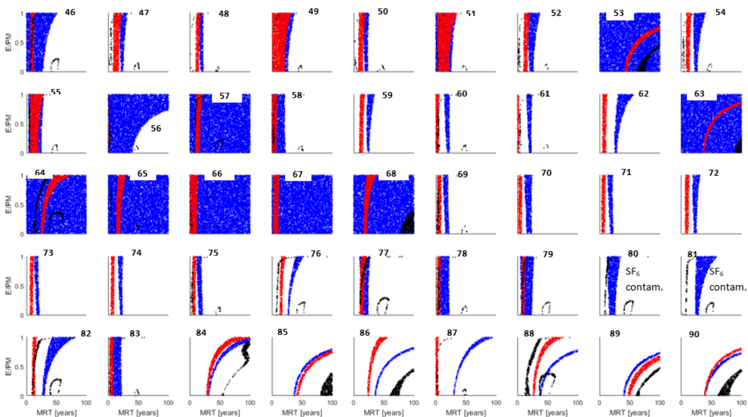
Figure 15: Behavioural age information (MRT and E/PM) inferred from SF 6 (red), tritium (black) and Halon-1301 (blue) for sites 46 to 90
