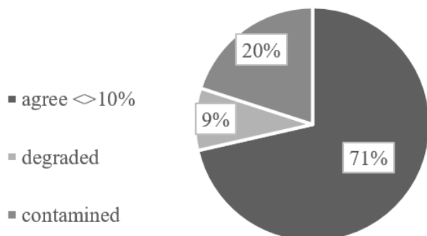
CFC-12 and tritium inferred MRTs
