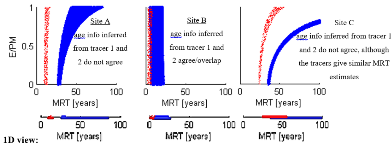
5 Figure 4: Example of behavioural lumped parameter model (LPM) parameter clouds inferred from two different tracers (tracer 1 in red and tracer 2 in blue). For site B (MIDDLE) the inferred LPM parameter clouds overlap, indicating that the age interpretation inferred from each tracer agree. For site A and C (left and right) the inferred LPM parameter clouds do not overlap, indicating that the two tracers give different age interpretations. For site C the tracers give similar MRT estimates giving the impression that the tracers age info agree when only looking at one dimension (bottom of each figure). To quantify difference/disagreement, the distance between the data clouds can be determined. [it might be useful to have one more example where the age info 1 and 2 overlap only at a certain E/PM ratio – this is a very realistic scenario using two tracers to constrain the E/PM ratio]
