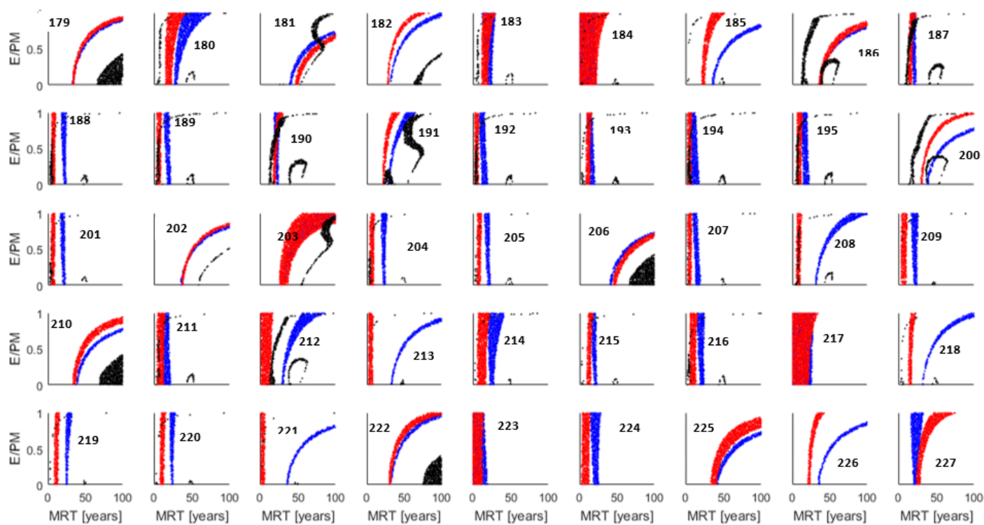
Figure 18: Behavioural age information (MRT and E/PM) inferred from SF 6 (red), tritium (black) and Halon-1301 (blue) for sites 179 to 227
