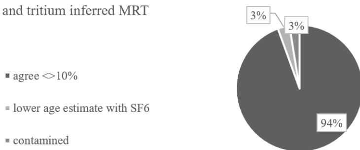
Figure 9: Agreement of SF 6 and tritium inferred MRTs. The data suggest that for most sites SF 6 inferred MRTs match tritium inferred MRTs. Only few sites (3 %) were contaminated with SF 6 and another 3 % showed lower age estimates with SF 6 than with tritium, which could result from a thick unsaturated zone and associated travel time to the aquifer.
