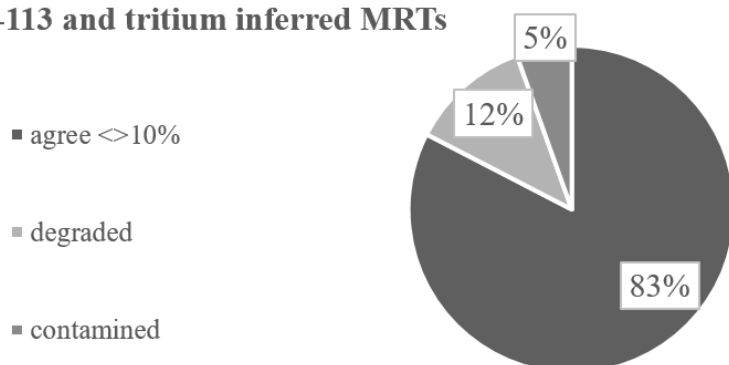
10 Figure 7: Agreement of CFC-113 inferred MRTs compared to those inferred with tritium, suggesting that for most sites MRTs inferred from CFC-13 match tritium inferred MRTs. Some (5 %) of the sites are contaminated with CFC-113 or (12 %) degraded in CFC-113. Overall CFC-113 performs considerably better than CFC-11 or CFC-12.
