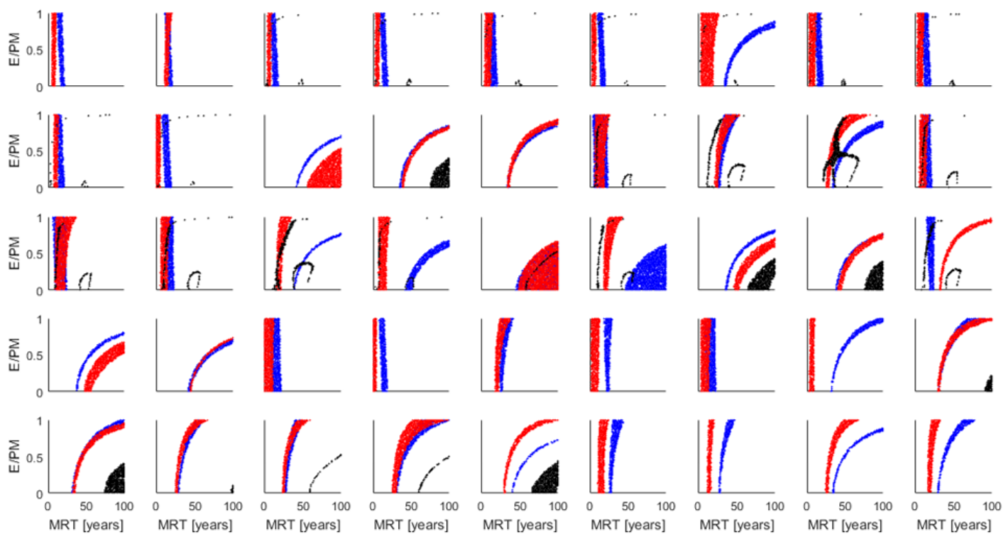
Figure 19: Behavioural age information (MRT and E/PM) inferred from SF 6 (red), tritium (black) and Halon-1301 (blue) for sites 228 to 270
