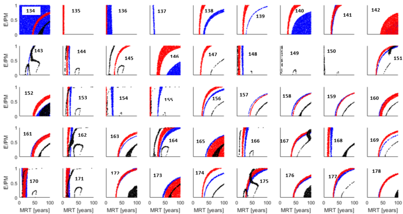
Figure 17: Behavioural age information (MRT and E/PM) inferred from SF 6 (red), tritium (black) and Halon-1301 (blue) for sites 134 to 178
