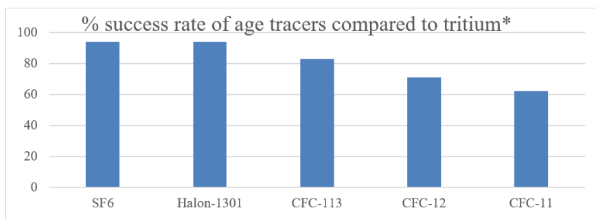
Figure 13: Success rate of Halon-1301, SF 6 and the CFC -11 and -12 compared to tritium in this study; *assuming tritium has a success rate of 100 %
