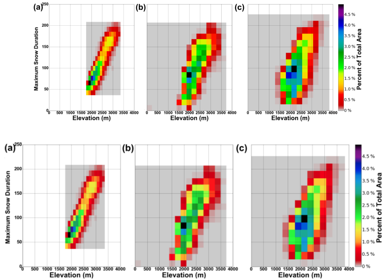
405 Figure 98: Heat maps showing the relationship between elevation and average maximum snow duration for three seasonally-dominant ecoregions in the Great Basin: (a) The Ruby mountains, (b) the Sierra Nevada mountains, and (c) the Wasatch/Uinta mountains.
