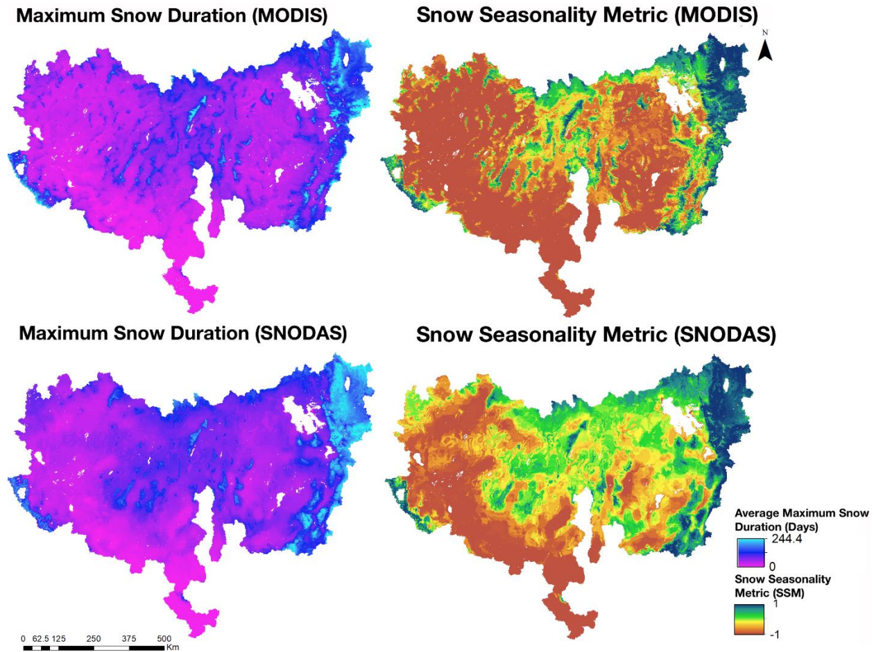
Figure 75: Average maximum consecutive snow duration ( Maximum maximum snow duration) and snow seasonality metric (SSM) for the Great Basin measured using moderate resolution imaging spectroradiometer (MODIS) and snow data assimilation system (SNODAS) data in the Great Basin, USA. MODIS data is from water years 2001-2015 and SNODAS data is from for water years 2005-2014.
