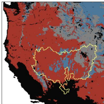
Figure 1410: Dominant mechanisms causing for snow ephemerality from water years 2009-2014 in the Western United States. Data obtained from SNODAS. Areas with seasonal snow, (grey), no snow, (black), and water bodies (black) are also depicted as black. The Great Basin region is outlined in yellow.
