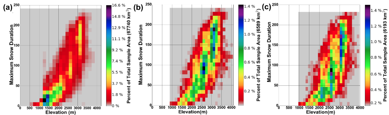
Figure 8: Heat maps showing the relationship between elevation and average maximum consecutive snow duration from MODIS at (a) all slopes, (b) north-facing slopes only, and (c) south-facing slopes only in the Great Basin, USA. North facing was defined as Northness > 0.25 and south facing was defined as Northness < -0.25. The colors correspond to Color bar scale is different in panel (a) reflecting the much larger area within each at low elevation and maximum snow duration.
