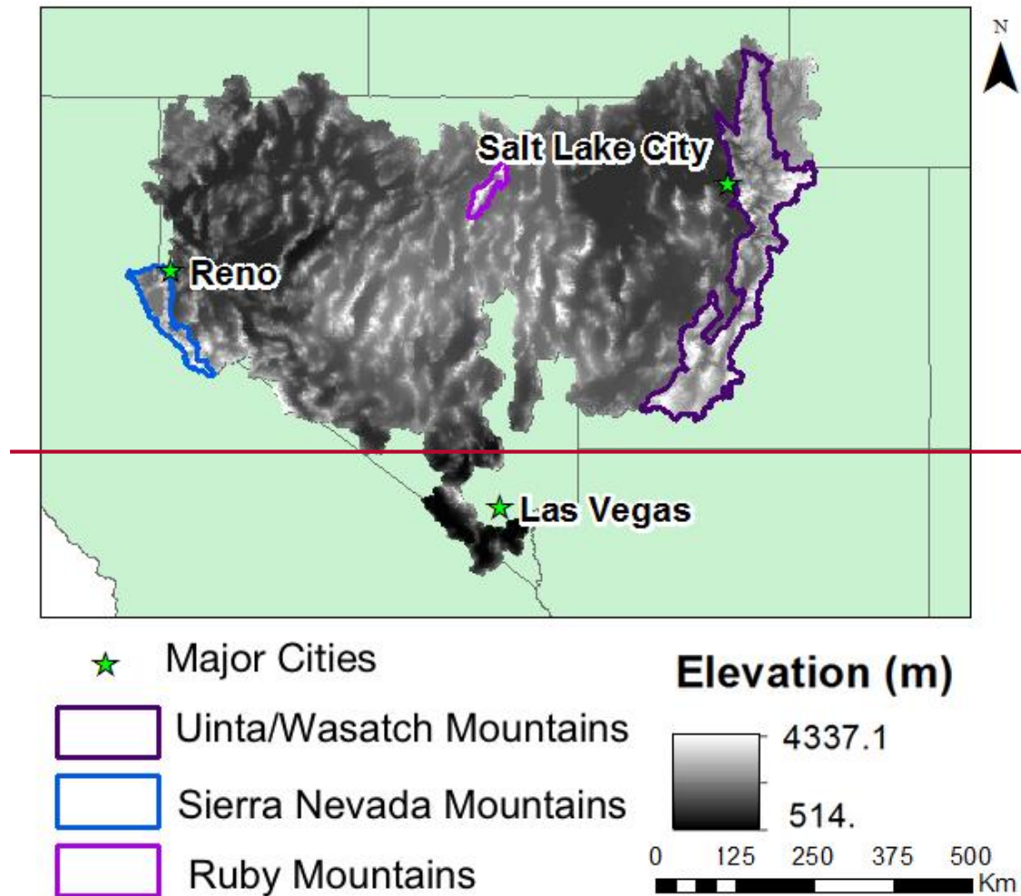
170 Figure 2: Map of the Great Basin region, USA as defined by the United States Geological Survey (USGS) Hydrologic Unit Code (HUC) Region 16 along with major cities and mountain ranges. The Sierra Nevada and Wasatch/Uinta mountain ranges defined using the US EPA L4 ecoregion classifications of “Sierra Nevada” and “Wasatch Uinta” respectively. Ruby Mountains were defined using a combination of “Mid-Elevation 175 Ruby Mountains” and “High Elevation Ruby Mountains” in the US EPA L3 classification (Omernik, 1987). Elevation contours at 1000 m intervals.
