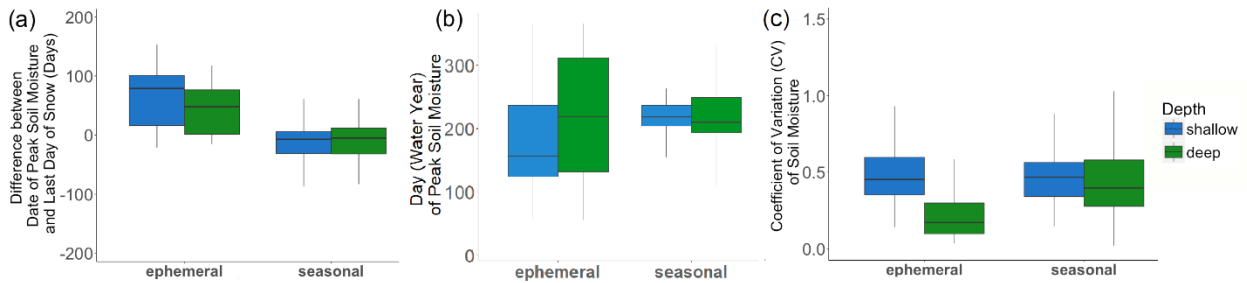
Figure 64: (a) The difference between date of peak soil moisture and last day of snow (Days) for shallow (5 cm) and deep (50 cm) soil moisture during water years 2014-2016 in Great Basin SNOTEL stations with ephemeral snow (50 site years) and seasonal snow (278 site years). (b) Day of peak soil moisture for SNOTEL and SCAN stations for shallow (5 cm) and deep (50 cm) soil moisture during water years 2014-2016 (c) The coefficient of variation (CV) for shallow (5 cm) and deep (50 cm) soil moisture during water years 2014-2016 in Great Basin SNOTEL and SCAN stations is also shown.
