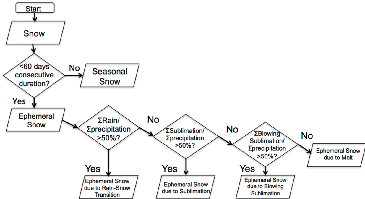
Figure 42: Diagram of the process for the ephemeral snow mechanism model. Seasonal snow outputs were rejected, all other outputs were categorized.
