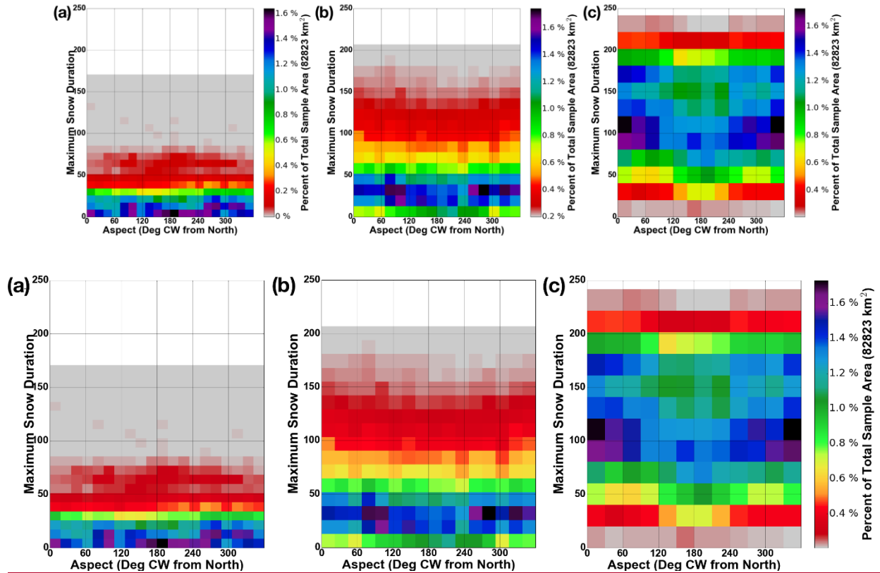
Figure 10: Heat maps of the relationship between aspect and average maximum consecutive snow duration at (a) low elevations (0-1500 m), (b) medium elevations (1500-2500 m) and (c) high elevations (>2500 m).
