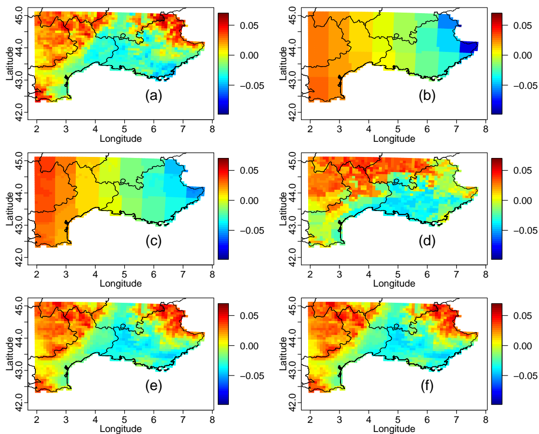
Figure 2. Maps of first temperature EOFs in winter over the evaluation period for (a) SAFRAN; (b) ERA-I; (c) 1d-BC (CDF-t); (d) 2d-R 2 D 2 (with PR as reference dimension); (e) 1506d-R 2 D 2 (on T2 only); (f) 3012d-R 2 D 2 .
