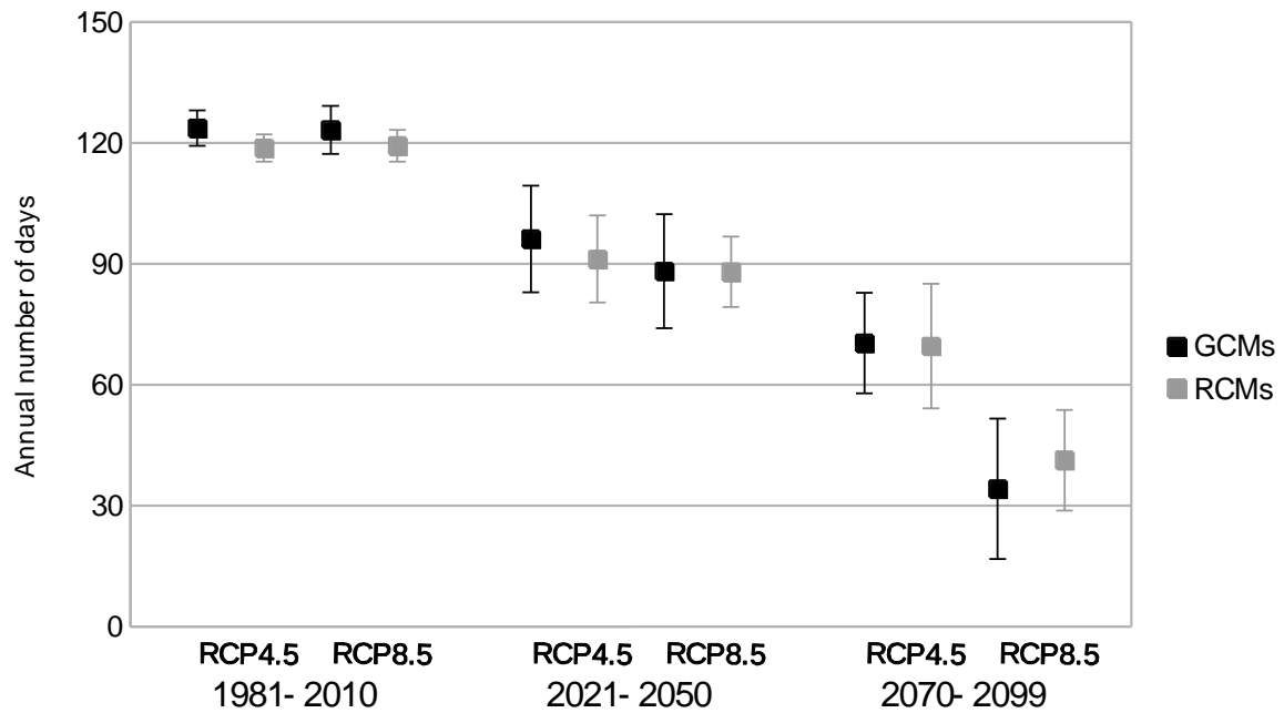
Figure 7. Annual mean number of days with good wintertime bearing capacity in drained pine-dominated peatland forests with multi-model standard deviations as averaged over whole of Finland separately for the GCM and RCM ensembles during the periods 1981–2010, 2021–2050 and 2070–2099 under the RCP4.5 and RCP8.5 scenarios.
