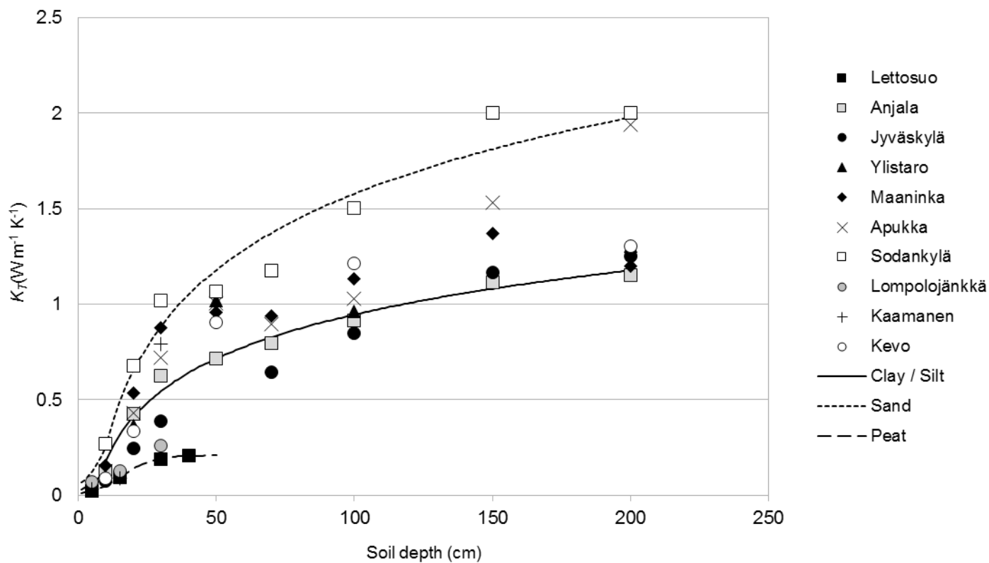
Figure 1. Calibrated K_T values at each soil temperature measurement site and depth. Logistic regression curves fitted to the data from Anjala, Sodankylä and Lettosuo stations representing clay/silt, sand and peat soil types, respectively, are shown as well.
