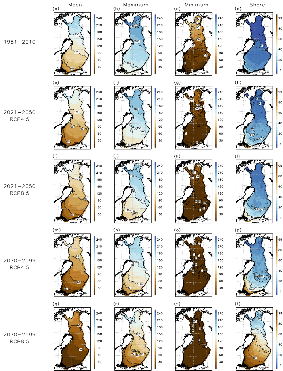
Figure 5. Modelled multi-GCM annual mean number of days with good bearing capacity in drained pine-dominated peatland forests during 1981–2010, 2021–2050 and 2070–2099 under the RCP4.5 and RCP8.5 scenarios (left panel). The second and third panel from the left show the modelled annual number of days with good bearing capacity during the winter with most (the second panel) and least (the third panel) such days within the 30-year periods based on the same multi-GCM mean. The last panel shows the share of winters (%) with less than 30 modelled days of good bearing capacity based on the multi-GCM mean.
