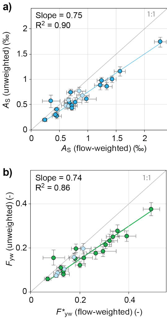
5 Figure 5: Panel a) compares the seasonal amplitudes of streamwater isotope cycles ( A_s ) with and without flow weighting. High-elevation, snowmelt-dominated sites are marked in light blue. Panel b) compares flow-weighted young water fractions F_{yw}^* with unweighted young water fractions ( F_{yw} ). Error bars show \pm 1 standard error. Unweighted young water fractions are roughly 26% smaller than flow-weighted young water fractions across these catchments.
