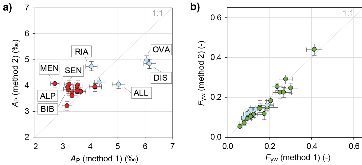
5 Figure 3: a) Comparison of flow-weighted seasonal amplitudes of precipitation \delta^{18}\text{O} cycles ( A_P ) obtained with two different interpolation methods, method 1(Seeger and Weiler, 2014) and method 2 (based on Allen et al., 2018; Supplement), respectively. Differences in A_P between the two interpolation methods were significant for the catchments highlighted with their abbreviated names. The abbreviations for the study sites stand for Allenbach (ALL), Alp (ALP), Biber (BIB), Dischmabach (DIS), Mentue (MEN), Ova da Clouzza (OVA), Ria di Calneggia (RIA), and Sense (SEN). b) Comparison of young water fractions derived from the two interpolation methods. High-elevation, snow-dominated catchments are marked in light blue colour. Error bars show \pm 1 standard error.
