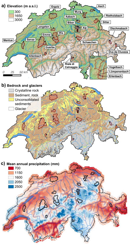
Figure 2: Locations of the 22 study catchments in Switzerland (a), bedrock geology (b), and mean annual precipitation based on the observation period 1991-2019 (c). The expanded panel in (a) shows the sub-catchments of the Alp basin.
