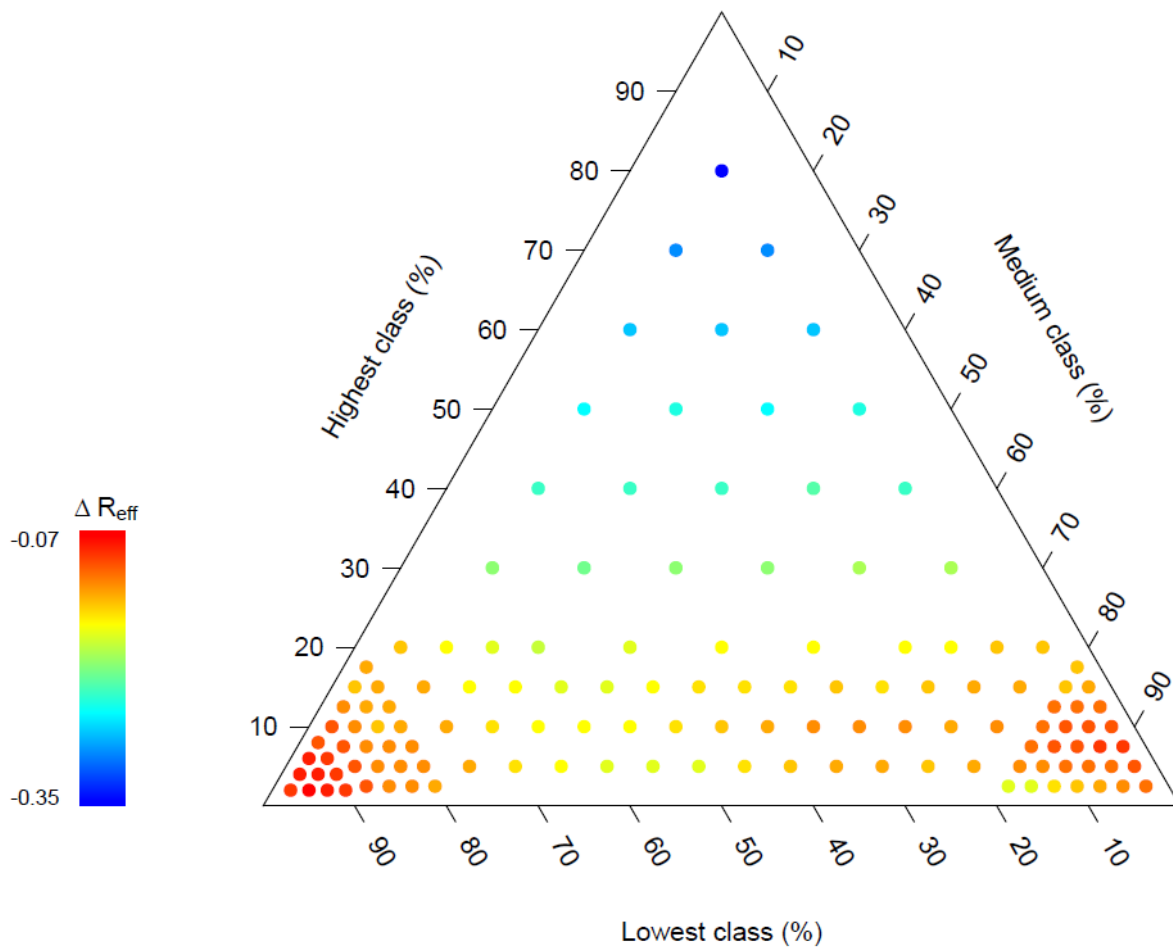
Figure 6. Median difference in model efficiency (for models calibrated with data for three water level classes and the upper benchmark ( \Delta R_{eff} ) for different class boundaries.
