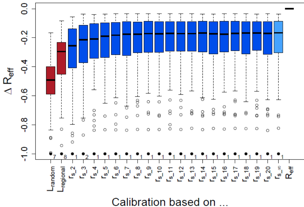
5 Figure 2. Box plots of the difference in the median model efficiency and the upper benchmark ( \Delta R_{eff} ) for all 100 catchments for the models calibrated on stream level class data (2 to 20 classes; r_{s_n} ), models calibrated on high-resolution stream level data ( r_{s_\infty} ), and the two lower benchmarks ( L_{random} and L_{regional} ). The box represents the interquartile range, the solid line the median, the whiskers reach to the furthest catchment that is still within a distance of 1.5 times the interquartile range from the box and the dots represent the outliers.
