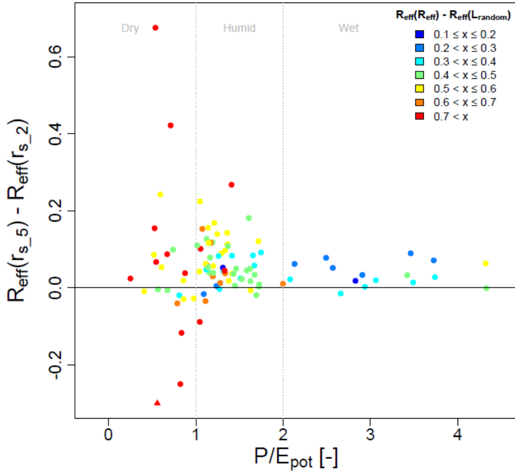
5 Figure 3. Difference in the median model validation result (model efficiency) for the models calibrated using two water level classes ( r_{s_2} ) and five water level classes ( r_{s_5} ) for all 100 catchments as a function of the aridity index ( P/E_{\text{pot}} ). The color of the symbols represents the difference between the upper and the lower benchmark (i.e. the difference in the median model performance when the model is calibrated with all available streamflow data ( R_{\text{eff}} ) and when the model is run with randomly selected parameters (i.e. without any calibration; L_{\text{random}} )). Triangles indicate outliers that would plot outside the range of the y-axis.
