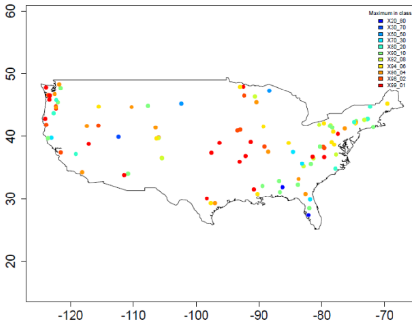
Figure 5. Difference in median model validation results relative to the upper benchmark ( AR_{eff} ) for models calibrated with two water level classes for different class boundary definitions (a) and a map of the optimal class boundary definition for each catchment (b). 5 As an example, 10-90 indicates that streamflow was in the lower water level class for 10% of the time and in the upper class for 90% of the time. The median difference in model efficiency is smallest when the class boundaries are set at 93-7%.
