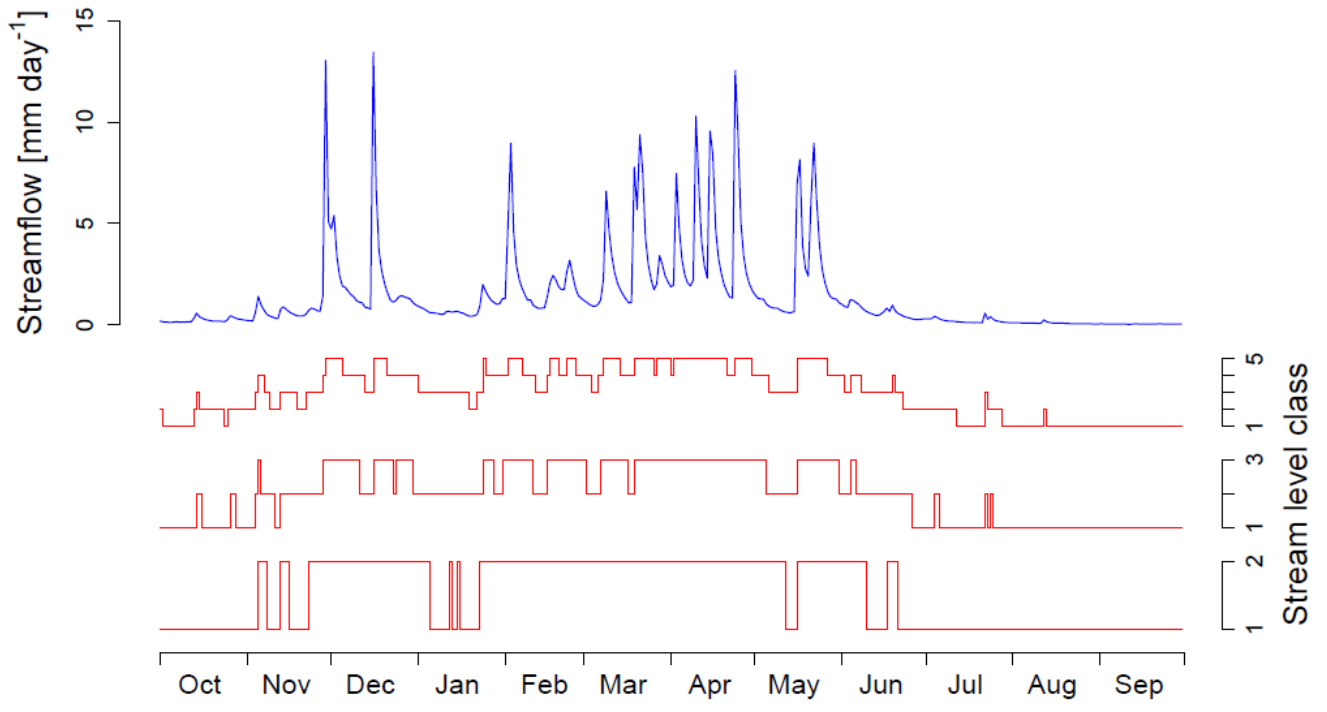
5 Figure 1. Time series of the observed streamflow (blue) for the first year of simulation (October 1982 – September 1983) for the catchment 002011460 (Back Creek near Sunrise, VA, a medium sized catchment (235 km 2 ) with a medium aridity index (1.33) and the derived time series of stream level class for the case of two, three and five level classes (red), where the stream level is in each water level class for, respectively, 50%, 33% and 20% of the time.
