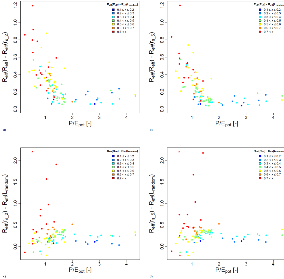
5 Figure 4. Difference in model validation results (model efficiency) for the models calibrated with data from two ( r_{s_2} ; left) and five ( r_{s_5} ; right) stream level classes and the upper benchmark ( R_{eff} ) (upper row) and the lower benchmark ( L_{random} ; bottom row) as a function of the aridity index ( P/E_{pot} ). Each dot represents one catchment; the color of the symbol represents the difference in model efficiency between the upper and lower benchmark for that catchment. Note the difference in the scale of the y-axis for the comparison to the upper benchmark (upper row; a and b) and the lower benchmark (lower row; c and d). Triangles indicate outliers that would plot outside the range of the y-axis.
