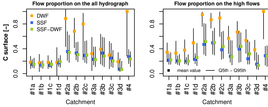
Figure 13. Proportion of surface runoff in the flows at the outlet. Left: The proportion over the whole hydrograph; right: the proportion at high discharges (Observed flow greater than 0.25 times the maximum flow during the event).
