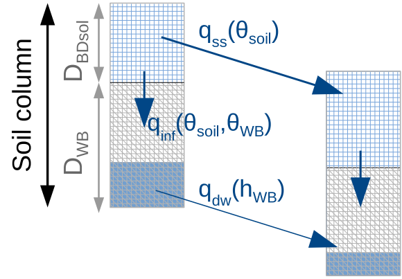
Figure 7. SSF and SSF-DWF models: flow generation by the saturation of the upper part of soil column and activation of preferential paths ( q_{ss} ), with support flow at depth ( q_{dw} ), and water exchanges from the upper layer to the lower one according to both soil water content ( q_{inf}(\theta_{soil}, \theta_{WB}) ). See equations 2, 3 and 4, for the definition of the flows.
