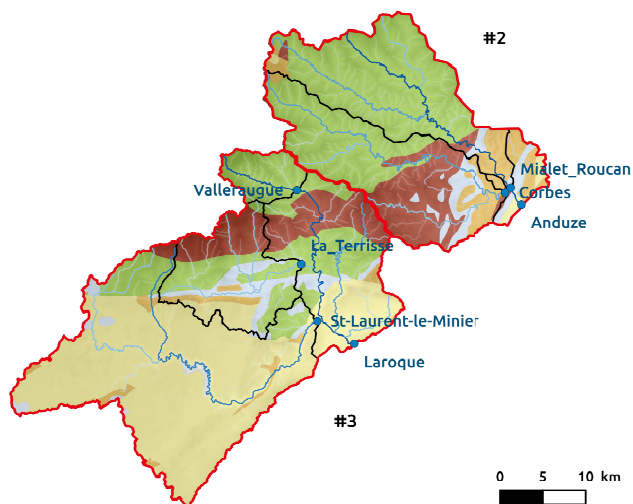
Figure 3. The geology of the Gardon and Hérault catchments (sources : BD Million-Géol, BRGM)
