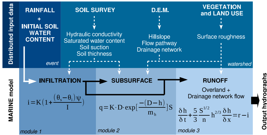
Figure 5. The MARINE model structure, parameters and variables. The Green and Ampt infiltration equation contains the following parameters: infiltration rate i ( \text{m.s}^{-1} ), cumulative infiltration I (mm), saturated hydraulic conductivity k ( \text{m.s}^{-1} ), soil suction at the wetting front \Psi (m), and, saturated current and initial water contents, \theta_s and \theta_i ( \text{m}^3.\text{m}^{-3} ), respectively. Subsurface flow contains the following parameters: soil thickness (m), lateral saturated hydraulic conductivity K ( \text{m.s}^{-1} ), local water depth h (m), transmissivity decay with depth m_h (m), and bed slope S ( \text{m.m}^{-1} ). The kinematic wave contains the following parameters: surface water depth h (m), time t (s), space variable x (m), rainfall rate r ( \text{m.s}^{-1} ), infiltration rate i ( \text{m.s}^{-1} ), bed slope S ( \text{m.m}^{-1} ), Manning roughness coefficient n ( \text{m}^{-1/3}.\text{s} ). The Module 2 described in this figure corresponds to the standard definition applied to the MARINE model. It corresponds, in fact, to the scope of model modifications proposed in this study, which are described in the next section (section 3.2.)
