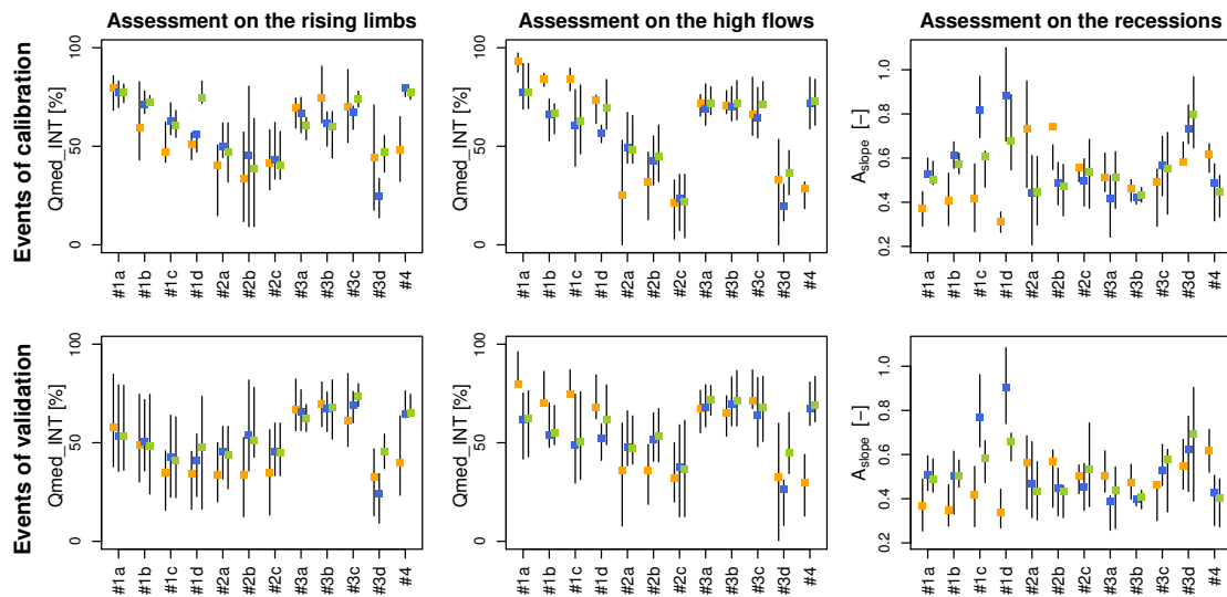
Figure 10. Assessment of the models by catchment over the different stages of the hydrographs. Left : Q_{med\_INT} scores calculated over the rising flood waters stage; center: Q_{med\_INT} scores calculated over the high discharges stage; right: A_{slope} scores. High Q_{med\_INT} scores and conversely low A_{slope} values indicate good performances of the model. Comparison of the modelled and observed characteristics of flood recession. Black: flood recession points for observed flows; orange: flood recession points for flows modelled using the DWF model; blue: flood recession points for flows modelled with the SSF model; green: flood recession points for flows modelled with the SSF-DWF model.
