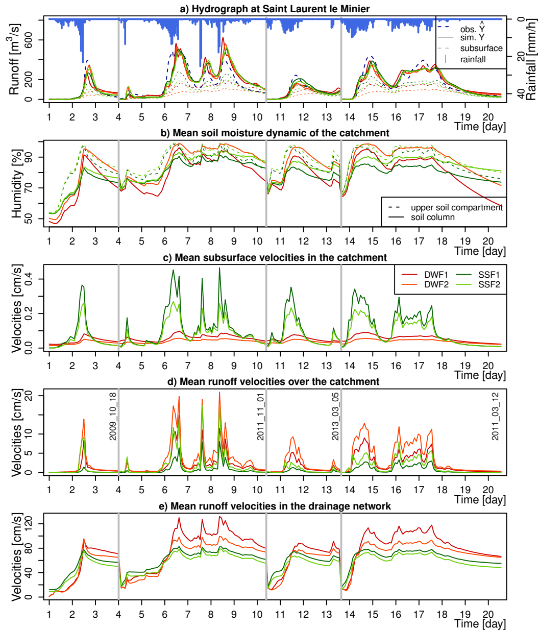
Figure 14. Comparison of the results of four equally plausible simulations on the Hérault at Saint Laurent le Minier (Table 3). a) Flood hydrographs (solid lines) and outlet flows transiting via the soil (dashed lines). b) Evolution in the overall moisture content of the soil column. c) Evolution in simulated mean velocities in the subsoil horizon (DWF model) and in the upper part of the soil column (SSF model). d) Average runoff velocities on the hillslopes. e) Average runoff velocities in the drainage network.
