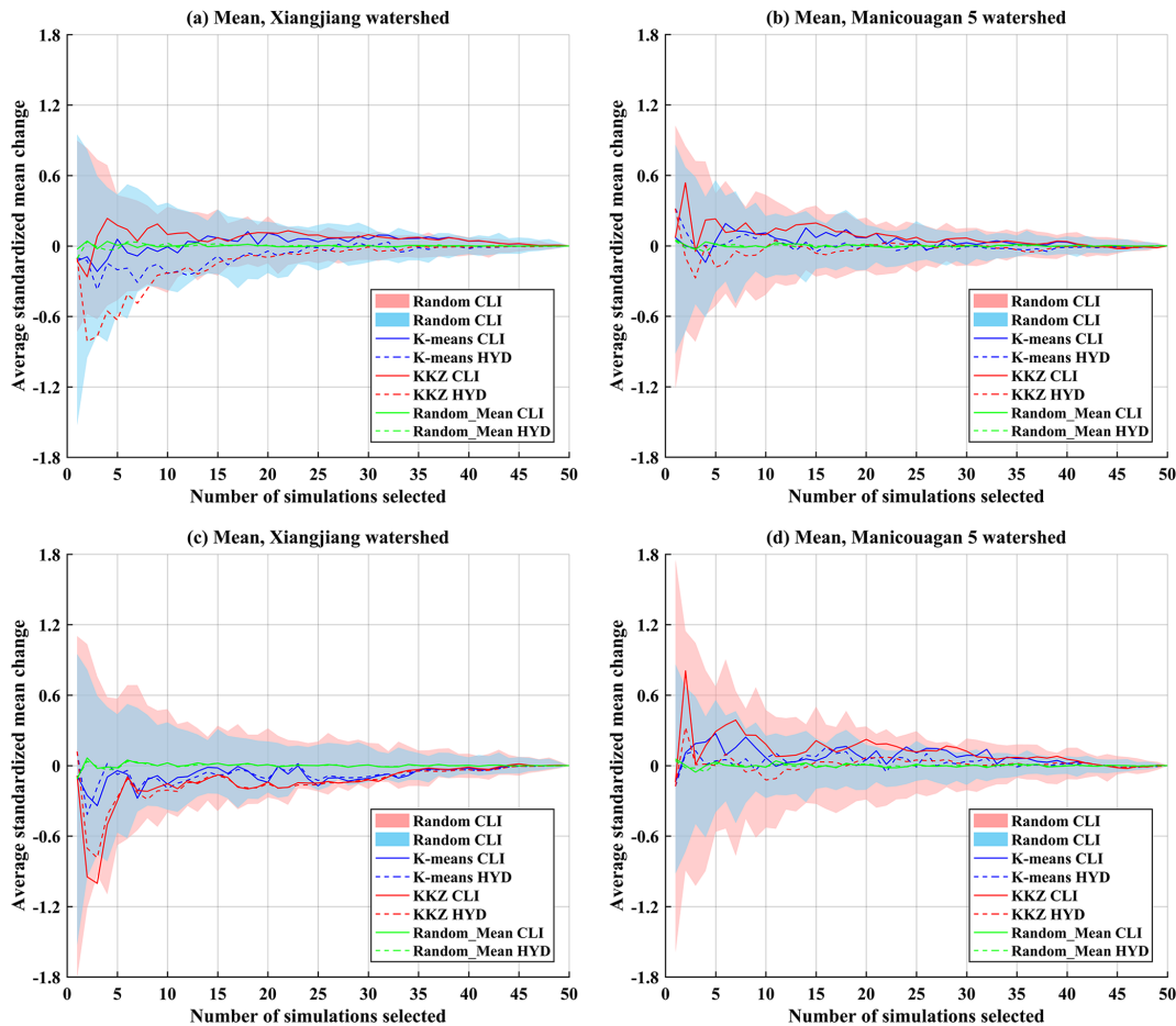
Figure 9. Averaged standardized mean changes in climate (CLI) and hydrological (HYD) variables of subsets selected by three selection methods ( K means, KKZ and random selection) over the Xiangjiang and Manicouagan 5 watersheds when temperature variables are (a, b) included or (c, d) excluded in the process of selection. The pink and blue panels are the envelopes resulting from 100 random selections.
