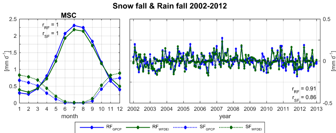
Fig. 5. Comparison of the mean seasonal cycle and interannual variability of rain fall and snow fall from WFEI product and from GPCP (snow fall as in the optimized model)
