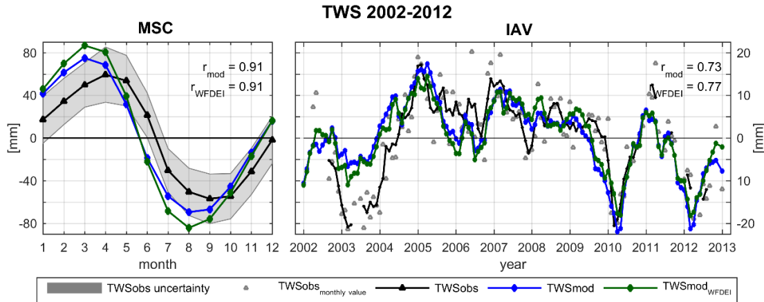
Fig. 4. Comparison of the mean seasonal cycle and interannual variability of TWSObs (GRACE), TWSmod (forced with GPCP precipitation) and TWSmodWFDEI (forced with WFDEI rain and snow fall)
