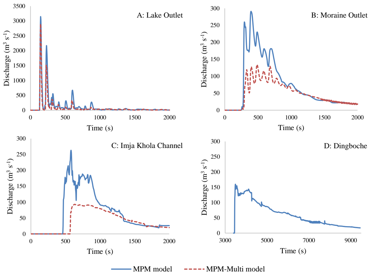
10 Figure 8: Combined sediment and water discharge for first 2000 s after initial wave generation from a large southeast avalanche at all three cross sections for both the MPM model (blue line) and the MPM-multi model (red line), plus debris discharge for first 9500 s at Dingboche for the MPM model. Note the larger discharge scale of (A).
