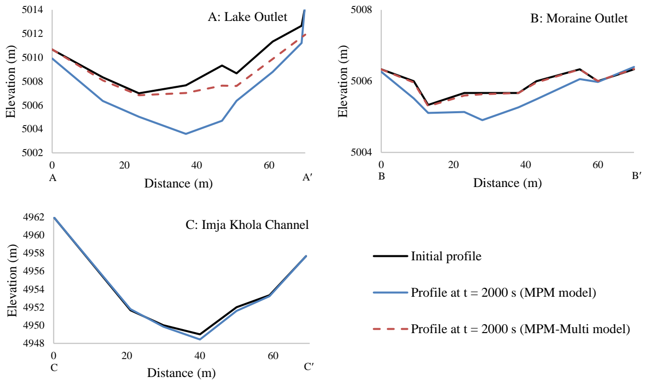
Figure 9: Surface elevation profiles at the start of wave generation (solid black line) from large southeast avalanche and 2000 s after generation at all three cross sections, for both the MPM model (solid blue line) and the MPM-Multi model (dashed red line), at the lake outlet (A), moraine outlet (B), and Imja Khola channel (C) transects shown in Figure 7. Note the smaller scale of (B). The MPM-Multi model at (C) lacked measurable erosion and is not shown.
