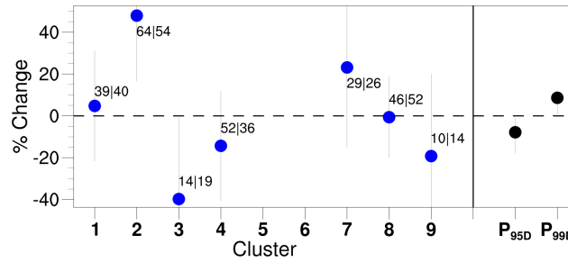
Figure 9. Percentage change in daily precipitation intensity between the historical and RCP8.5 periods (JJA), conditional on extremal circulation pattern, from the 0.02° simulations. The numbers indicate the total number of PEDs for each pattern (i.e. cluster) in the historical (left) and RCP8.5 (right) periods, while vertical bars represent 90% confidence intervals. Clusters with less than 10 days in either period are excluded from the calculations. On the right hand side, the corresponding climate change signal for the 95 th and 99 th percentile of all days is provided for reference.
