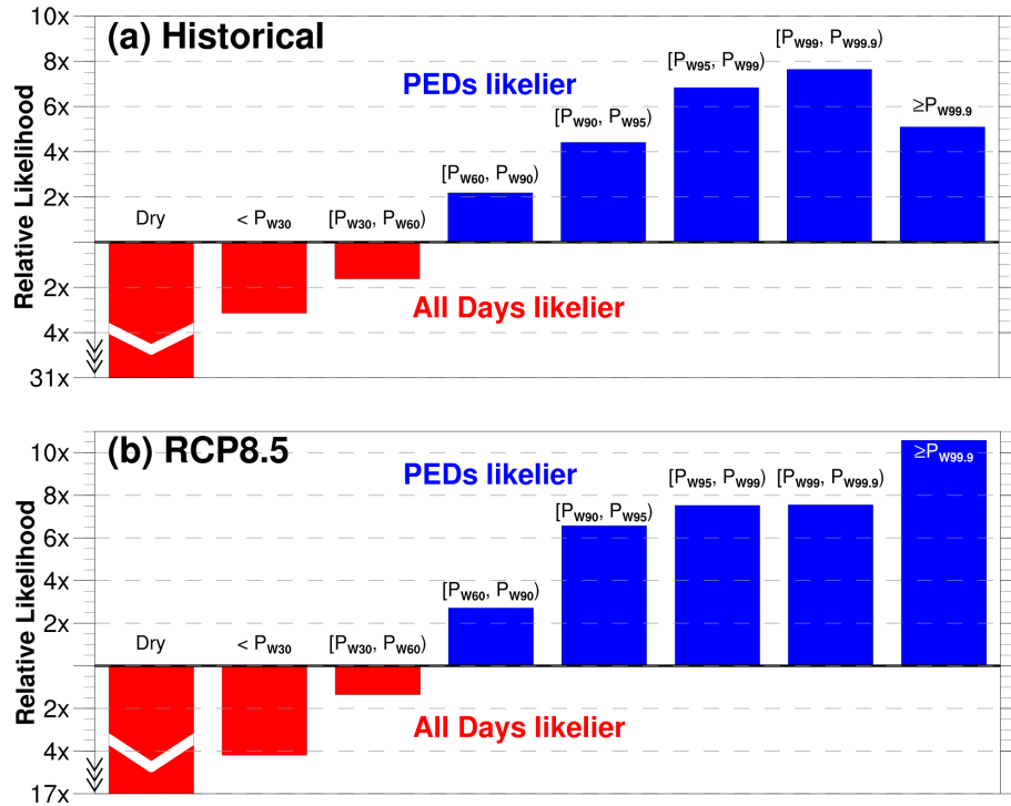
Figure 8. Relative likelihoods of precipitation on a randomly sampled day from the set of all days and the PEDs being within a given intensity range for the (a) historical and (b) RCP8.5 0.02° simulations. Note that precipitation intensities are based on the percentiles of wet days ( P_D \geq 0.1 mm)
