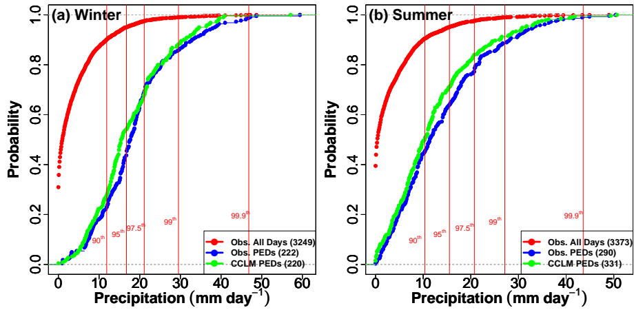
Figure 5. Empirical cumulative distribution functions of daily precipitation for all days (red, observed), PEDs (blue, observed), and CCLM PEDs (green, downscaled to 0.02^\circ ). (a) Winter 1980-2015, (b) summer 1979-2015 (up to 31.07.2015). Differences between the blue and red curves (REGNIE) highlight the increased likelihood of heavy rainfall events amongst the PEDs. All values are area averages over the Wupper catchment. Vertical red lines mark important percentiles of the all-day distribution. The area of the Wupper catchment encompasses 753 and 161 grid cells of REGNIE and CCLM data, respectively. Stations in and around the Wupper catchment are marked in Fig. 2. The similarity of the blue (REGNIE) and green (CCLM) PED-curves shows that, with skilful identification of PEDs, convection-permitting downscaling can well-reproduce the observed PED statistics.
