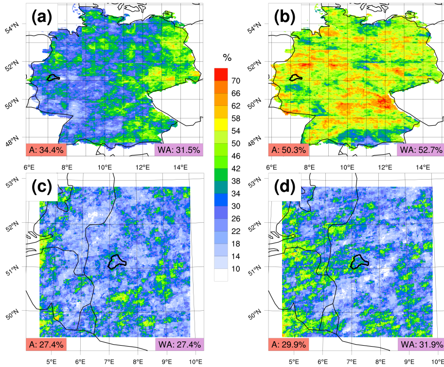
Figure 1. Coarse model extreme precipitation is a poor predictor of extreme precipitation in both observations and high-resolution simulations. Plots show the rate at which extreme precipitation events in a coarse model are temporally/spatially coincident with extreme precipitation events in (a, b) observations and (c, d) further downscaled high-resolution simulations. (a) For summer extreme precipitation (1979-2015), the percentage of 99 th percentile days in ERA-Interim (Dee et al., 2011) for which the corresponding day in observations (REGNIE; Rauthe et al., 2013) exceeds the observed 99 th percentile; percentiles are over all days. A value of 100% would mean that, for a given grid cell, all ‘extreme’ dates in ERA-Interim were also ‘extreme’ dates in REGNIE. (b) As in (a), except for winter (1980-2015). (c), (d) As in (a), except between the 0.11° and 0.02° CCLM simulations discussed in Sect. 2 for the (c) historical (1970-1999) and (d) RCP8.5 (2070-2099) periods. Values in the bottom-left of each panel show the area average over all data points, while values in the bottom right show area averages over the Wupper catchment in western Germany (marked; see also Sect. 2).
