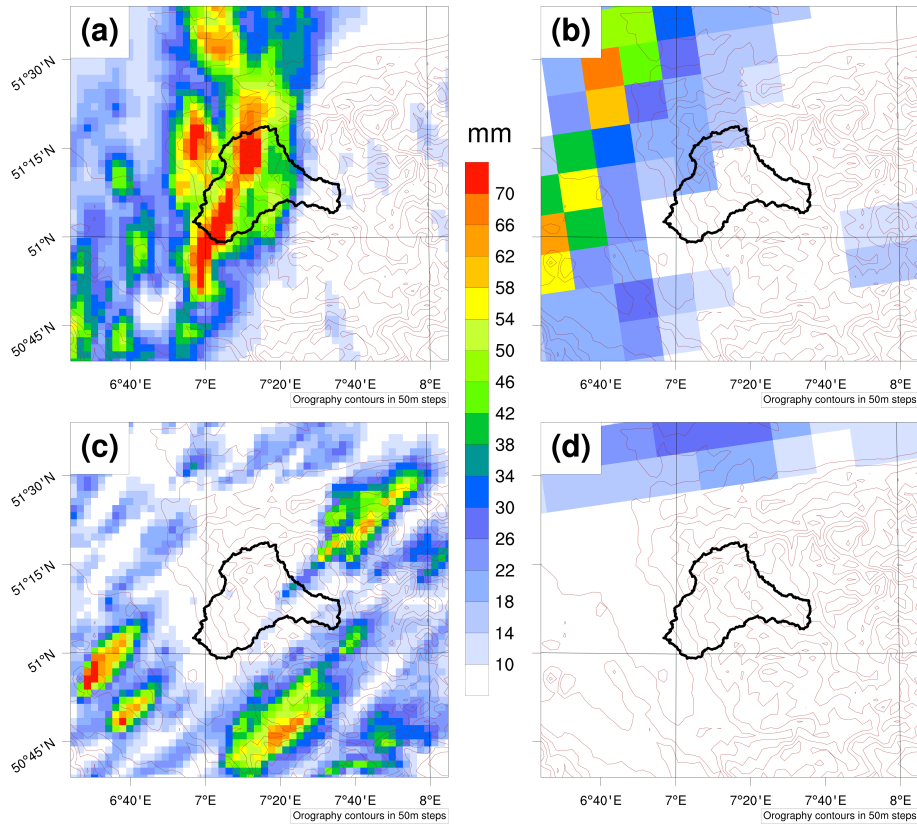
Figure 6. Illustrative modelled PEDs. (a) Example summer PED downsampled to 0.02^\circ and (b) the same day in the 0.11^\circ parent model. In this example, the strongest precipitation directly strikes the catchment in the 0.02^\circ CCLM despite missing the catchment in the parent 0.11^\circ CCLM. (c) Example summer PED with highly localised intense precipitation which falls outside the catchment in the 0.02^\circ CCLM. (d) The corresponding day in the 0.11^\circ CCLM.
