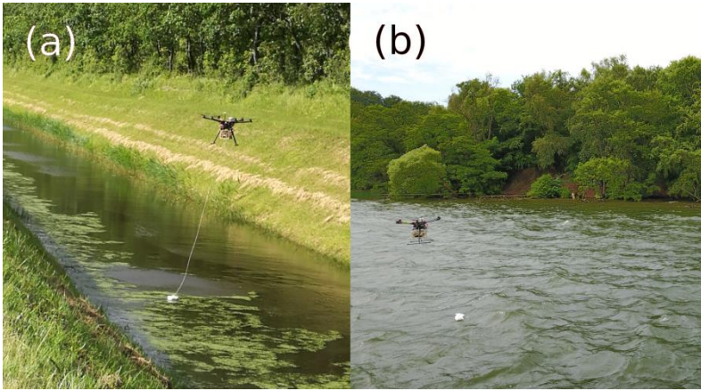
5 Figure 1. Pictures of the UAV and the tethered sonar. These pictures were retrieved in: (a) Marrebæk Kanal, Denmark. (b) Furesø lake, Sjælland, Denmark. In (b) the drone was flown a few hundreds of meters from the shore and the picture was retrieved using an optical camera onboard an auxiliary UAV (DJI Mavic Pro).
