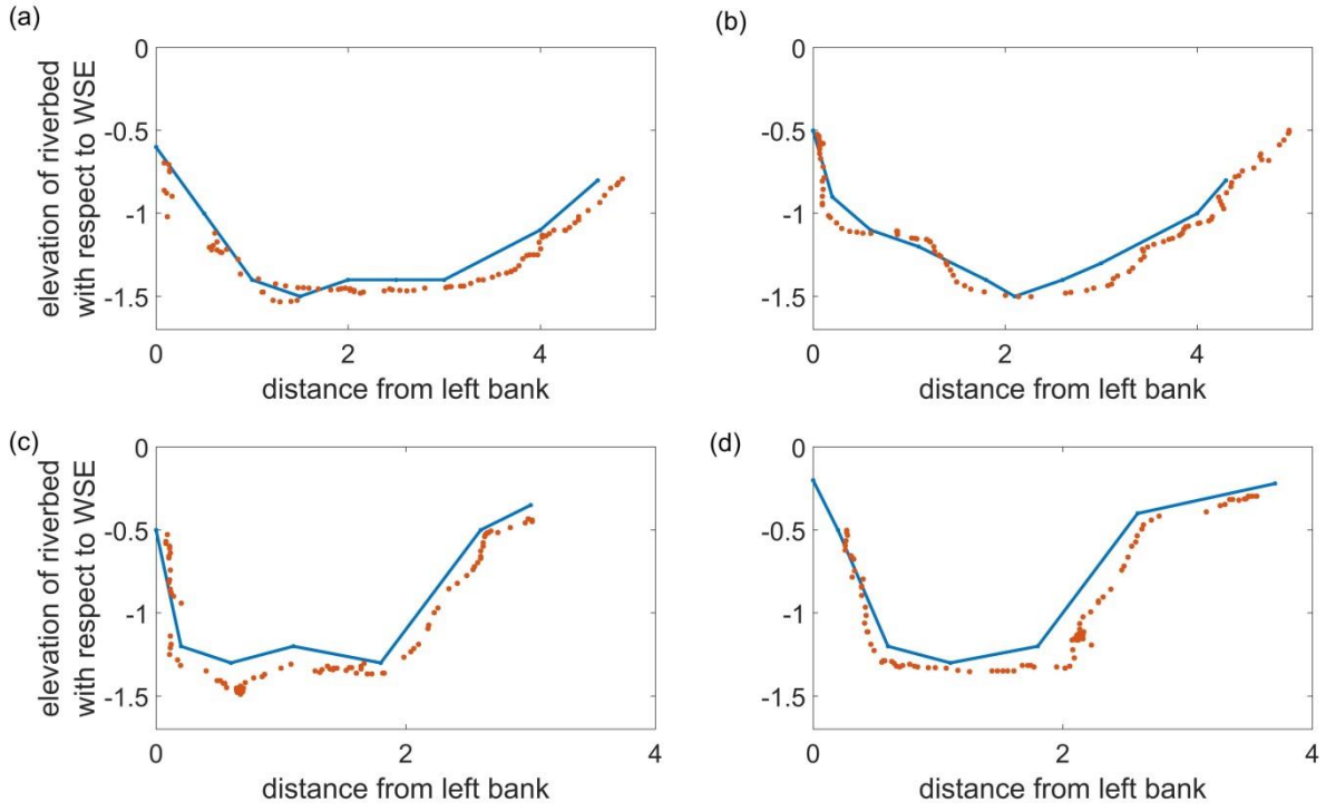
Figure 10. River cross sections retrieved at different locations along Marrebæk Kanal. The y-axis shows the difference between riverbed elevation and WSE (opposite sign of water depth). Red points are retrieved with UAV-borne observations, blue lines are the ground truth observations. The latitude and longitude coordinates of the left bank of the river cross sections are (a) 54.676300°, 11.913296° (b) 54.675507°, 11.913628° (c) 54.682117°, 11.911957° (d) 54.681779°, 11.910723° (WGS84 coordinates).
