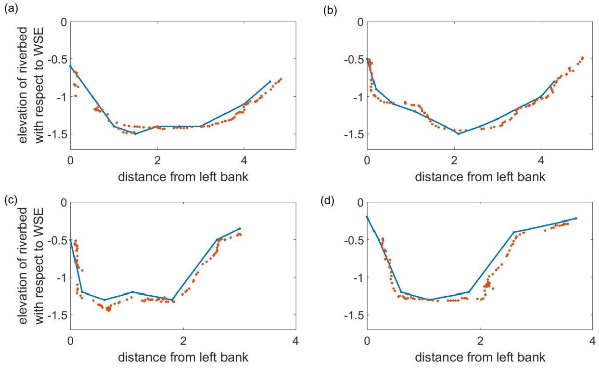
Figure 11. River cross sections observations retrieved from Marrebæk Kanal at the locations shown in Figure 10 after correction of the Deeper sonar observations. Red points are retrieved with UAV-borne observations, blue lines are the ground truth observations.
