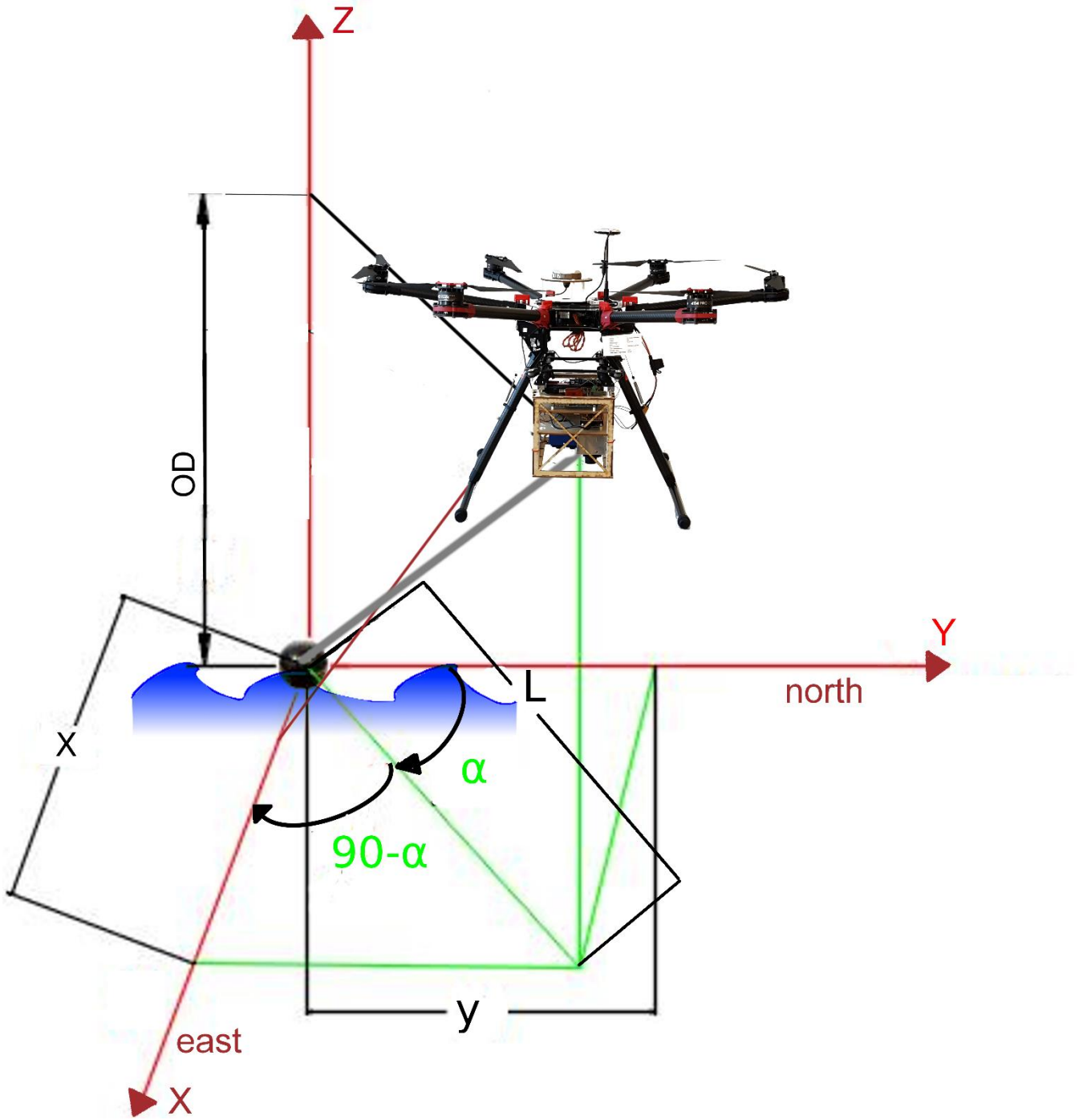
Figure 3. Sonar is the center of the reference system X, Y, Z. The horizontal displacement between the sonar and the drone is computed along the X and Y directions, the vertical displacement along the Z axis (Object Distance - OD). The angle \alpha is the azimuth, i.e. the angle between the Y-axis pointing north and the vector between the drone and the sonar, projected onto the horizontal plane (in green). The azimuth angle is measured clockwise from north (i.e. \alpha is positive in the figure).
