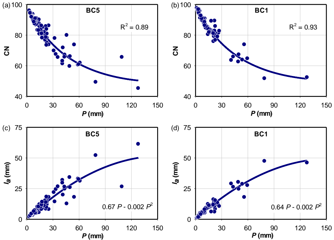
Figure 2. Variation of CN ( \lambda = 0.2 ) with P in watersheds (a) BC5, (b) BC1, near Greenville, SC. Variation of I_a with P in (c) BC5, (d) BC1 (see Santikari (2017) or Santikari and Murdoch (2018) for study area description). Best fit curves for I_a are quadratic functions of P with zero intercept. Corresponding best fit curves for CN were derived from those of I_a using eqs. (3) and (5).
