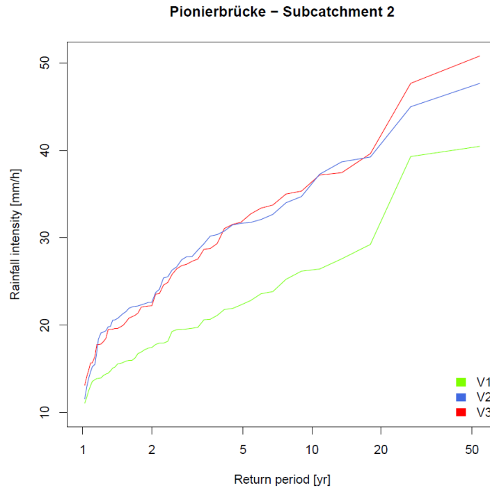
5 | Fig. 57. Annual rainfall extremes of the areal rainfall intensities for subcatchment 2 in Pionierbrücke (for one realization, based on n=53 annual extreme values from 01.11.1950-31.10.2003).
