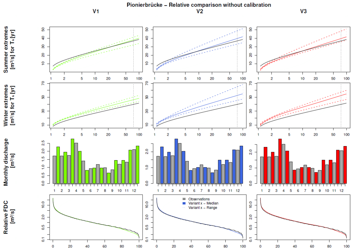
Fig. 157. Runoff simulation results with WaSiM without calibration for Pionierbrücke, validation period
