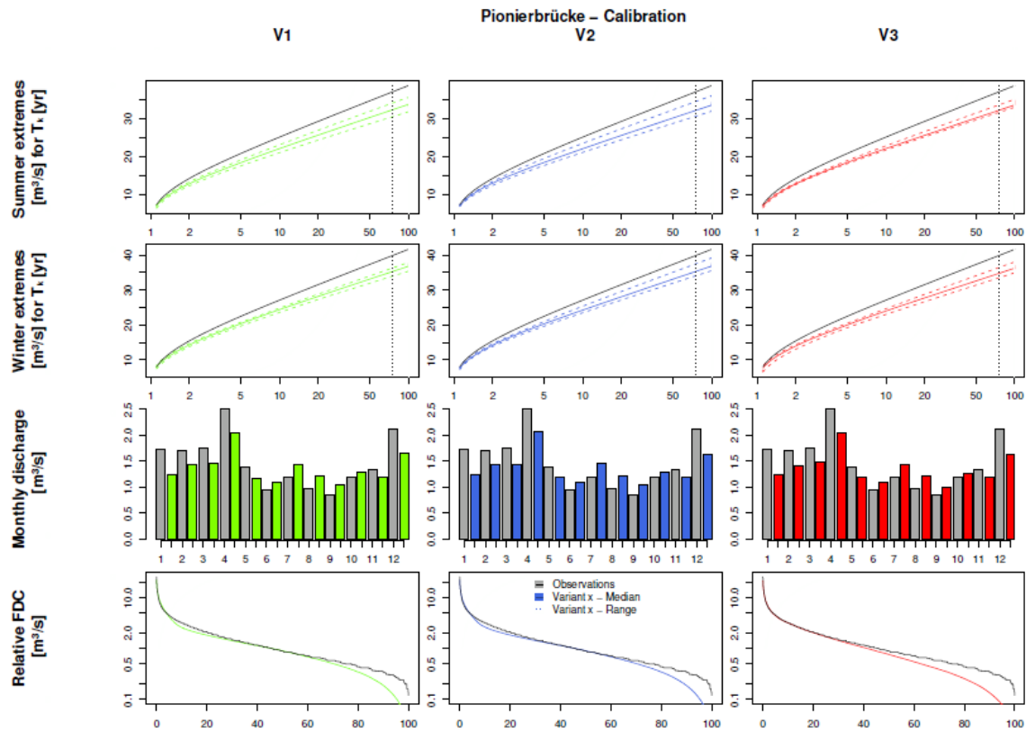
5 | Fig. 810. Runoff simulation results with HBV for Pionierbrücke, calibration period
