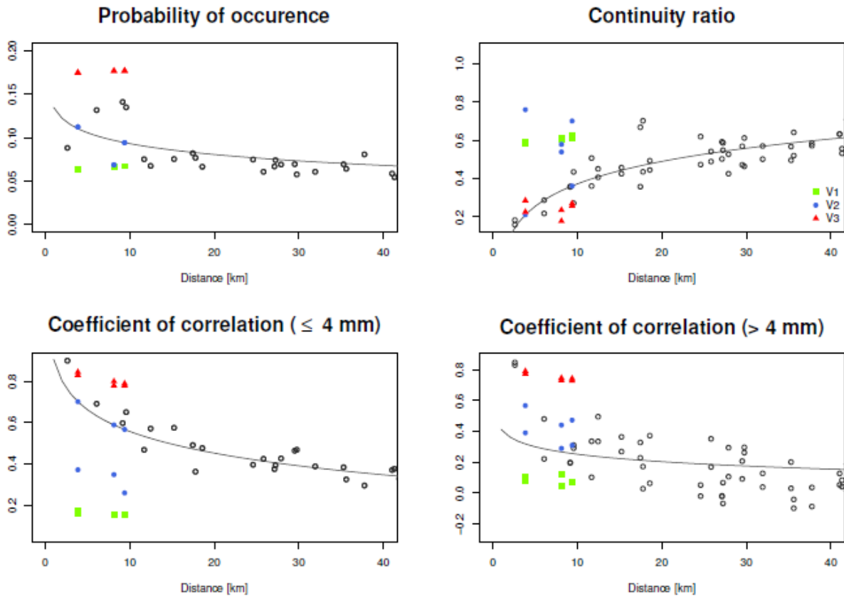
Fig. 45. Bivariate spatial rainfall characteristics of V1, V2 and V3 in comparison to observations for the catchment Pionierbrücke (for one realization, black circles represent observations - for details the reader is referred to Müller and Haberlandt (2015) ).
