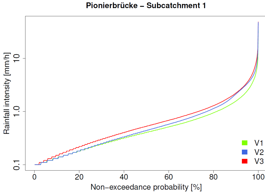
Fig. 6. Non-exceedance curve of areal rainfall intensities for V1, V2 and V3 for one subcatchment of Pionierbrücke (for one realization)
