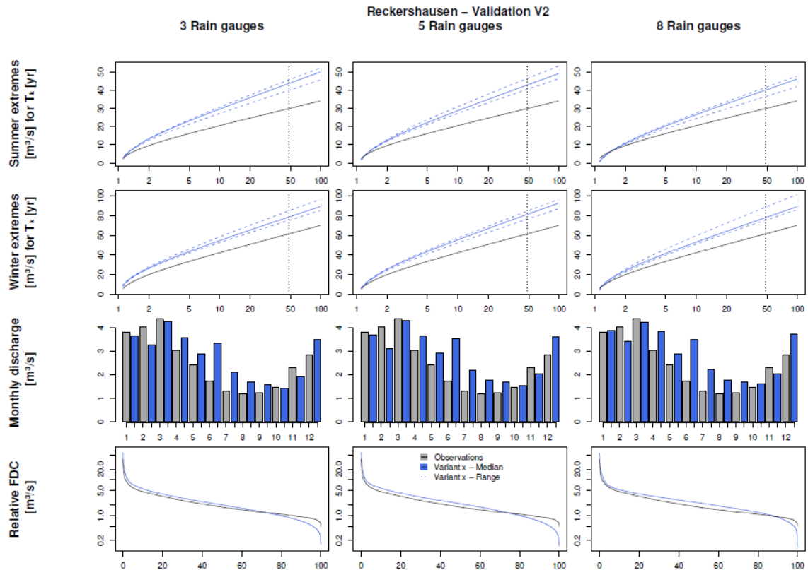
Fig. 124. Runoff simulation results for V2 with 3, 5 and 8 rain gauges with HBV for Reckershausen, validation period
