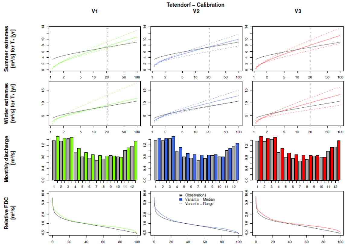
Fig. 9.41. Runoff simulation results with HBV for Tetendorf, calibration period
