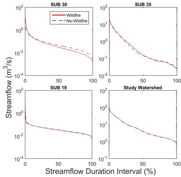
Figure 9: Flow-duration curves for select sub-basin-watersheds as well as the entire study watershed. Subbasin-Subwatershed area and percentage of burned area for subbasins-subwatersheds 30; 35; 19 and study watersheds are: 11 km 2 , 79%; 269 km 2 , 16%; 90 km 2 , 10% and 2,732 km 2 , 14% respectively.
