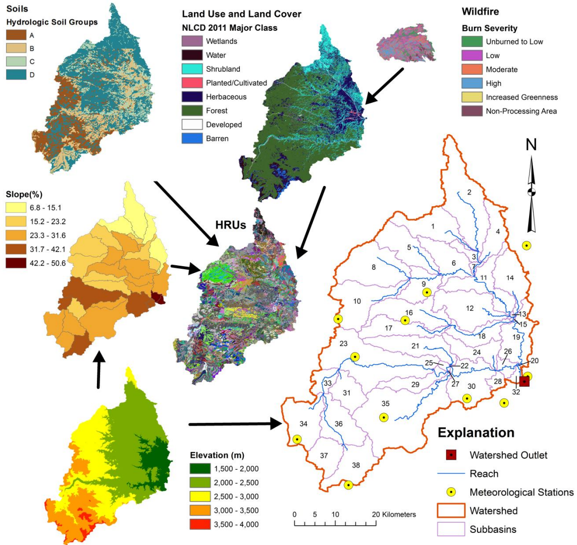
Figure 2: Initial SWAT model development summary. Outer figures show terrain, LULC, wildfire burn severity, soils, and HRUs. Main figure (lower right) includes labeled sub-basins, subwatersheds, location of meteorological stations, and reach network. Note that for illustrative purposes the soils and LULC classifications shown are simplified versions of the actual classifications used to establish HRUs.
