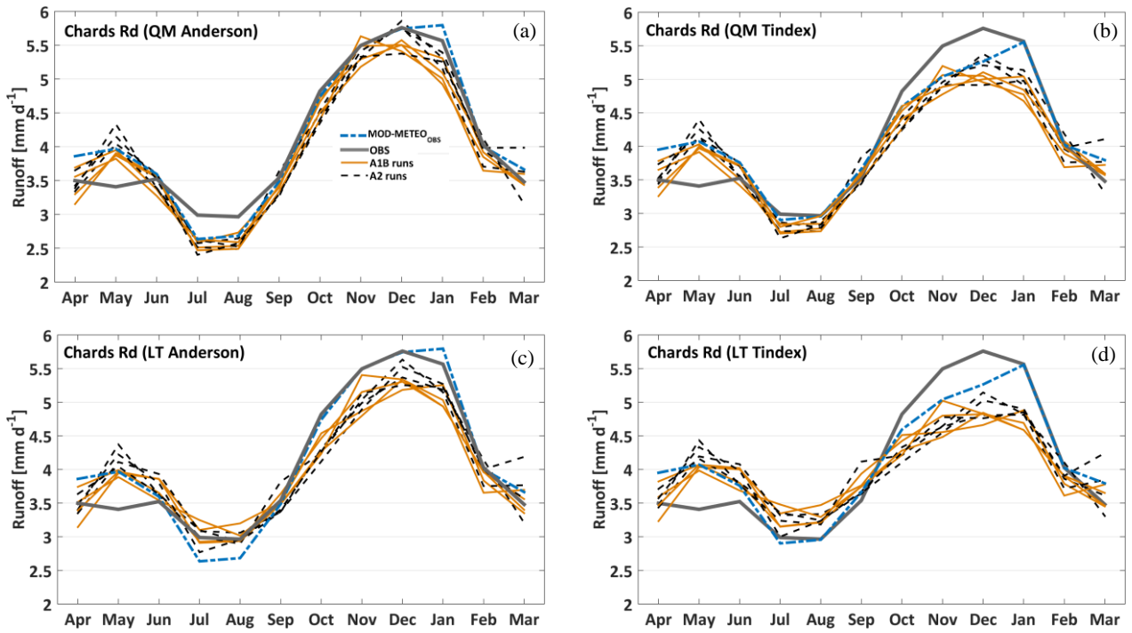
Figure 4 RCM driven mean daily runoff simulations for the 1/4/1992–30/3/2011 period at Chards Rd. Simulations are compared with the observed regime (grey line) and the modelled (WaSiM forced with observed meteorology) regime (blue line) for the four sub-ensembles: QM-Anderson (a), QM-Tindex (b), LT-Anderson (c) and LT-Tindex (d).
