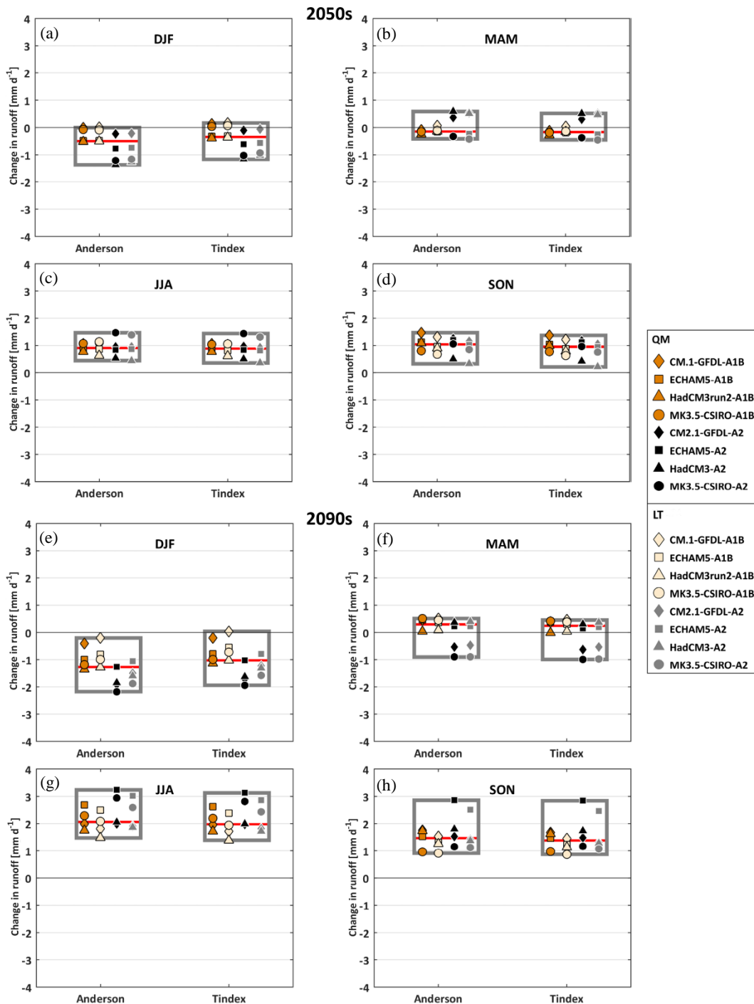
Figure 8 The uncertainty range of the seasonal runoff signal is shown for Chards Rd. Each plot contains an uncertainty box for WaSiM-Anderson and WaSiM-Tindex simulations, respectively. In each box (red line = median) the uncertainty range is broken down into the two emission scenarios and the two bias correction methods (LT and QM). The results are shown for the 2050s (a-d) and the 2090s (e-h).
