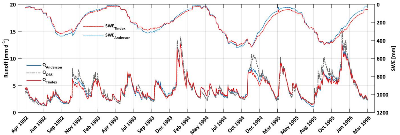
Figure 3 Observed and modelled (WaSiM-Anderson and WaSiM-Tindex) daily runoff at Chards Rd during the first four years of the validation period (1992-1996). The snow water equivalent (SWE) is also plotted for the Tindex and Anderson simulations, respectively.
