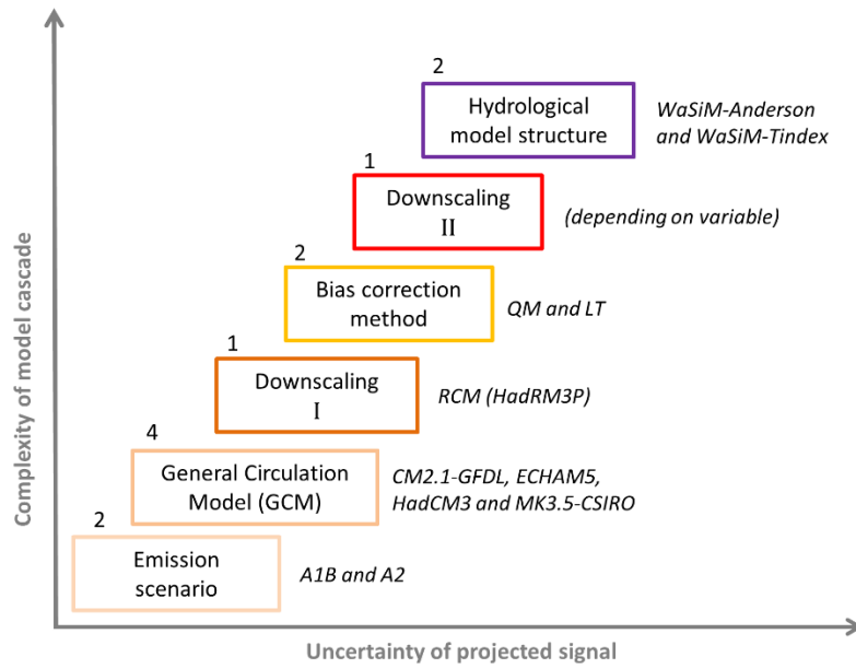
Figure 2 The model cascade is depicted with the individual members of each component listed on the right. Permuting the members of all components results in a total of 32 hydrological projections.
