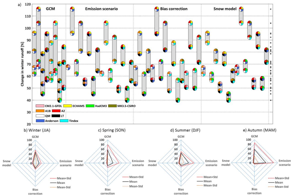
5 Figure 10 (a) Uncertainty by varied model component exemplified for winter and relative contribution to the overall uncertainty for the simulated changes in seasonal runoff for (b) winter, (c) spring, (d) summer and (e) autumn. Based on the permutations for each season the radar charts show the mean contributions [%] of the four model components to the overall uncertainty as well as the standard deviations [%].
