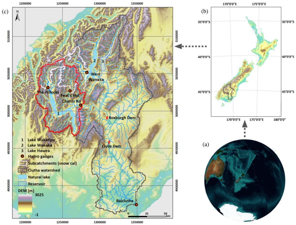
Figure 1 Maps showing (a) the location of New Zealand in the Southern Ocean, (b) New Zealand with the Clutha catchment located in the lower South Island and (c) the Clutha catchment with some of the key sites (including natural storages and water management).
