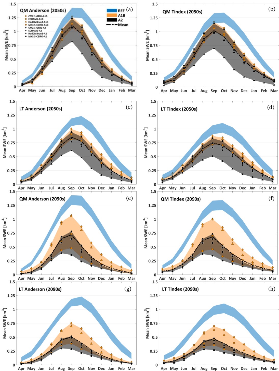
Figure 9 The monthly SWE storage ( \text{km}^3 ) is depicted for the 2050s period (a-d) and the 2090s period (e-h). The results are shown for the four sub-ensembles QM-Anderson, QM-Tindex, LT-Anderson and LT-Tindex, respectively. In each plot the individual
