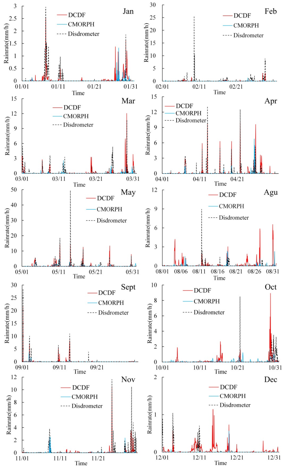
Fig. 6. Time series of disdrometer data, original CMORPH and DCDF precipitation at hourly scale in 2014
