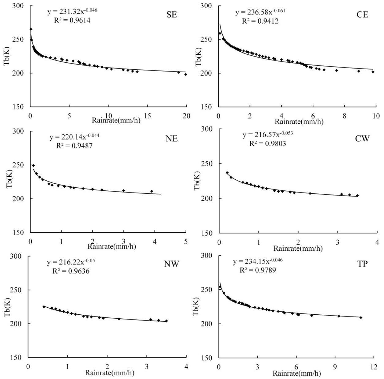
Fig. 4. Examples of fitting of precipitation rate and Tb for each region in China during 20140709-20140718 for subregion SE (115°35'E, 27°28'N), subregion CE (115°39'E, 36°14'N), subregion NE (124°20'E, 51°42'N), subregion CW (101°38'E, 37°31'N), subregion NW (85°43'E, 46°47'N), and subregion TP (91°06'E, 30°29'N).
