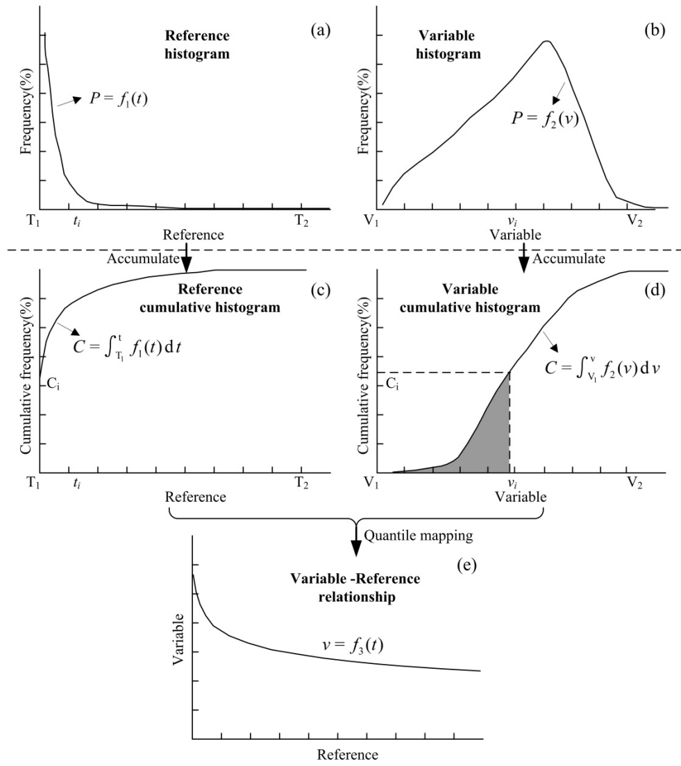
Fig. 2. Schematic of the cumulative distribution of frequency (CDF) matching method
