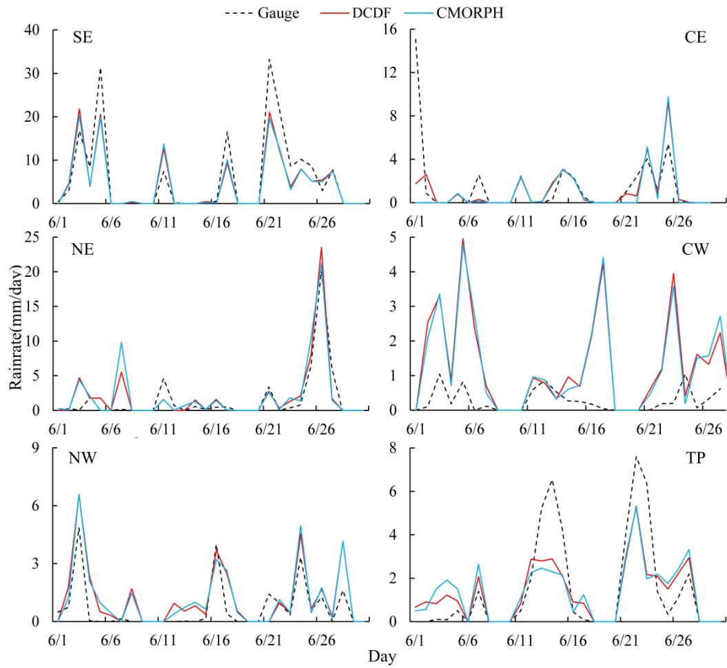
Fig. 7. Time series of the average precipitation of each region derived from gauge, DCDF and CMORPH at the daily scale in June 2014.
