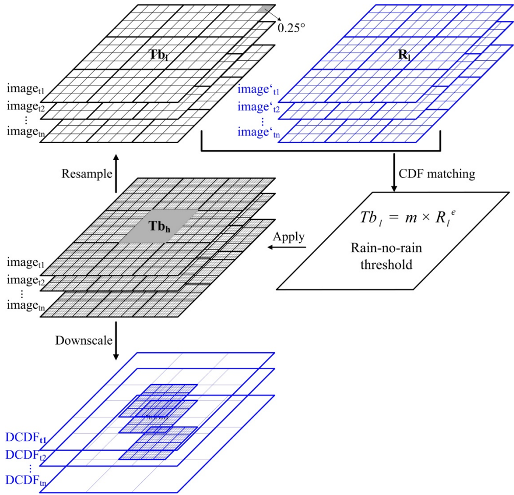
Fig. 3. Schematic of the CDF-based downscaling method (DCDF) using CMORPH and FY2-E Tb in this study. R represents precipitation rate.
