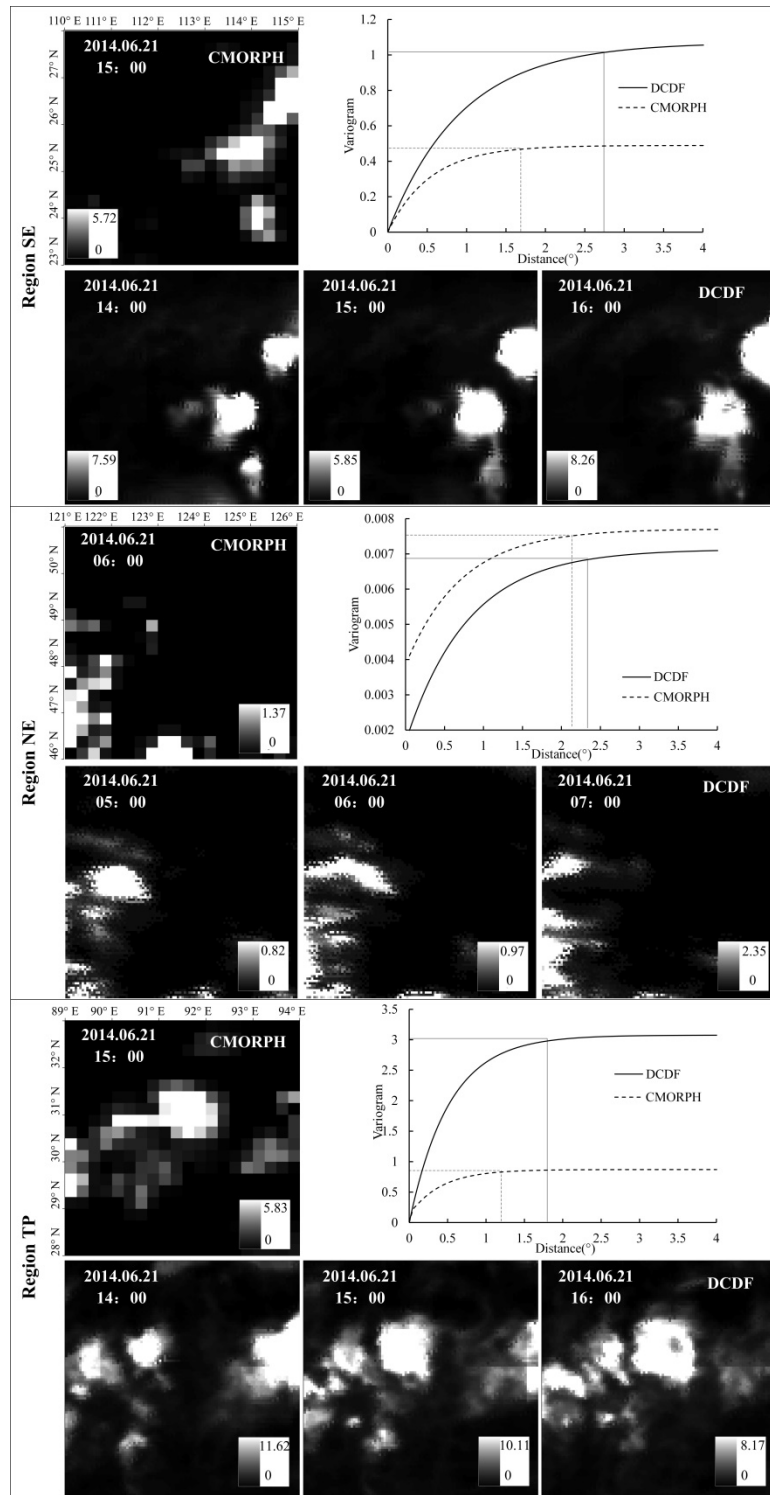
Fig. 5. CMORPH precipitation estimates at a nominal resolution of 0.25^\circ and DCDF precipitation maps at a 0.05^\circ resolution for regions SE, NE and TP
