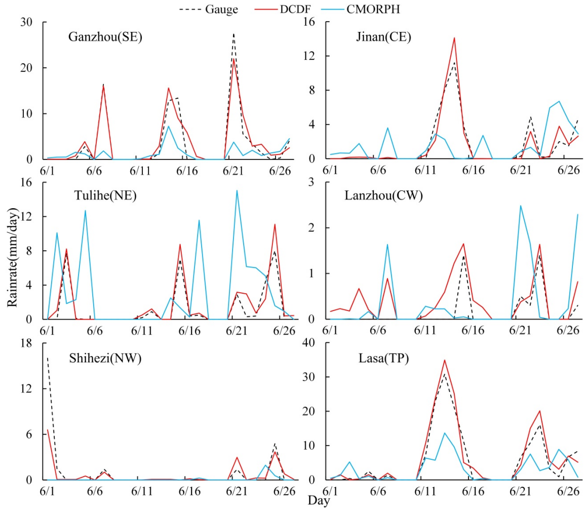
Fig. 8. Time series of rain gauge data, original CMORPH and DCDF precipitation for each randomly selected gauge. Ganzhou station (SE), 113.1667°E, 25.8667°N; Jinan station (CE), 117.05°E, 36.6°N; Tulihe station (NE), 121.6833°E, 50.4833°N; Lanzhou station (CW), 103.8833°E, 36.05°N; (e) Shihezi station (NW), 86.05°E, 44.3167°N; (f) Lasa station (TP), 91.1333°E, 29.6667°N.
