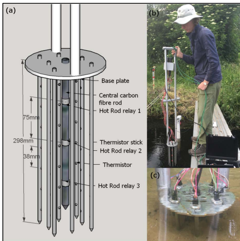
Figure 1: (a) Detailed design of the active HPS Hot Rod with 3 heating elements on the central carbon fibre rod surrounded by 56 temperature sensors at two distances from the central heat source (28 and 47 mm). (b) and (c) Installation of the Hot Rod in a small stream characterised by shallow bedforms.
