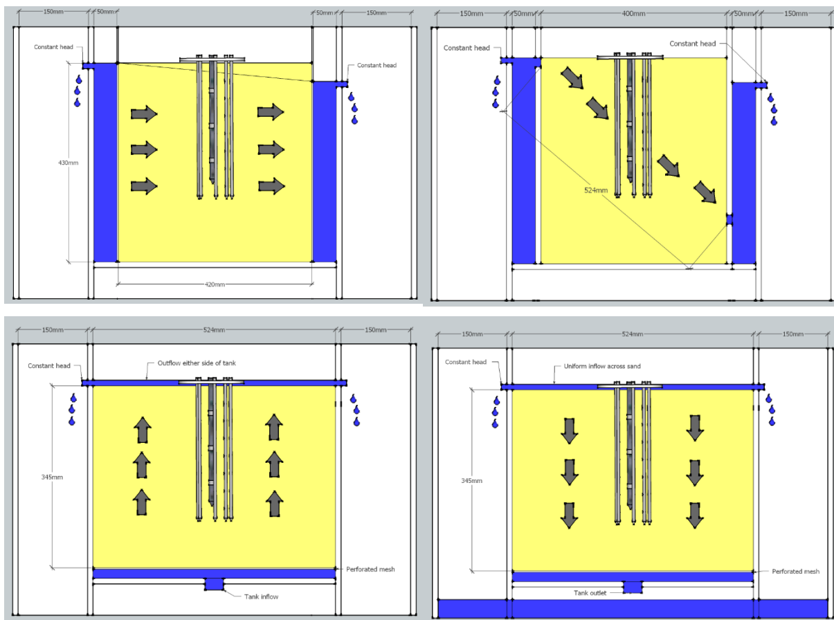
5 Figure 3: Laboratory sand tank dimensions for each of the flow scenarios (a) horizontal flow, (b) diagonal flow, (c) upward flow, and (d) downward flow.
