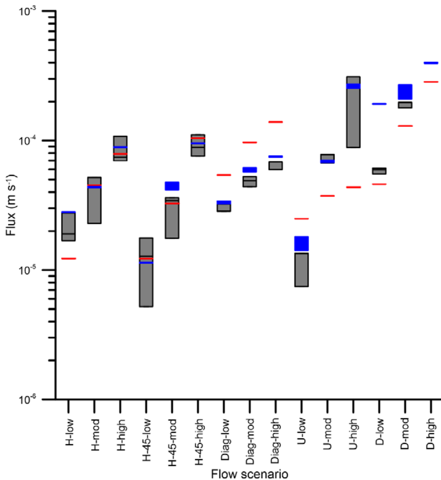
5 Figure 6: Fluxes of the different flow scenarios and different flow intensities calculated based on different heat injection depth of the HPS (grey bars) compared to fluxes determined based on Darcys law (hydraulic gradient and hydraulic conductivity- red dashes) and the measured discharge from the tank using an ultrasonic flow meter (blue dashes).
