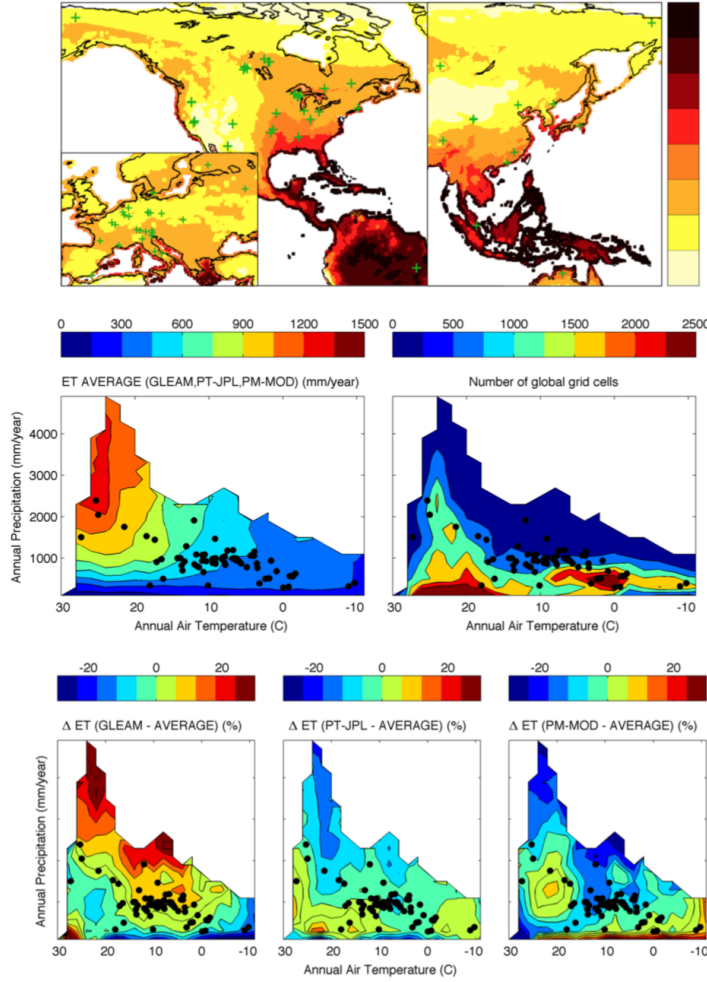
Figure 1. Distribution of tower sites used in the study. Top: geographical location (green crosses) on a map of the multi-annual simple average of the three ET products (GLEAM, PT-JPL, and PM-MOD). Middle: distribution of the averaged multi-annual ET (left), and the number of global grid cells (right), as function of the annual air temperature and precipitation, together with the location of the tower sites in this space (black dots). Bottom: the relative GLEAM (left), PT-JPL (middle), and PM-MOD (right) ET differences normalized by the multi-annual simple average of the three ET products.
