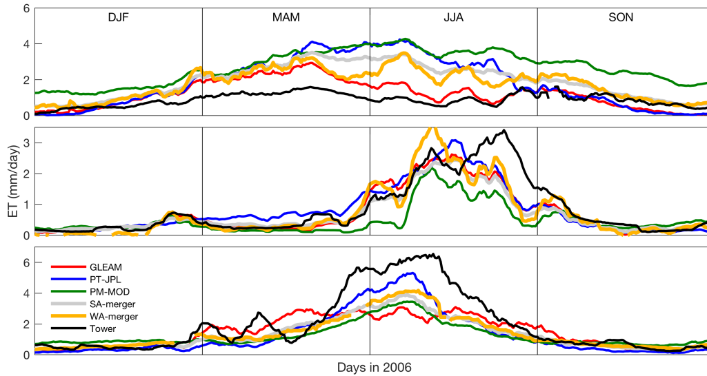
Figure 6. 2006 time series of the different ET products and the sites shown in Fig. 5: FR-Pue (top), US-SRM (middle), and US-Ne1 (bottom). The daily values are time smoothed using a 10-day moving averaged window to better display the more persistent temporal features.
