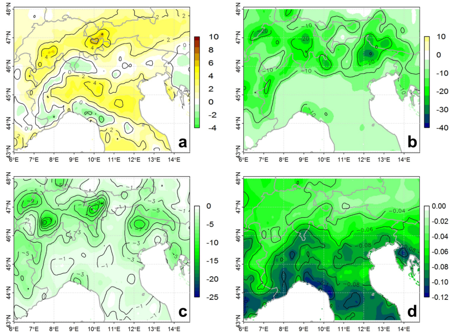
Figure 6. Hydrologic budget components: differences between FC_{A2} and RC (i.e., FC_{A2} - RC ) of the mean values of a) ET (in mm), b) PR (in mm), c) SR (in mm) and d) surface SM (in m^3 m^{-3} ). The mean is calculated over the month of July.
