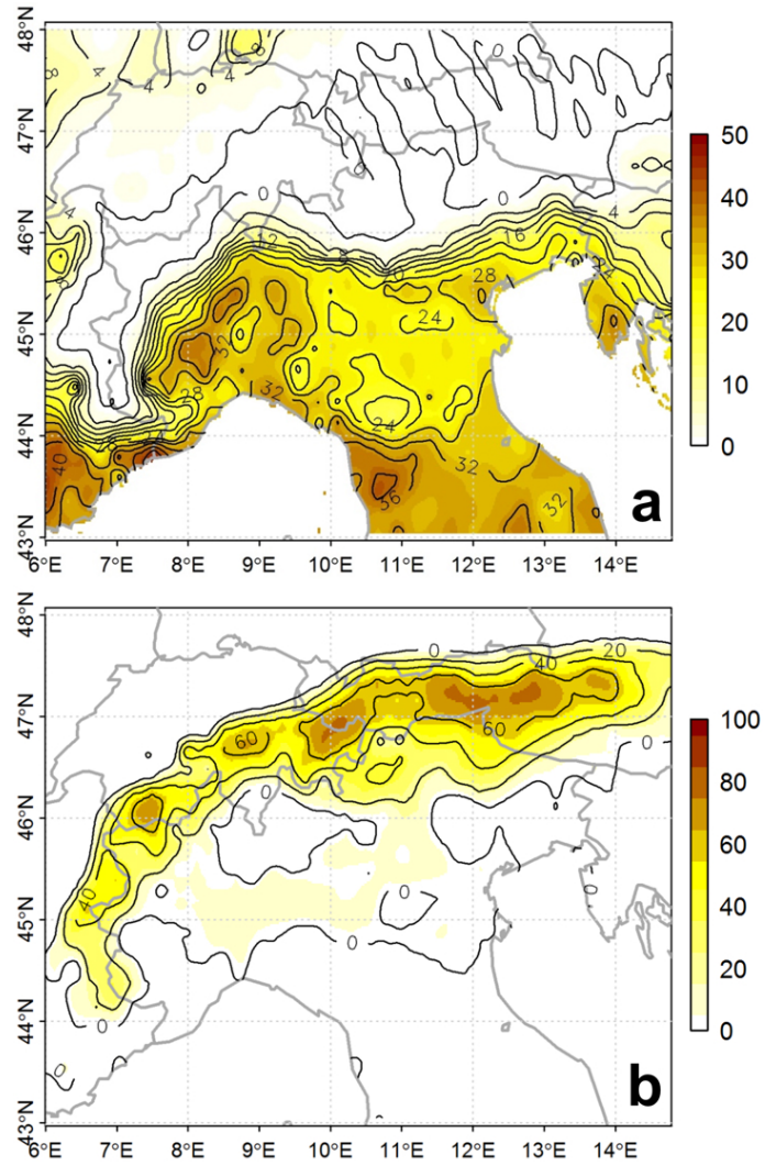
Figure 7. The anomalies in number of a) dry days and b) wet days in FC A2 .
