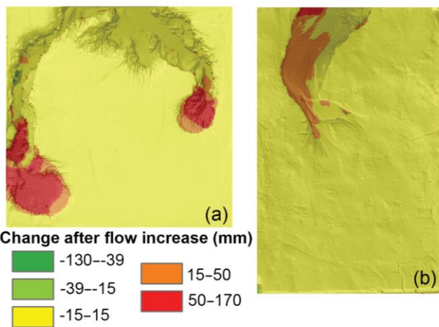
Figure 6: These differenced DEMs show how changes in flow impact channel width. In the fine-grained runs (A) the width changed in the newly formed channel, while in the sand runs (B) the channel width was altered along the entire channel length. Flow is bottom to top in both images.
