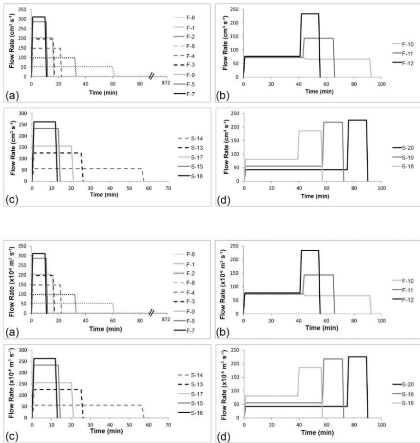
Figure 2: These hydrographs show the range of flow rates tested. Each set of curves is for a separate set of experimental runs. A) 190 litres of water over the fine-grained-substrate. B) 380 litres of water over the fine-grained substrate. C) 190 litres of water over the sand substrate. D) 380 litres of water over the sand substrate.
