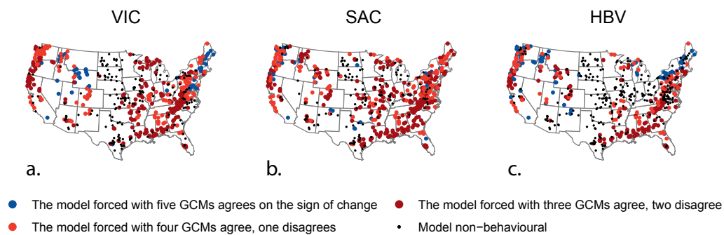
Figure A3. The agreement on the sign of the ensemble mean change in mean annual runoff in the output from the same hydrologic model forced with five different climate models. a) Agreement when the Variable Infiltration Capacity Model (VIC) is forced with data from five different GCMs. b) Agreement when Sacramento Soil Moisture Accounting Model (SAC) is forced with data from five different climate models. c) Agreement when Hydrologiska Byråns Vattenbalansavdelning Model (HBV) is forced with data from five different GCMs.
