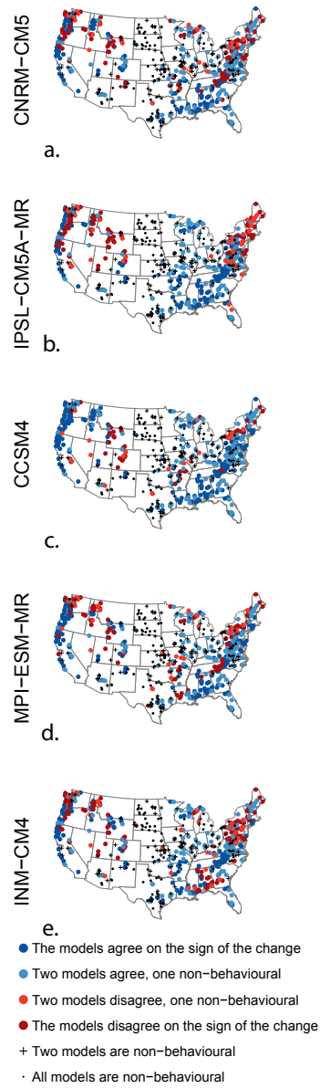
Figure A2. The agreement among the three hydrologic models on the sign of the ensemble mean change in mean annual runoff, forced with five different climate models. a) The three hydrologic models are forced with CNRM-CM5 data. b) The three hydrologic models are forced with IPSL-CM5A-MR data. c) The three hydrologic models are forced with CCSM4 data. d) The three hydrologic models are forced with MPI-ESM-MR data. e) The three hydrologic models are forced with INM-CM4 data.
