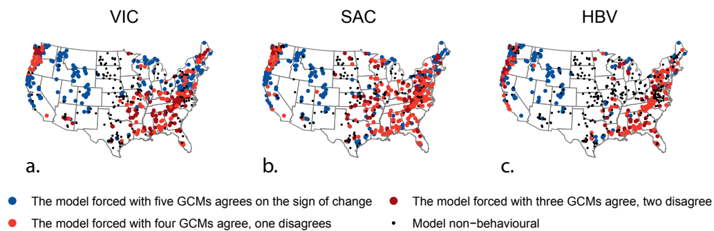
Figure B3. The agreement on the sign of the ensemble mean change in discharge timing in the output from the same hydrologic model forced with five different climate models. a) Agreement when Variable Infiltration Capacity Model (VIC) is forced with data from five different GCMs. b) Agreement when Sacramento Soil Moisture Accounting Model (SAC) is forced with data from five different climate models. c) Agreement when Hydrologiska Byråns Vattenbalansavdelning Model (HBV) is forced with data from five different GCMs.
