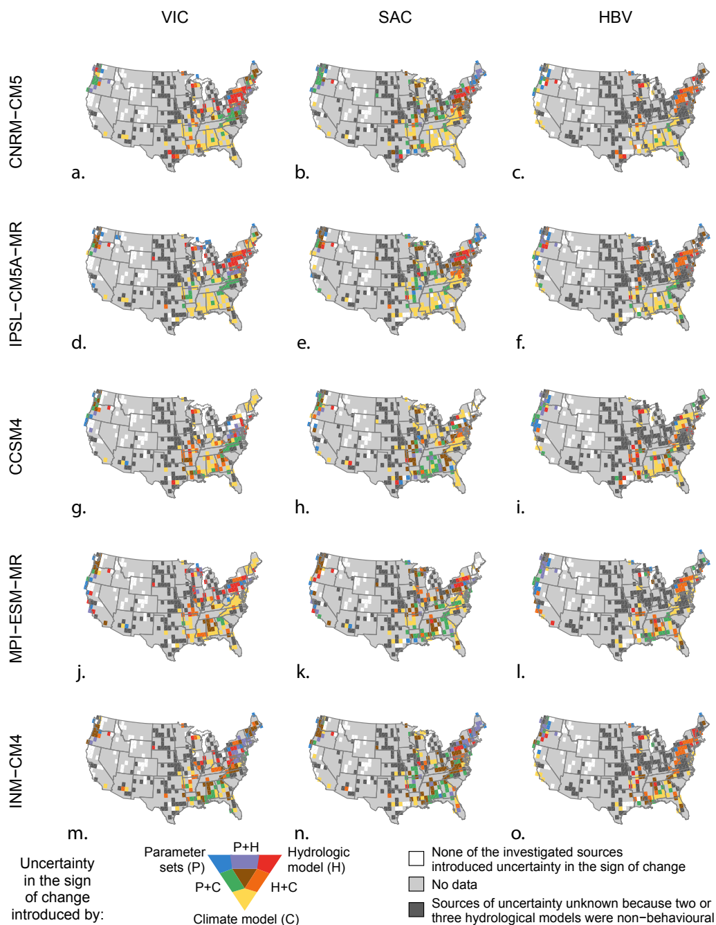
Figure B4. Distribution of the combined investigated sources of uncertainty for the discharge timing. Spatial coverage is obtained by determining a grid-based maximum likelihood. a) Variable Infiltration Capacity Model (VIC) was used as reference when climate model uncertainty was tested, CNRM-CM5 was used as reference when the hydrologic models were tested. b) Sacramento Soil Moisture Accounting Model (SAC) and CNRM-CM5 as reference options. c) Hydrologiska Byråns Vattenbalansavdelning Model (HBV) and CNRM-CM5 as reference options. d) VIC and IPSL-CM5A-MR as reference options. e) SAC and IPSL-CM5A-MR as reference options. f) HBV and IPSL-CM5A-MR as reference options. g) VIC and CCSM4 as reference options. h) SAC and CCSM4 as reference options. i) HBV and CCSM4 as reference options. j) VIC and MPI-ESM-MR as reference options. k) SAC and MPI-ESM-MR as reference options. l) HBV and MPI-ESM-MR as reference options. m) VIC and INM-CM4 as reference options. n) SAC and INM-CM4 as reference options. o) HBV and
