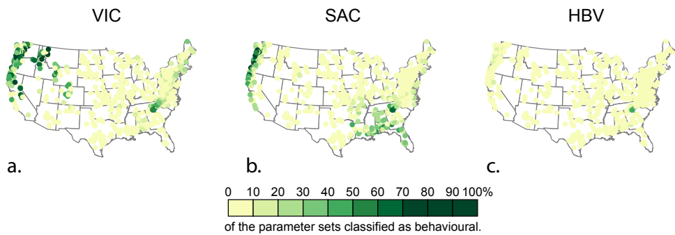
Figure C1. The percentage of parameter sets that have been classified as behavioural based on the Kling-Gupta criterion. a) for the Variable Infiltration Capacity Model (VIC), for a total parameter sample of 1800. b) for the Sacramento Soil Moisture Accounting Model (SAC), with a total parameter sample of 1900. c) for the Hydrologiska Byråns Vattenbalansavdelning Model (HBV) with a total parameter sample of 1600.
