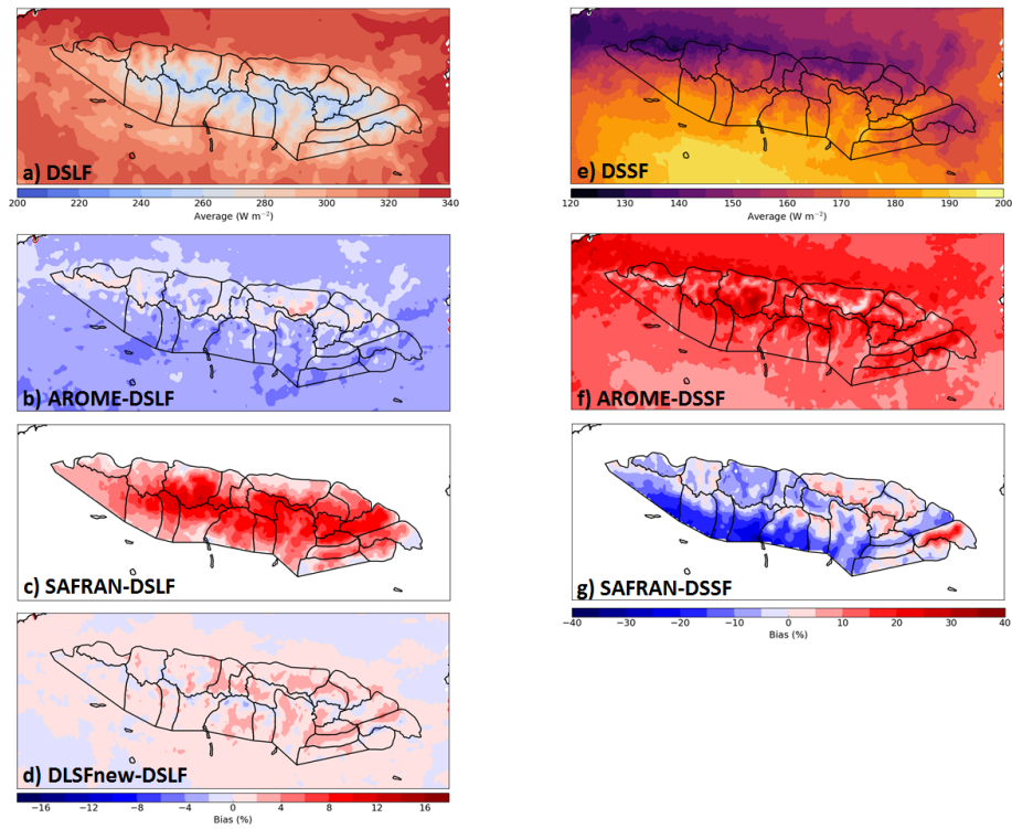
Figure 6. a) Average of the DSLF from 1 August 2010 to 31 July 2014 in the Pyrenees, and relative difference with the DSLF for: b) AROME, c) SAFRAN and d) DLSFnew. e) Average of the DSSF, and relative difference with the DSSF for: f) AROME, g) SAFRAN.
