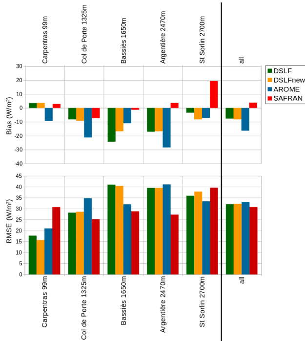
Figure 3. Bias and RMSE of LW_{\downarrow} irradiance products (DSLF in green, DSLFnew in orange, AROME in blue, SAFRAN in red) compared to each station (left) and all stations (right).
