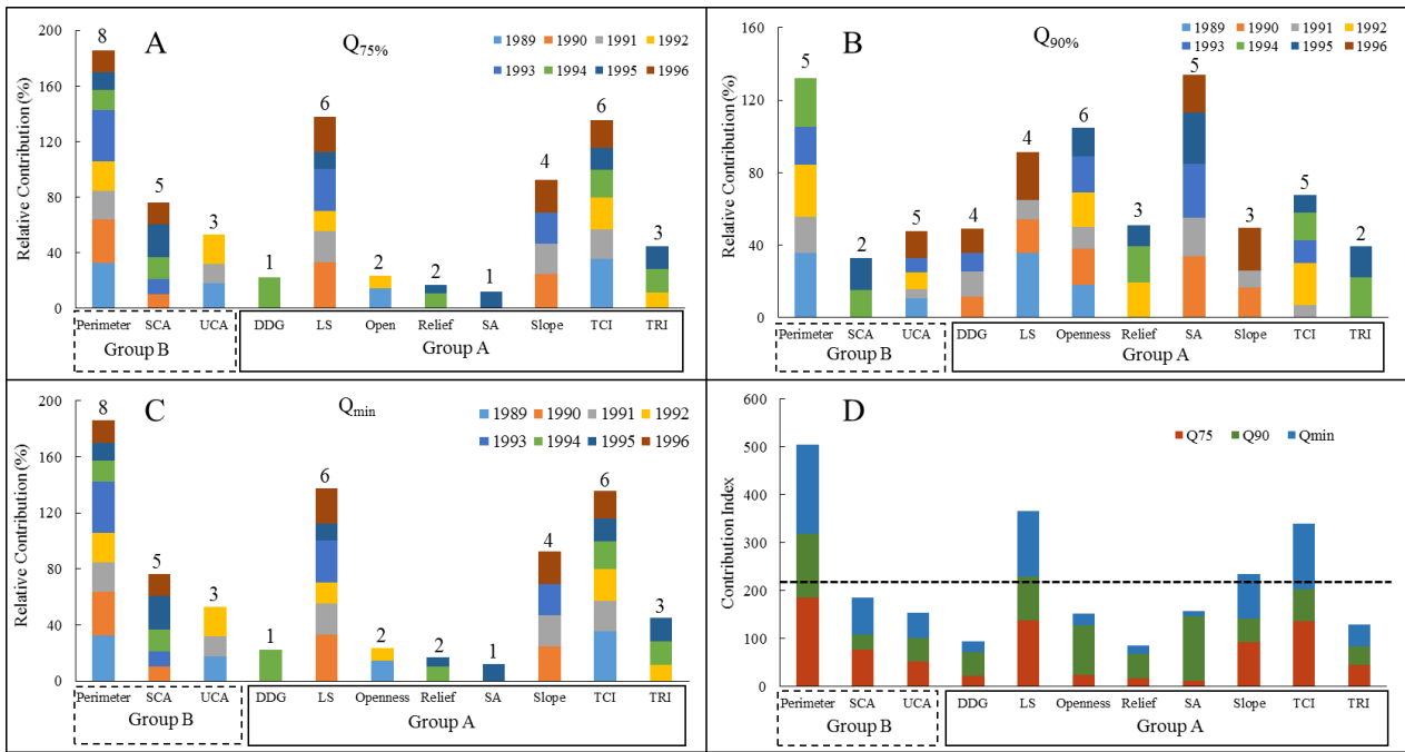
Figure 3. Relative contributions of each topographic index (TI) to Q_{75\%} (Panel A), Q_{90\%} (B), and Q_{min} (Panel C) from 1989 to 1996. Note that the numbers above the bars indicate the number of years when the given TIs were included in the regression models. Panel D: Contribution index (CI) of the 11 topographic indices (TIs) selected by factor analysis (FA) to Q_{75\%} , Q_{90\%} , and Q_{min} , respectively. Dash line is the average of the lumped CI.
