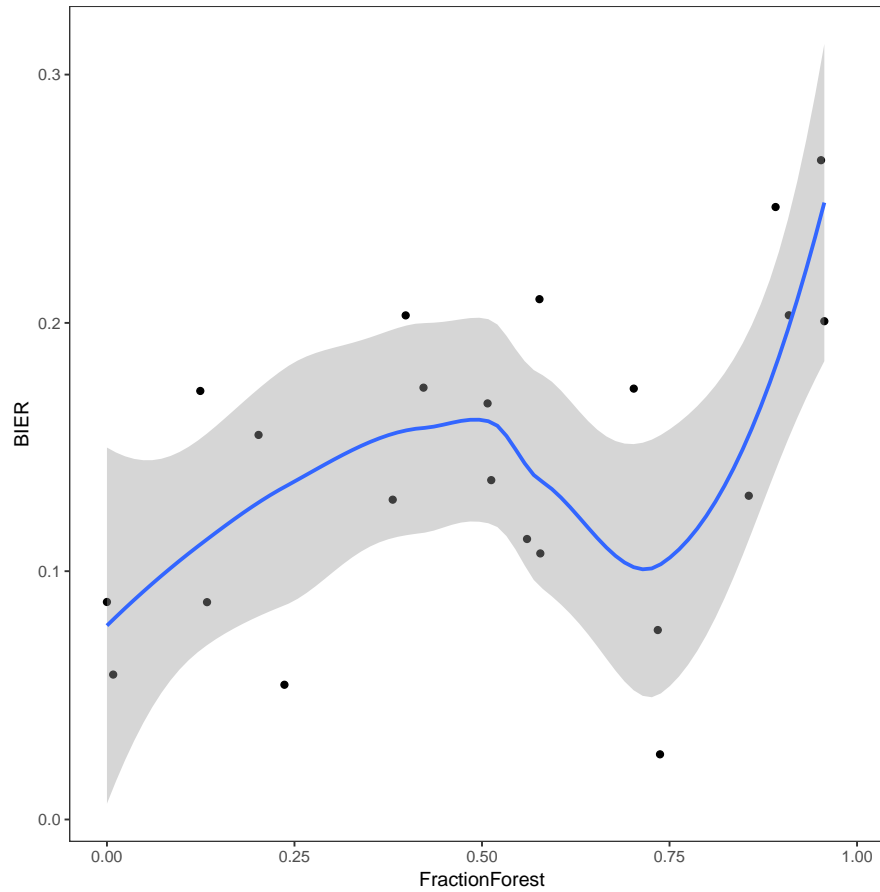
Fig. 2. Moisture recycling ratios
