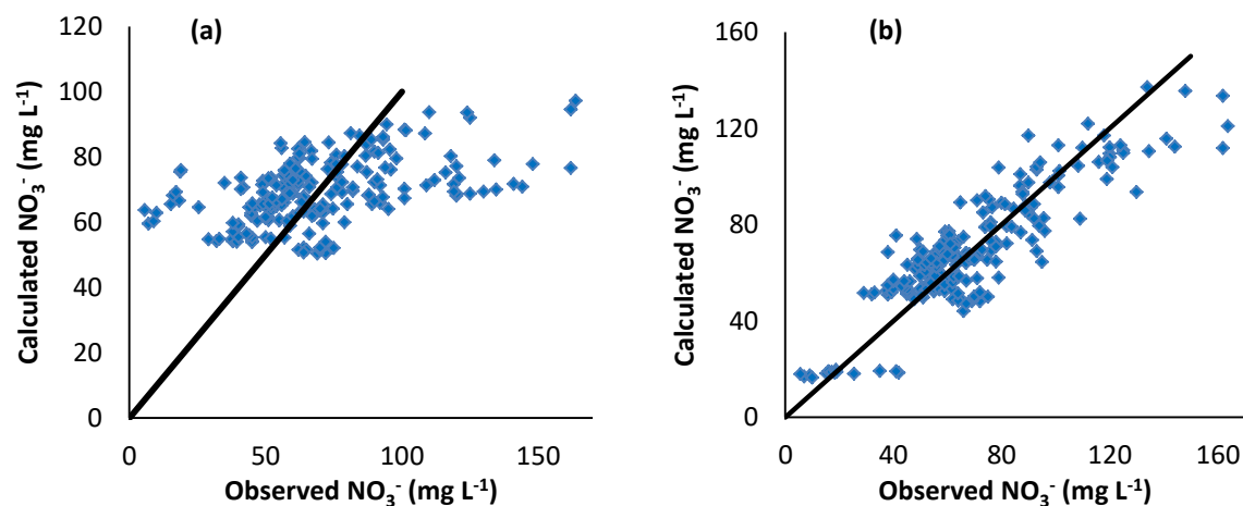
340 Figure 8: Calculated vs. observed nitrate concentrations. (a) After the first calibration stage (parameter fit). (b) After the second calibration stage (local multipliers). Black line is calculated = observed.
