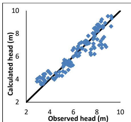
Figure 7: Calibrated flow model's calculated vs. observed heads in meters above mean sea level. Black line: calculated = observed.
