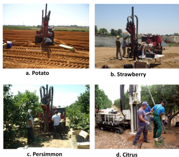
140 Fig. 3. Direct push sampling of the unsaturated zone (0–10 m below ground surface) under the different agricultural land uses. (a– c) Sampled in the current study. (d) Sampled for Kurtzman et al. (2013): the unsaturated model developed there was used here.
