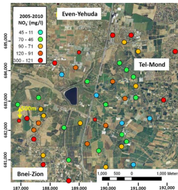
Figure 2: The agricultural area selected for modeling and 5-year average nitrate concentration in wells. Note the high spatial variability. Nitrate concentration data are from the Israel Water Authority. Coordinates system: Israeli Transverse Mercator (ITM).
