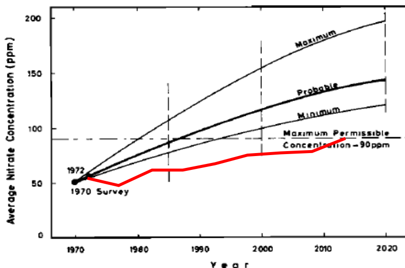
390 Figure 10: Post-audit of average nitrate concentration predicted in 1976 for another part of the Israeli coastal aquifer. All black lines and writing are original predictions from Mercado (1976). Red line is the historical average nitrate concentrations from the wells in that area that produced since 1970 (no new wells, data were obtained from the Israel Water Authority. Maximum permissible concentration of nitrate was reduced from 90 mg L -1 to 70 mg L -1 in 2001).
