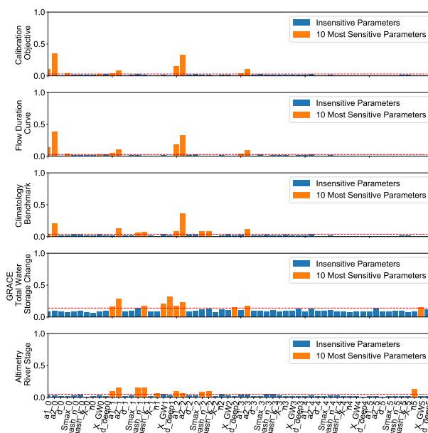
Figure 6. Sensitivity analysis of the model parameters on contributions to aggregated objective function (top) on (from second row down): FDC, climatology, GRACE and altimetry water height.
