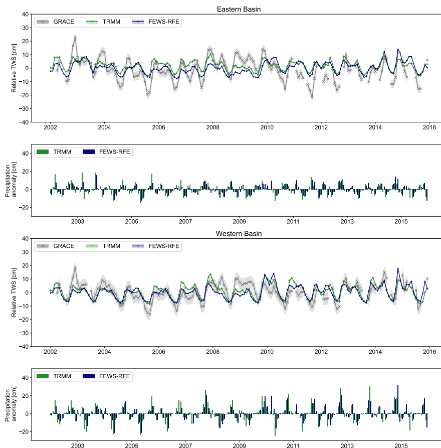
Figure 9. Total water storage change and precipitation anomaly referenced to the monthly climatology over the period of simulation for the Eastern (top) and Western (bottom) basins.
