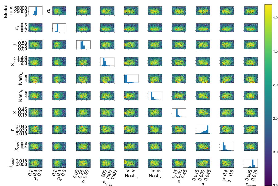
Figure 7. Parameter space post-calibration for the Ngounié calibration zone and the TRMM model. The yellow dots represent the best model runs and the red dots indicate the best parameter values. Example for TRMM model, Ngounié parameters.
