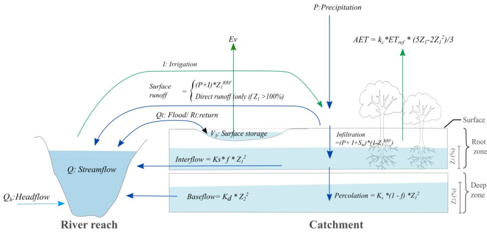
5 Figure 4. Schematic of the enhanced two-layer soil moisture model including a surface storage component.
