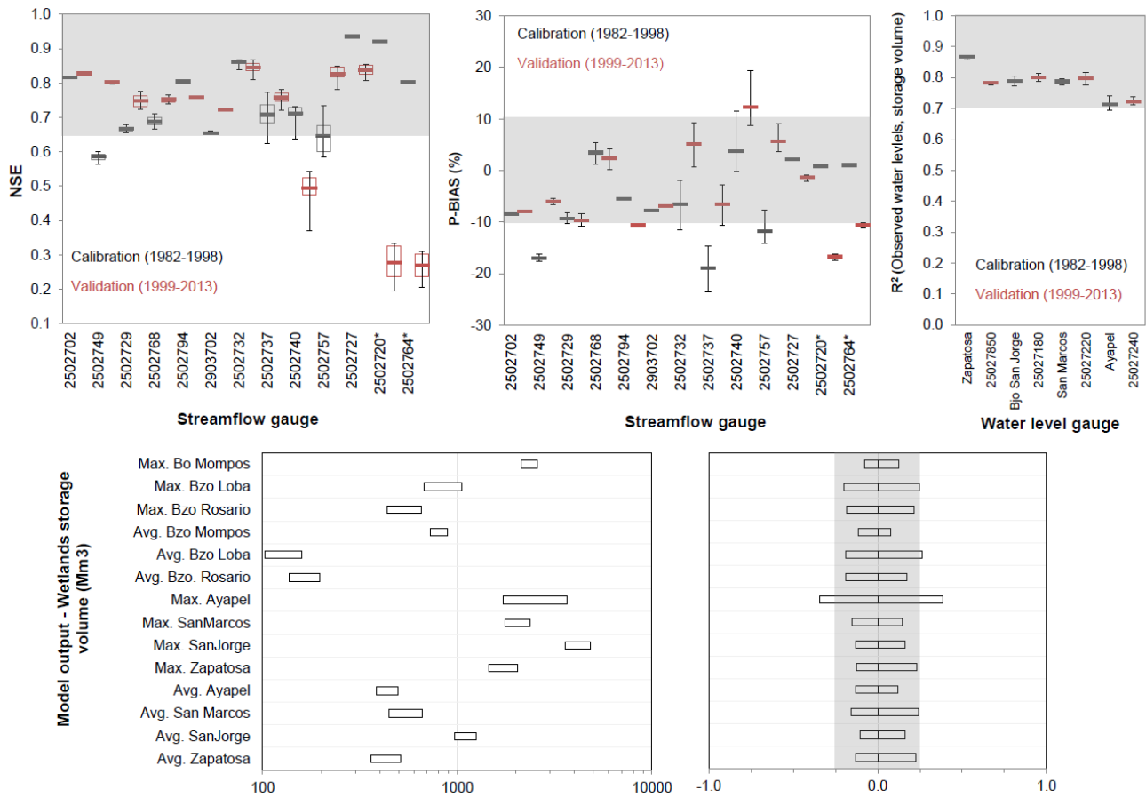
Figure 11. Comparison of the subset of models with highest performance obtained from Monte Carlo calibration: (Above) NSE and Percentile Bias of streamflow, and Correlation Coefficient of water levels and storage volumes. Acceptance ranges highlighted in grey. (Below) Model sensitivity of “good-fit models”, in terms of average and maximum volume storage in the main floodplain sub-units of the Mompós Depression.
