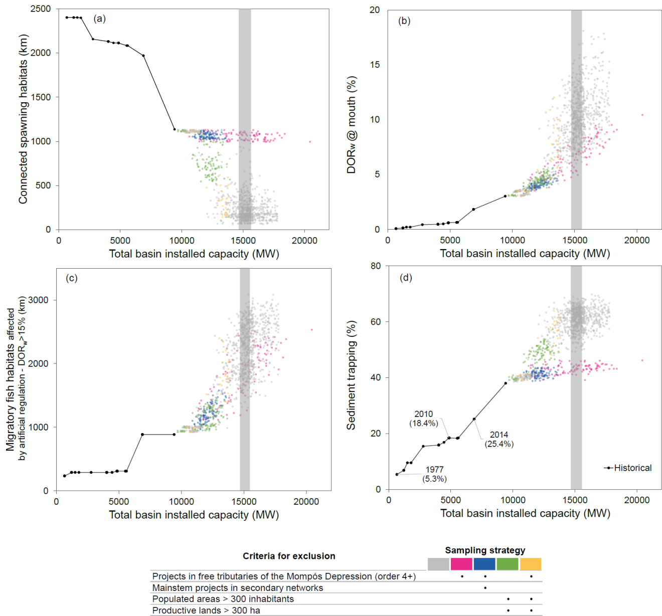
5 Figure 8. Indicators of basin-level cumulative alteration of historical hydropower development and randomly generated expansion scenarios (dots) using different sampling strategies (differentiated by color). Shaded area shows the range of expected capacity by 2050 (15 250±500 MW). (a) Longitudinally connected migratory fish spawning habitat (river length) at 400–1000 masl. (b) Cumulative streamflow regulation measured as weighted degree of regulation ( DOR_w ). (c) Migratory fish habitat (river length) affected by artificial regulation ( DOR > 15\% ) (d) Total sediment trapping in reservoirs upstream of the Mompós Depression.
