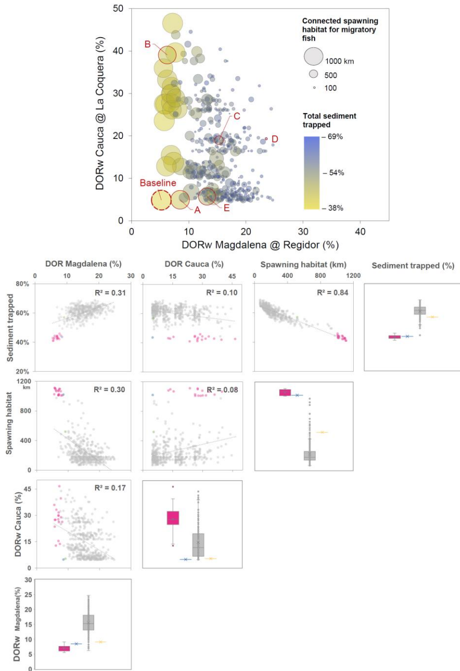
5 Figure 9. Trade-off plot for scenarios in the range of expected hydropower expansion ( 15\ 250 \pm 500 MW). (Top): X and Y axes are expected DOR_w upstream of the Mompós Depression on the Magdalena and the Cauca, respectively; bubble size represents length of connected network in the range of 400–1000 masl (spawning habitat), and color indicates the expected loss of sediment load due to reservoir trapping. Selected scenarios for detailed analyses are labeled as A, B, C, D, and E. (Bottom) 2-D plots and box-plots of individual metrics of basin-level impacts. Colors identify different sampling strategies following legend shown in Figure 8.
