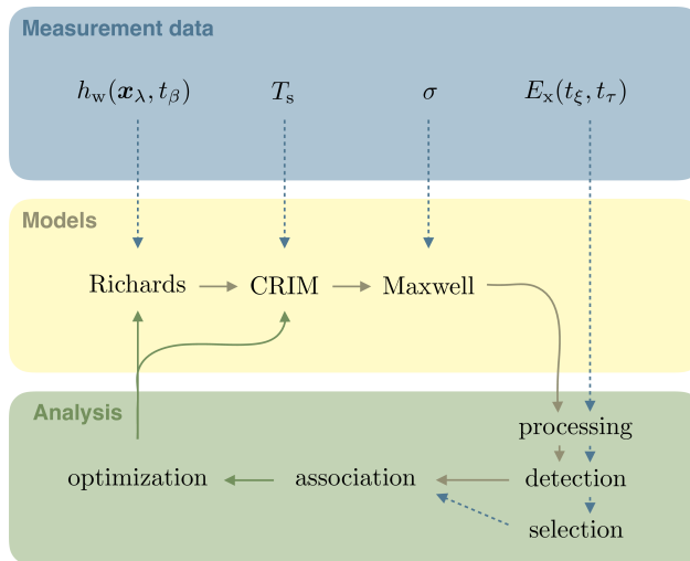
Figure 8. The general setup of the optimization is sketched with this figure. The available hydraulic potential h_w is measured at the position of the groundwater well x_\lambda times t_\beta . These measurements are used as a boundary condition for the Richards equation (Sect. 2.2.1). Estimates for the soil temperature T_s and the electrical conductivity \sigma are derived from TDR related measurements. The actual signal of the GPR system is proportional to the x -component of the electric field E_x and measured discretely at experiment time t_\xi and signal travel time t_\tau . This signal is processed (Sect. 2.3.1) and used for event detection (Sect. 2.3.2). Based on the detected events in the measurement data, other events can be either added or deleted in the subsequent event selection step (Sect. 2.3.3). The simulated water content distribution is converted to relative permittivity distribution with the CRIM and used to solve Maxwell's equations (Sect. 2.2.4 and 3.1.1). After the processing step and the event detection, the simulated events are assigned to measured events (Sect. 2.3.4). The resulting mapping of the events is used to calculate the cost in the optimization step (Sect. 2.4). Dashed arrows indicate initial processing steps, whereas solid arrows indicate iterative steps required for the optimization.
