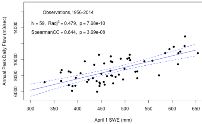
Figure 3: a) Regression of observed APF against basin-averaged 1 April SWE over the Fraser Basin, within the period of overlapping records, 1956-2014. The solid blue line is the least squares linear regression fit, while the dashed curves show the 95% confidence interval. Adjusted Pearson and Spearman rank correlation coefficients, along with their associated p -values, are indicated at upper left. b) Correlogram of all observed variables, averaged over the Fraser Basin over the common period of records for all variables, 1956-2006. Numerical values are Spearman rank correlation coefficients, and coloured squares indicate significant correlations at the p < 0.1 level.
