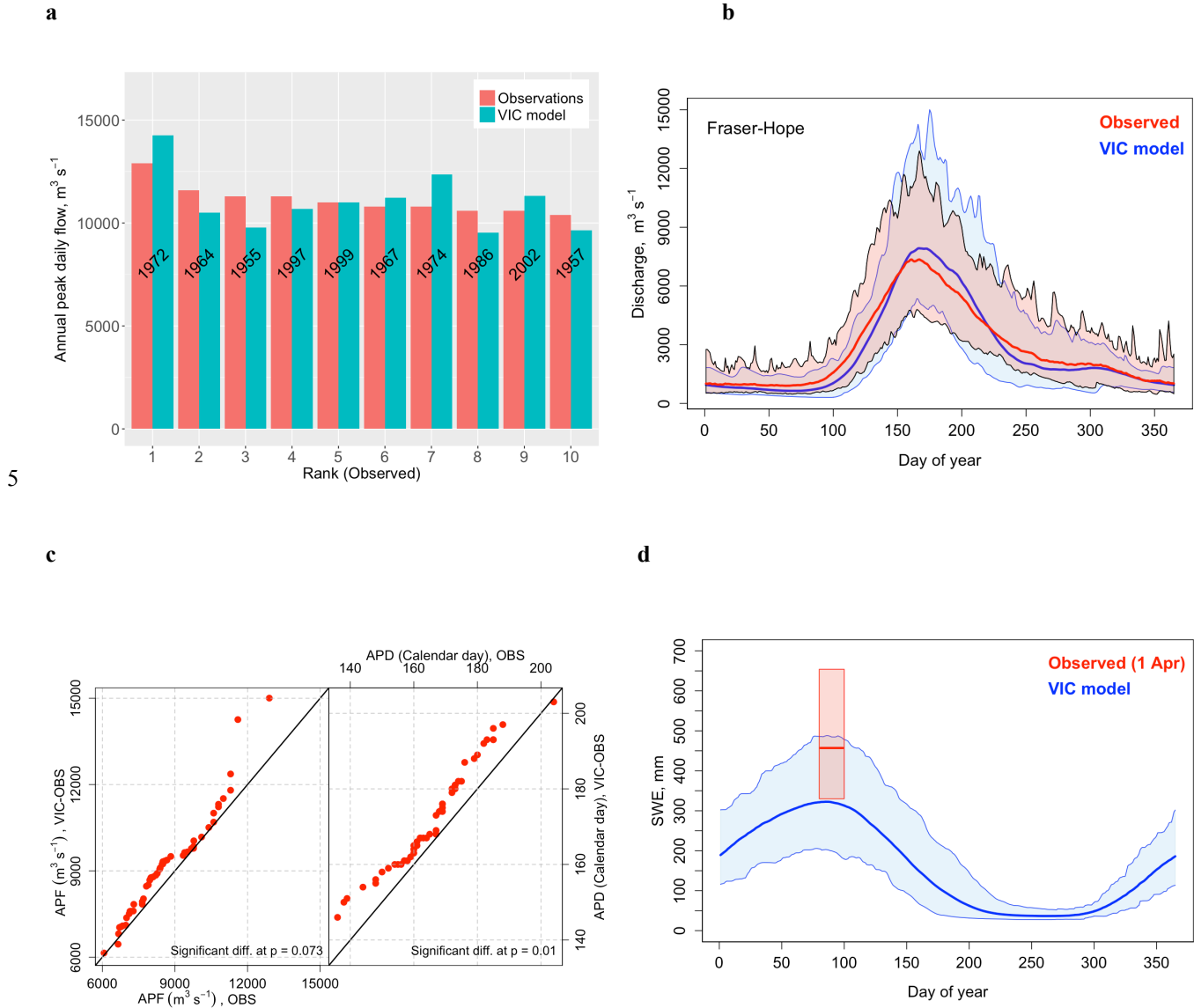
Figure 5: a) Annual peak daily streamflow (APF) magnitude in observations (red) and in the VIC simulation (blue) at Fraser-Hope, ranked by observed values over 1955-2004. b) Annual cycle of daily streamflow in observations (red) and VIC simulation (blue) over 1955-2004 at Fraser-Hope. c) Quantile plots of VIC-simulated versus observed APF and APD at Fraser-Hope. Differences between the respective distributions are assessed using a permutation test with 10^4 resamples; the resulting p -values are indicated in each sub-panel. d) 1 April observed SWE (red) compared with annual cycle of SWE from VIC, both averaged over the FRB for 1956-2006. Heavy curves in panels b and d show the multi-year mean while shaded areas show the interannual range.
