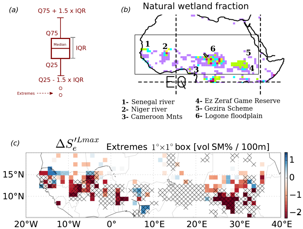
Figure 6. (a) - Schematic box plot illustrating the (Q_{25}-1.5 \times IQR, Q_{75}+1.5 \times IQR) range used to identify extreme \Delta(S_e^{Lmax}) values. Here, Q_{75} and Q_{25} are the third and first quartiles respectively, and the interquartile range (IQR) is the difference between them. (b) - Natural wetland fraction from Matthews and Fung (1987) on a 1^\circ \times 1^\circ grid (adopted from Fig.3 in Prigent et al. (2007)). Names of major wetland and river locations are marked with a number. (c) - Distribution of soil moisture gradient \Delta(S_e^{Lmax}) extremes in the corresponding event sample of a 1^\circ \times 1^\circ box (color). \Delta(S_e^{Lmax}) is considered to be an extreme if it lies outside the (Q_{25}-1.5 \times IQR, Q_{75}+1.5 \times IQR) range. Black crosses indicate boxes containing Lmin locations, in which climatology of daily soil moisture drying rates does not vary much with different absolute soil moisture values. These relationship is equivalent to low soil moisture variability in time, and is representative for a wet (flooded) locations. For detailed algorithm the reader is referred to the Appendix Figure A1. The distribution of identified potentially flooded locations is consistent with the natural wetland fraction (b).
