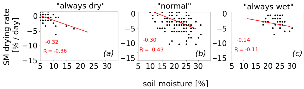
Figure A1. Examples of three possible relationships between climatology of soil moisture drying rate and absolute soil moisture in L_{min} locations. The red numbers indicate values of a slope and Spearman correlation respectively.
