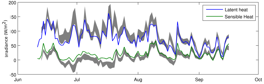
Figure 8. 5% and 95% uncertainty bounds for the heat fluxes, obtained from the GLUE global sensitivity method. The Nash-Sutcliffe performance was used to evaluate the model for the 2007 open-water season
