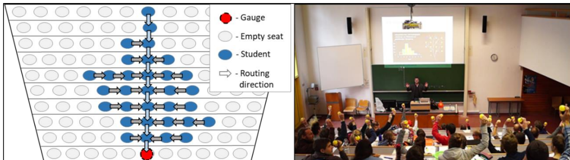
21 22 Figure 3: Catchment setup by 32 students in the original lecture theatre (right). The catchment/each student received an effective 23 precipitation of 1mm represented by a plastic ball. A sketch of student seating, flow routing and the gauge (left). Blue flow 24 arrows indicate the main stream channel within the catchment.
