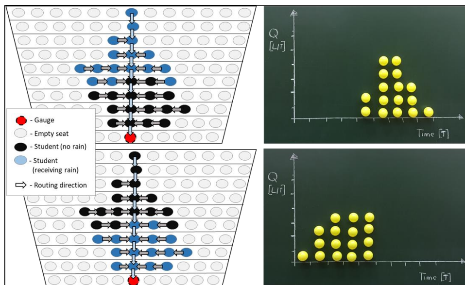
24 Figure 7: The effect of different spatial distributions of effective precipitation within the catchment on the resulting hydrograph. 25 The student seating, the spatial distribution of effective precipitation and the routing scheme are indicated on the left, the 26 hydrograph are illustrated on the right.
