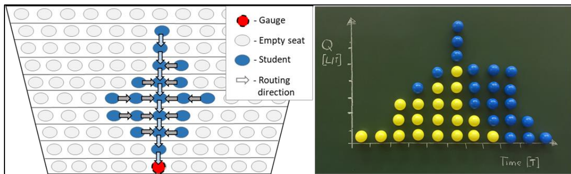
Figure 5: The superposition of two rainfall events, both producing an effective precipitation of 1mm. The first event is represented by yellow balls, the second event which is delayed by 4 time steps is represented by blue balls. The resulting hydrograph is shown on the right. The left figure illustrates the student seating and routing scheme applied in this experiment.
