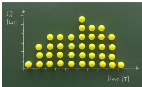
19 Figure 4: A lecture theatre catchment unit hydrograph resulting from 1mm effective precipitation (represented by a yellow 20 plastic ball) homogeneously spread over the catchment.
