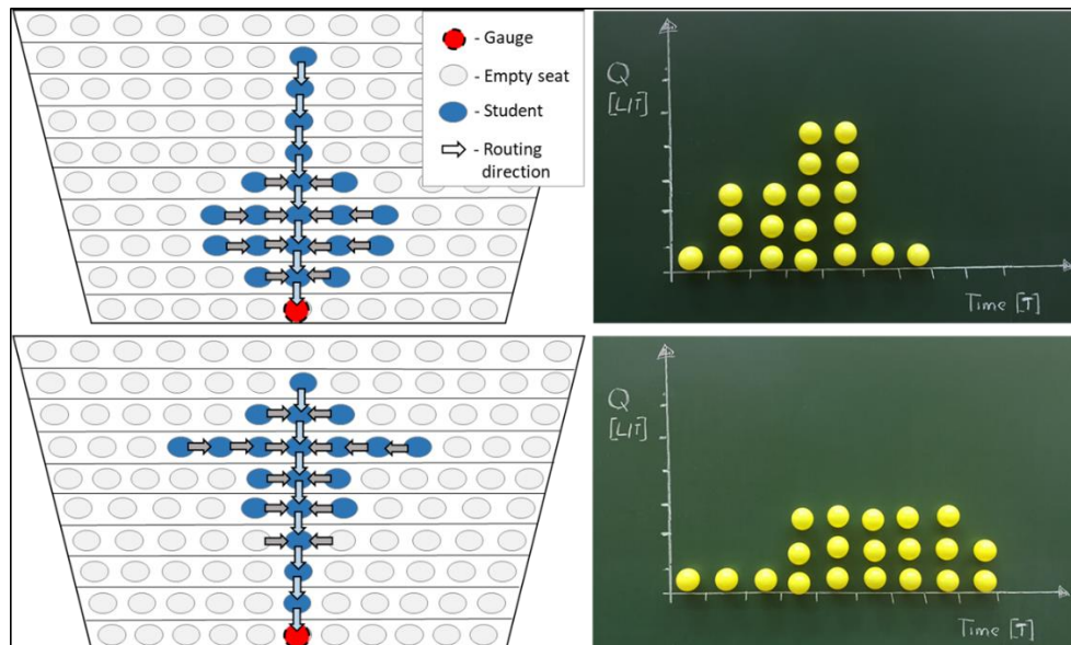
16 17 Figure 6: The effect of different catchment forms (same area/number of students, left) on the resulting hydrographs (right).
