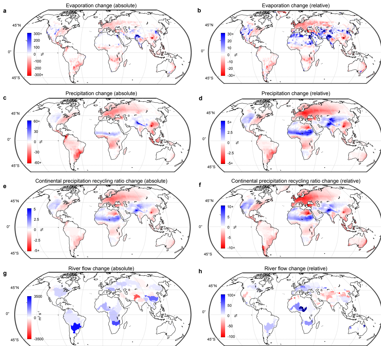
Figure 4. Land-use change induced changes in hydrological flows (current land-use - potential vegetation scenario): a, absolute change in evaporation, b, relative change in evaporation, c, absolute changes in precipitation, d, relative change in precipitation, e, absolute change in continental precipitation recycling ratio (i.e., precipitation with terrestrial origin divided by total precipitation P_{\text{tracked}}/P and converted to the unit of percent), f, relative change in continental precipitation recycling ratio, g, absolute change in river flow at outlet, and h, relative change in river flows at outlet.
